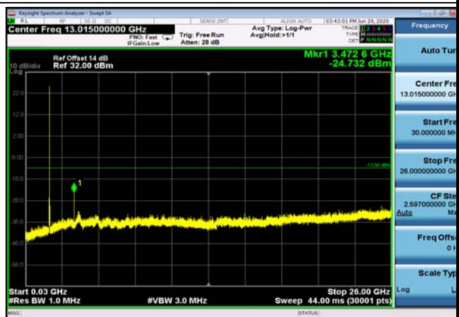
FDD04_HighRange_5MHz_30MHz~26GHz
