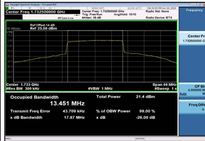
FDD04_MidRange_20_1732.5_QPSK
