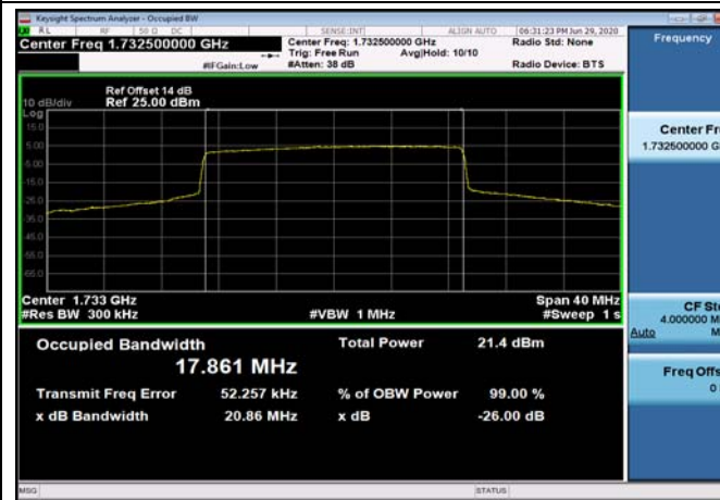
FDD04_MidRange_20_1732.5_QPSK
