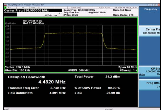
FDD05_MidRange_5_836.5_Q16
