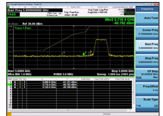
U-NII-3 ,Plot 1,Band Edge-802.11ac(20 MHz),5745MHz,Ant1
