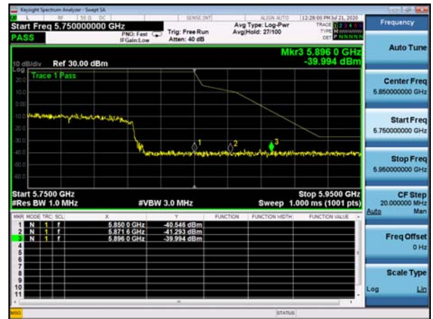
U-NII-3 ,Plot 1,Band Edge-802.11ac(80 MHz),5775MHz,Ant1
