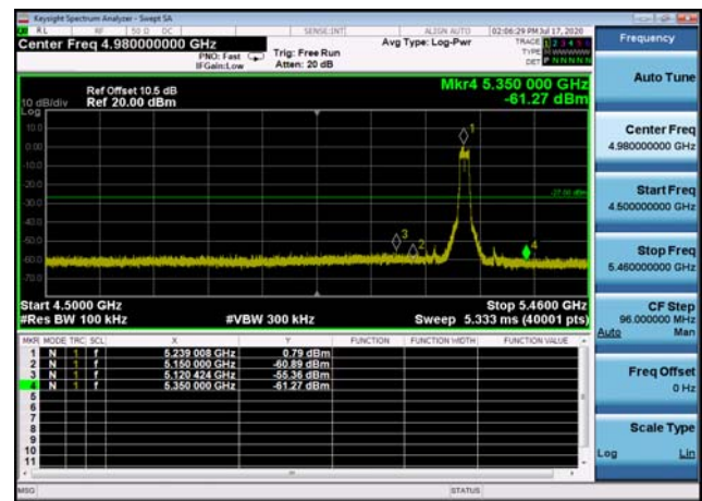
U-NII-1 Band Edge-802.11a(20MHz) ,5240MHz,Ant1
