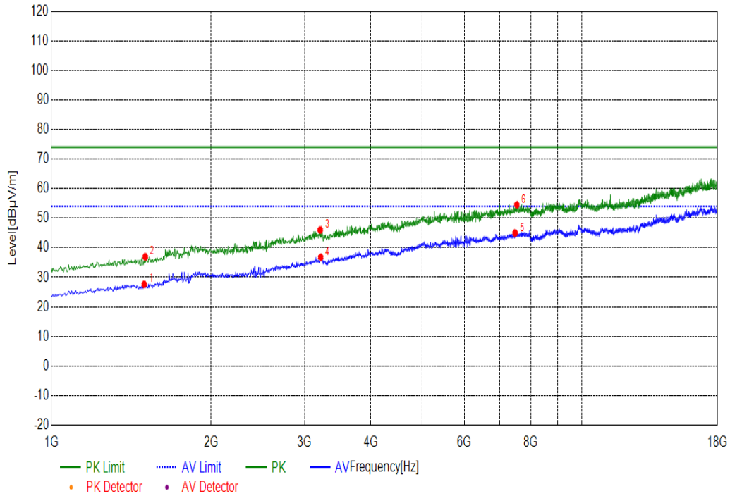
(Plot N: Test Antenna Vertical 1G – 18G)
