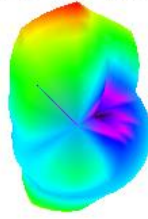
GSM850 251 TIS
