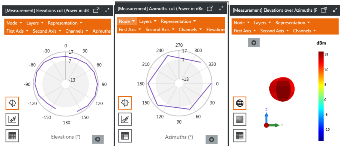
LTE-B17
