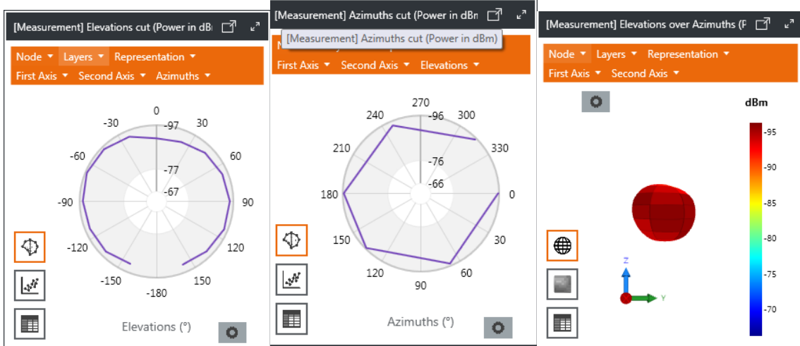
LTE-B17
