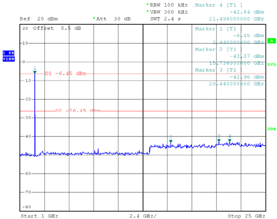
Channel = 39, 1GHz to 25GHz
