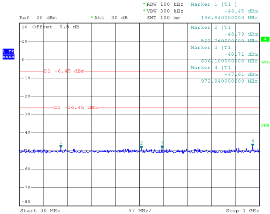
Channel = 39, 30MHz to 1GHz
