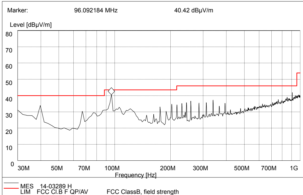
(Plot B: 30MHz to 1GHz, Antenna Horizontal)
