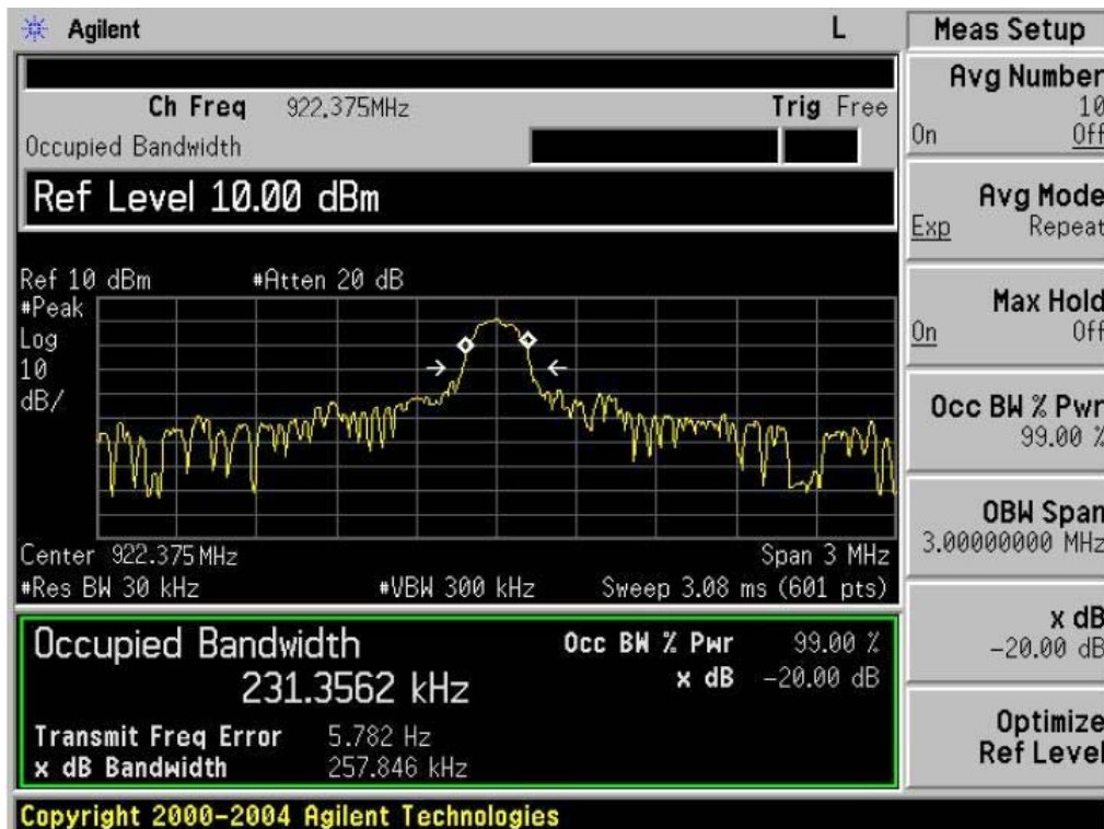
922.375MHz 20 dB Bandwidth
