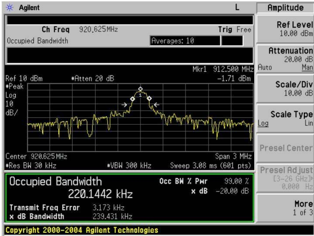
920.625MHz 20 dB Bandwidth
