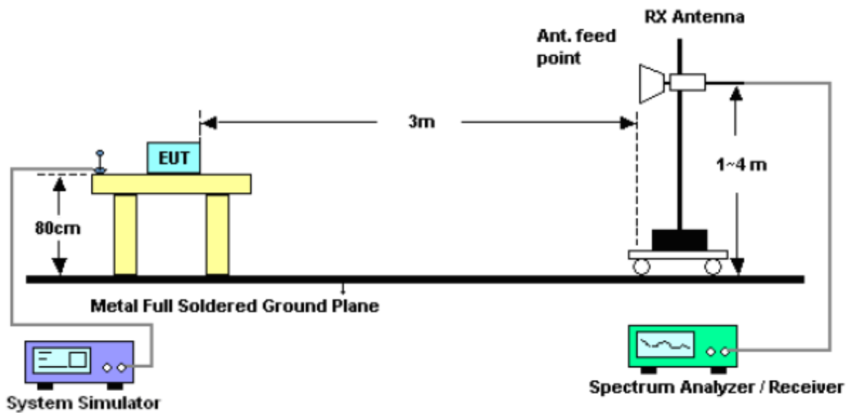
Radiated emissions above 1GHz
