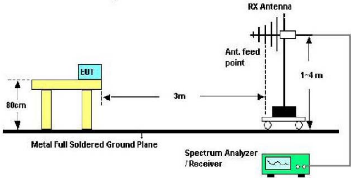
Radiated emissions from 30MHz to 1GHz
