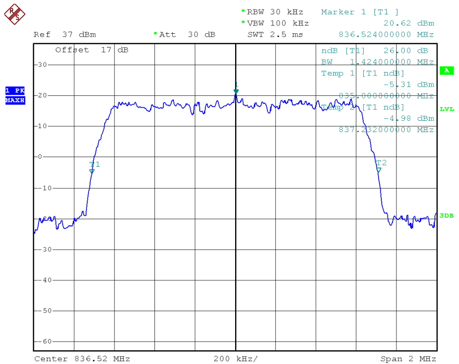
26dB Occupied Bandwidth Plot on Channel 384
