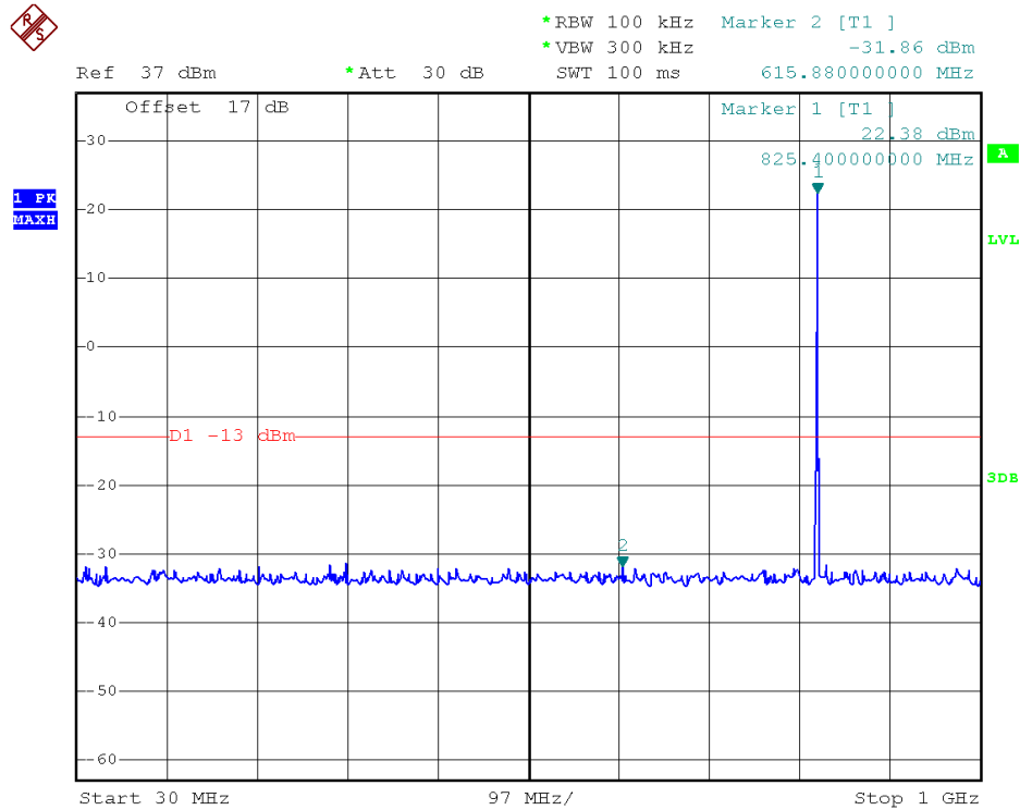
30MHz~1GHz
