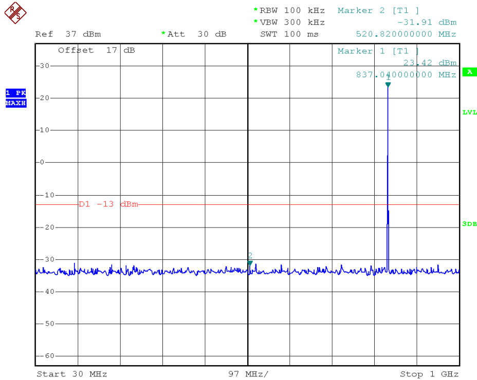
30MHz~1GHz
