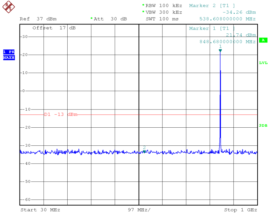
30MHz~1GHz
