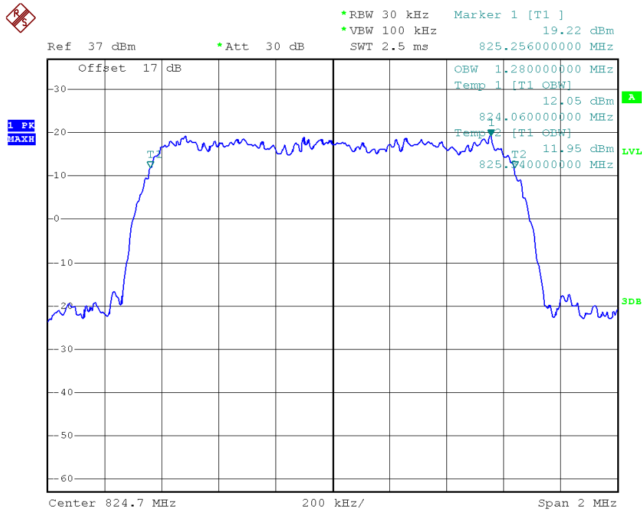
99% Occupied Bandwidth Plot on Channel 1013
