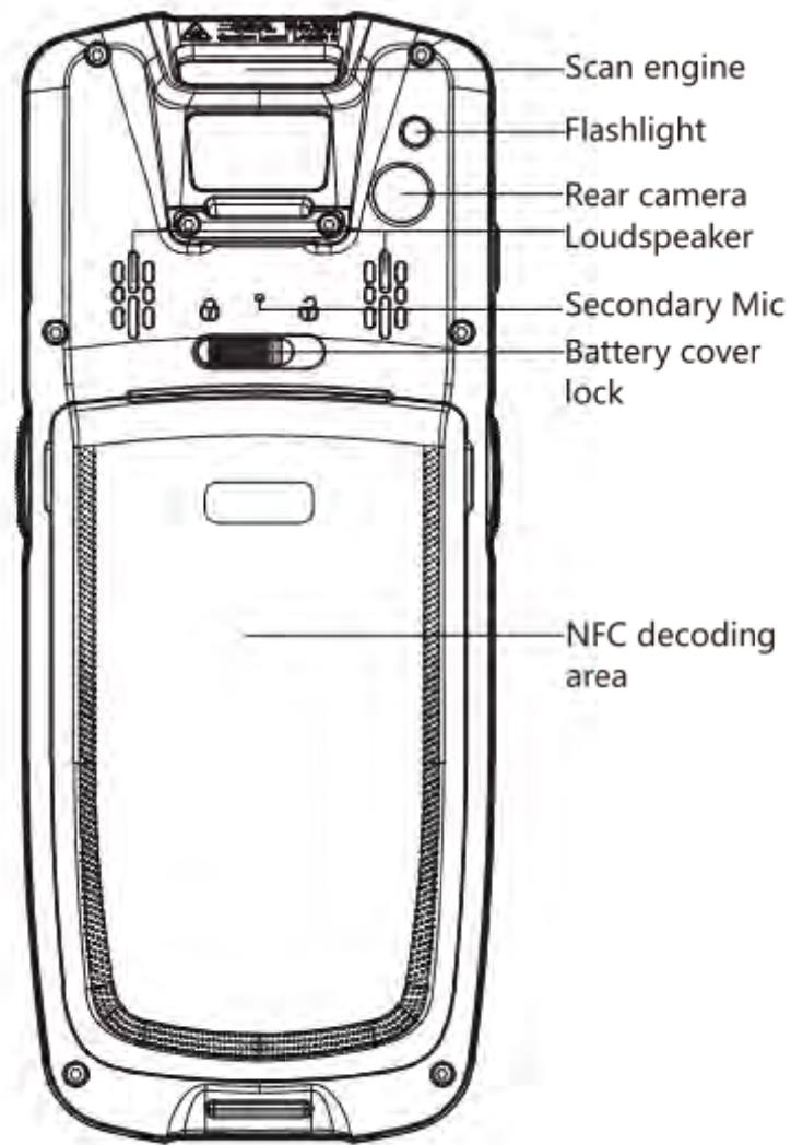
Fig 2. Back view
