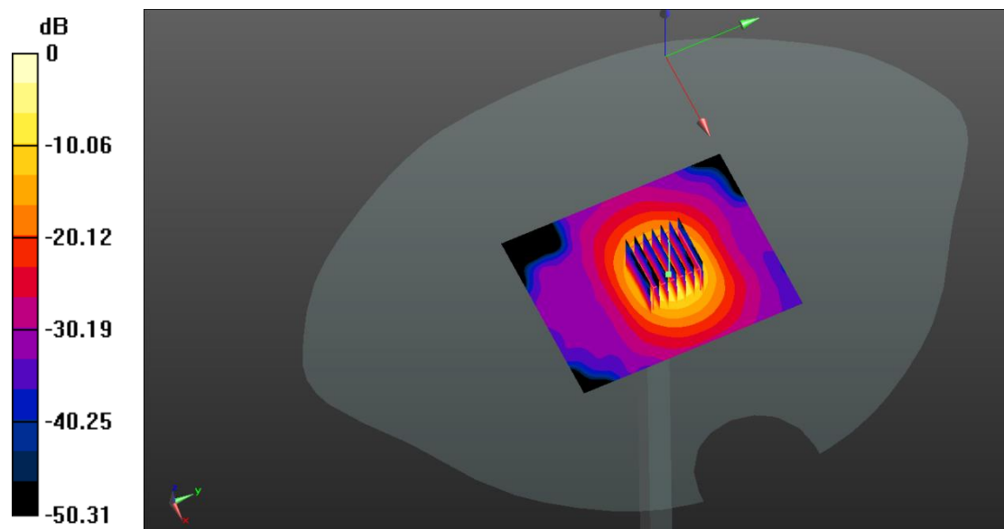
0 dB = 16.8 W/kg
