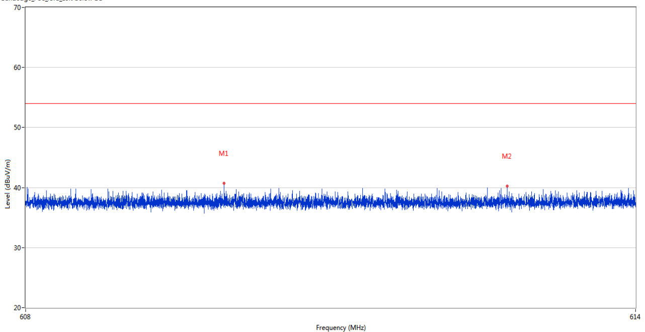
Bandedge_FCC_lora_Left below 1G
