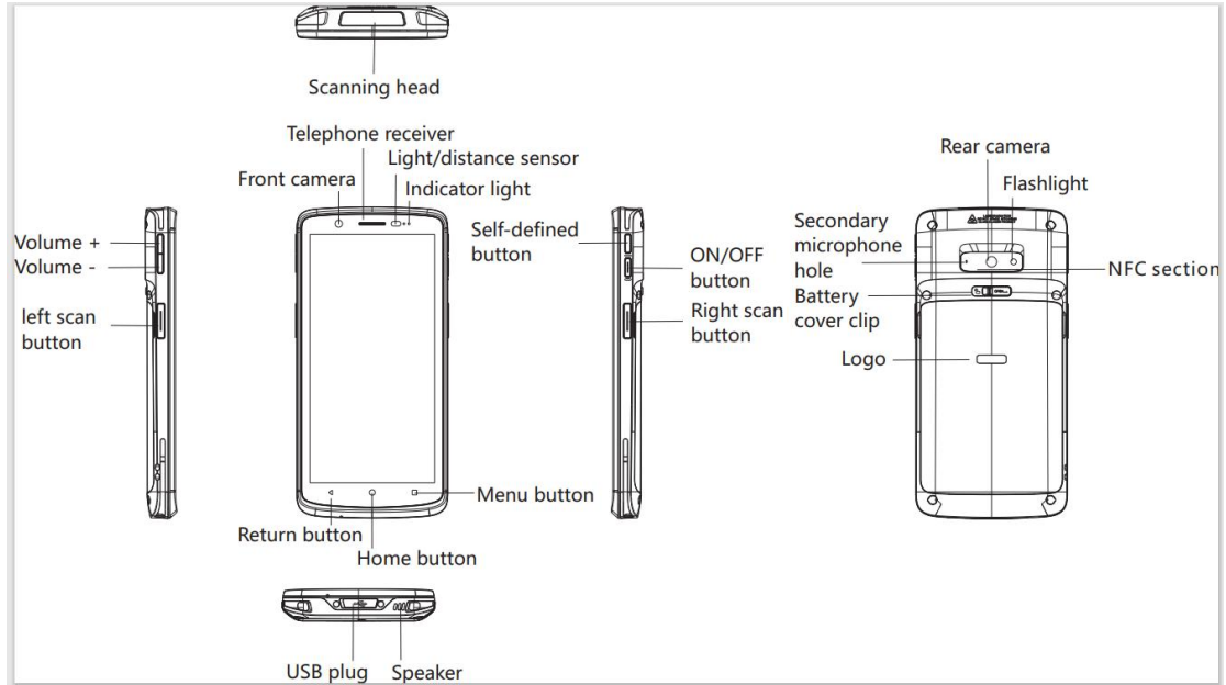
Figure 2-1 Six-sided View
