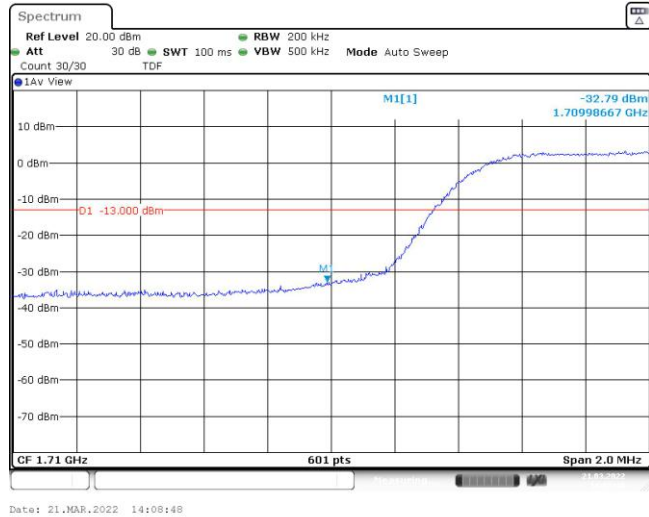
Band66-10MHz-QPSK-132622-50RB#0
