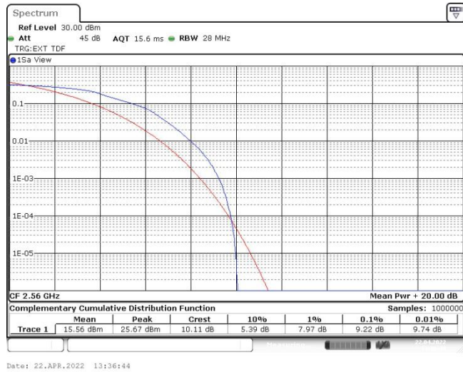
Band41-10MHz-16QAM-40620-50RB#0
