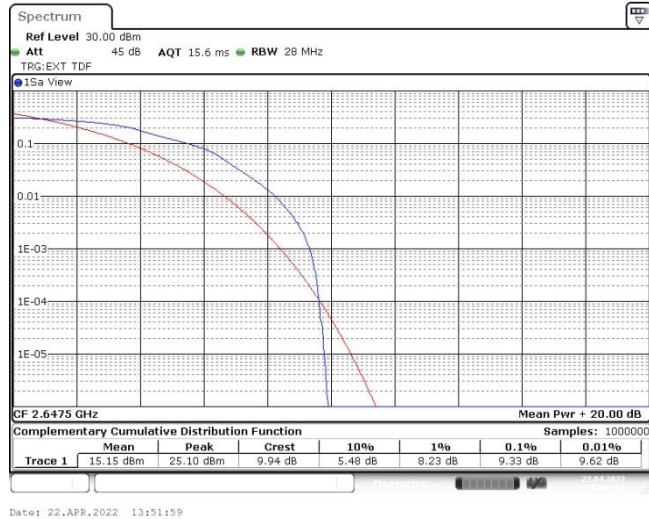
Band41-15MHz-16QAM-40315-75RB#0
