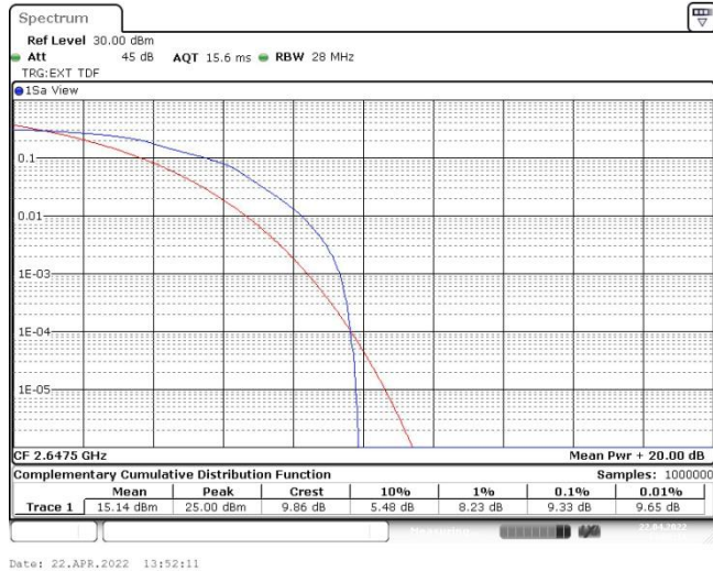
Band41-20MHz-QPSK-40340-100RB#0
