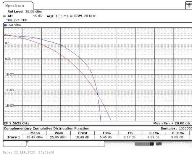
Band41-15MHz-16QAM-40620-75RB#0
