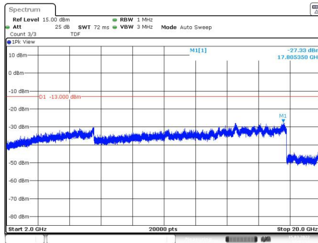
Band25-1.4MHz-QPSK-26047-1RB#0-Range3:2000~20000MHz
