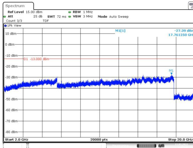
Band2-1.4MHz-QPSK-18607-6RB#0-Range3:2000~20000MHz
