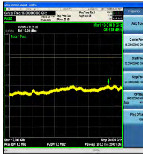
1-N2-15-20-H-1-DFT-PI2BPSK-Inner_1RB_Left-1@1 -12000-20000-Ant1--38.62--13-PASS
