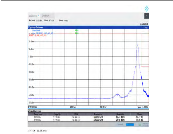
1-N2-15-15-H-2-DFT-PI2BPSK-Edge_1RB_Right-1@7 8-Ant1-seegraph-PASS-see graph
