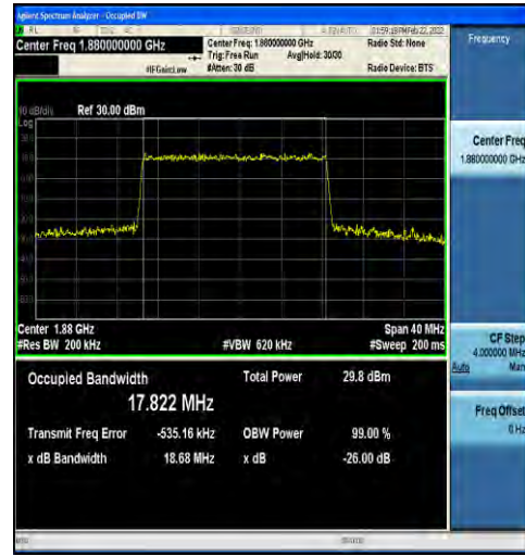
1-N2-15-20-M-4-DFT-64QAM-Outer_Full-100@0-Ant 1-17.822-18.68-≤20-PASS
