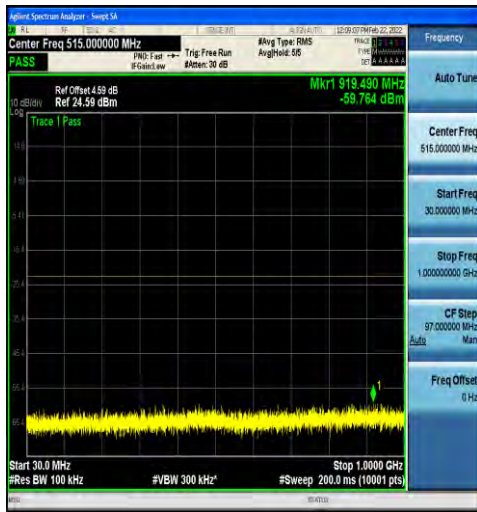
1-N2-15-20-M-1-DFT-PI2BPSK-Inner_1RB_Left-1@ 1-30-1000-Ant1--59.76--23-PASS
