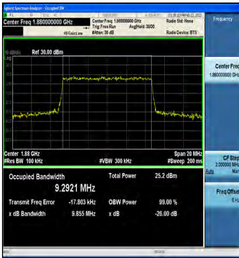
1-N2-15-10-M-9-CP-256QAM-Outer_Full-52@0-Ant 1-9.2921-9.855-≤10-PASS
