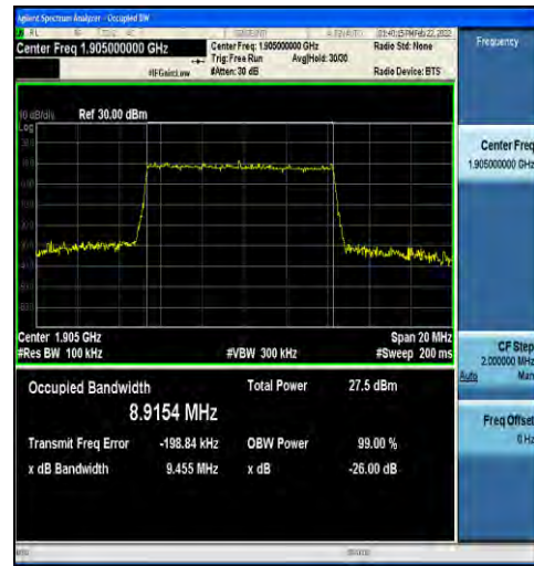
1-N2-15-10-H-5-DFT-256QAM-Outer_Full-50@0-Ant 1-8.9154-9.455-≤10-PASS
