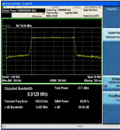
1-N2-15-10-M-5-DFT-256QAM-Outer_Full-50@0-Ant 1-8.9129-9.482-≤10-PASS
