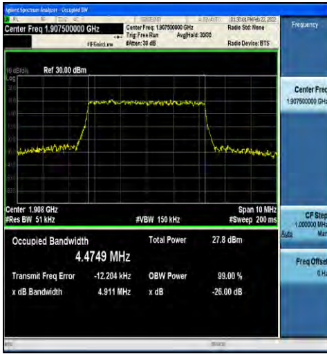
1-N2-15-5-H-7-CP-16QAM-Outer_Full-25@0-Ant1-4. 4749-4.911-≤5-PASS
