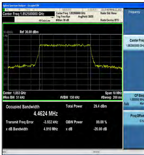
1-N2-15-5-L-3-DFT-16QAM-Outer_Full-25@0-Ant1- 4.4624-4.910-≤5-PASS
