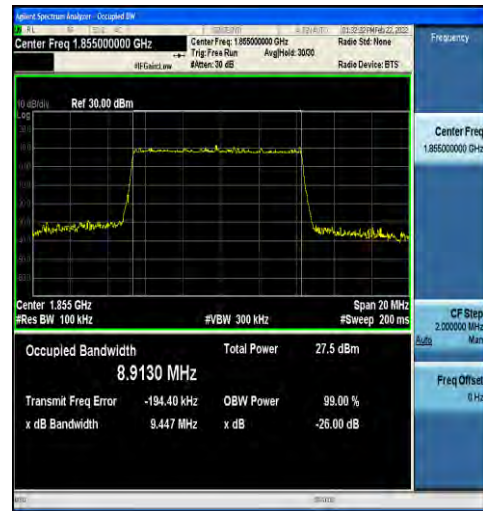
1-N2-15-10-L-5-DFT-256QAM-Outer_Full-50@0-Ant 1-8.9130-9.447-≤10-PASS
