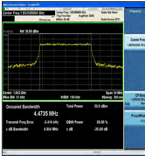
1-N2-15-5-L-1-DFT-QPSK-Outer_Full-25@0-Ant1-4. 4735-4.854-≤5-PASS
