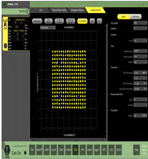
1-N2-15-20-M-9-CP-256QAM-Outer_Full-106@0-Ant 1-see graph-PASS
