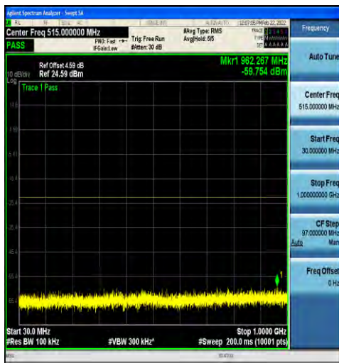
1-N2-15-20-L-1-DFT-PI2BPSK-Inner_1RB_Left-1@1 -30-1000-Ant1--59.75--23-PASS
