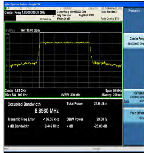
1-N2-15-10-M-2-DFT-PI2BPSK-Outer_Full-50@0-An t1-8.8960-9.442-≤10-PASS
