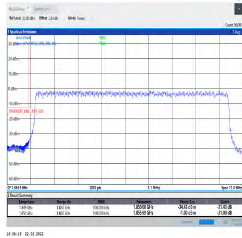
1-N2-15-10-L-3-DFT-PI2BPSK-Outer_Full-50@0-Ant1-seegraph-PASS-see graph
