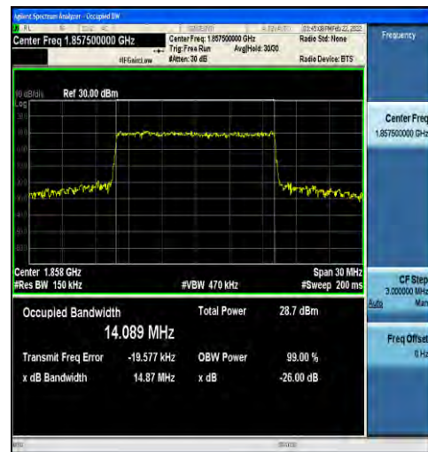
1-N2-15-15-L-6-CP-QPSK-Outer_Full-79@0-Ant1-14 .089-14.87≤15-PASS
