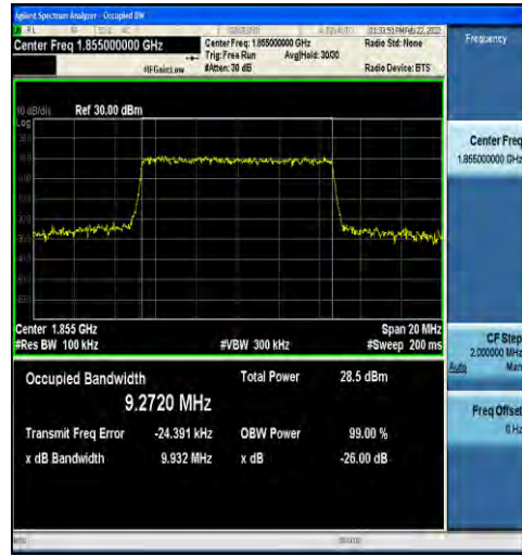
1-N2-15-10-L-7-CP-16QAM-Outer_Full-52@0-Ant1-9 .2720-9.932-≤10-PASS
