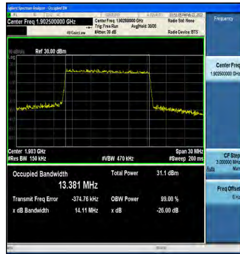
1-N2-15-15-H-2-DFT-PI2BPSK-Outer_Full-75@0-Ant 1-13.381-14.11-≤15-PASS
