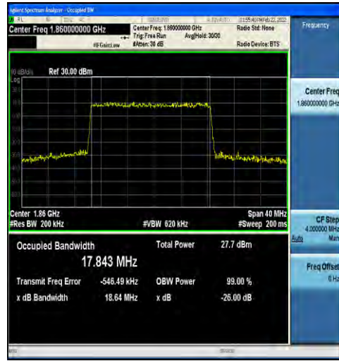
1-N2-15-20-L-5-DFT-256QAM-Outer_Full-100@0-An t1-17.843-18.64-≤20-PASS
