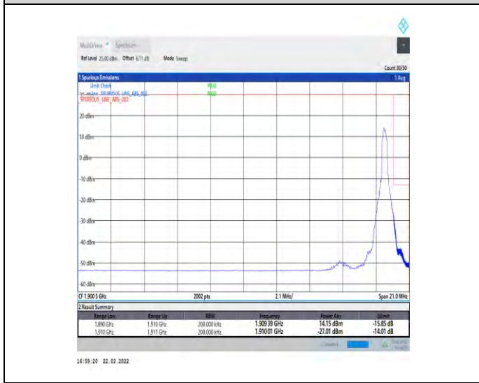
1-N2-15-20-H-5-CP-QPSK-Edge_1RB_Right-1@105-Ant1-seegraph-PASS-see graph
