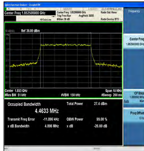
1-N2-15-5-L-8-CP-64QAM-Outer_Full-25@0-Ant1-4. 4633-4.896-≤5-PASS
