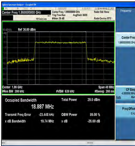
1-N2-15-20-L-6-CP-QPSK-Outer_Full-106@0-Ant1 18.887-19.74-≤20-PASS
