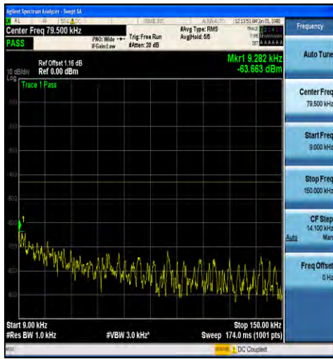
1-N2-15-20-H-1-DFT-PI2BPSK-Inner_1RB_Left-1@ 1-0.009-0.15-Ant1--63.66--43-PASS
