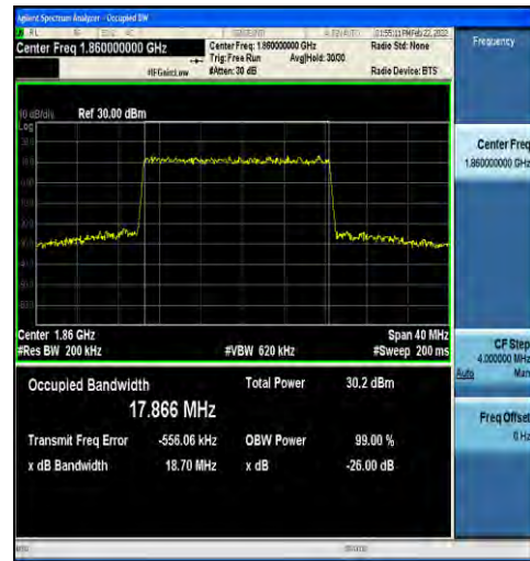
1-N2-15-20-L-3-DFT-16QAM-Outer_Full-100@0-Ant 1-17.866-18.70-≤20-PASS
