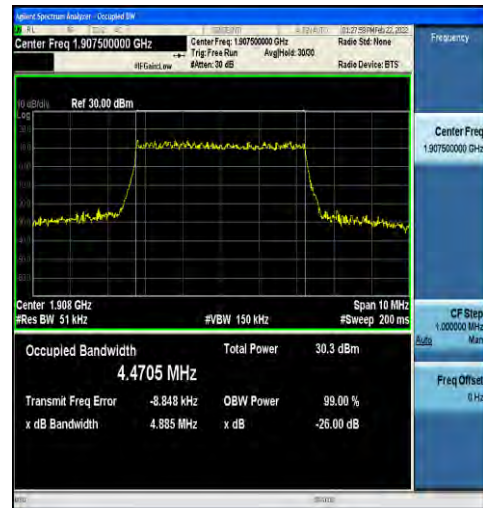
1-N2-15-5-H-2-DFT-PI2BPSK-Outer_Full-25@0-Ant1 -4.4705-4.885-≤5-PASS
