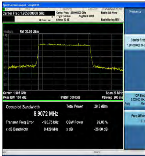
1-N2-15-10-H-4-DFT-64QAM-Outer_Full-50@0-Ant1 -8.9072-9.429-≤10-PASS
