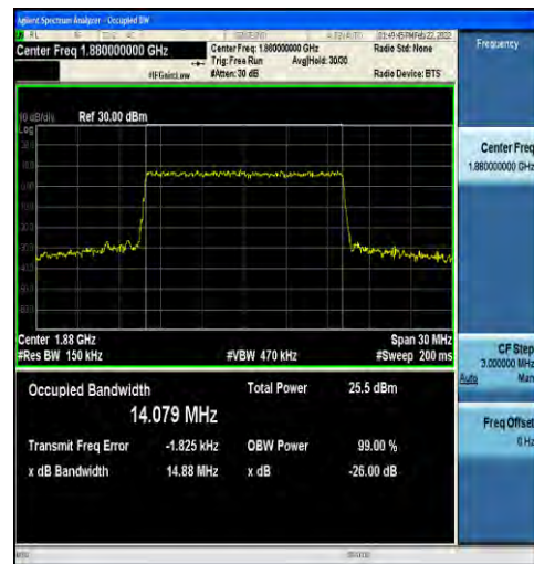
1-N2-15-15-M-9-CP-256QAM-Outer_Full-79@0-Ant1-1 -14.079-14.88-≤15-PASS
