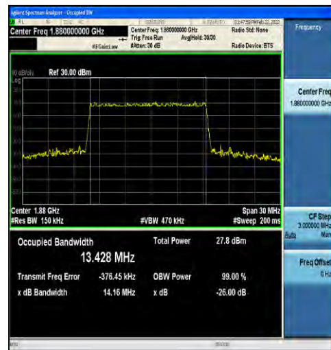
1-N2-15-15-M-5-DFT-256QAM-Outer_Full-75@0-Ant 1-13.428-14.16-≤15-PASS
