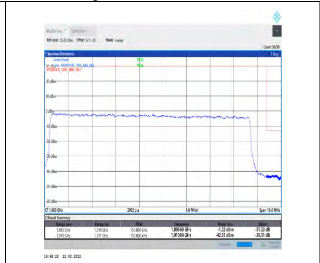
1-N2-15-15-H-3-DFT-PI2BPSK-Outer_Full-75@0- Ant1-seegraph-PASS-see graph
