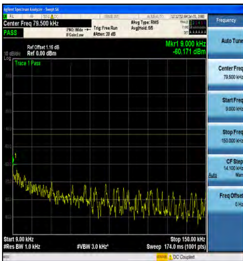
1-N2-15-20-M-1-DFT-PI2BPSK-Inner_1RB_Left-1@1 1-0.009-0.15-Ant1--60.17--43-PASS
