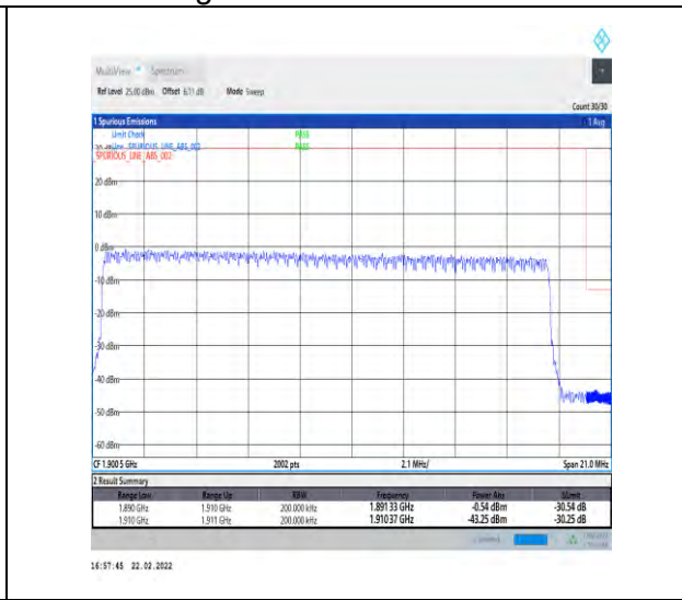
1-N2-15-20-H-3-DFT-PI2BPSK-Outer_Full-100@0-Ant1-seegraph-PASS-see graph
