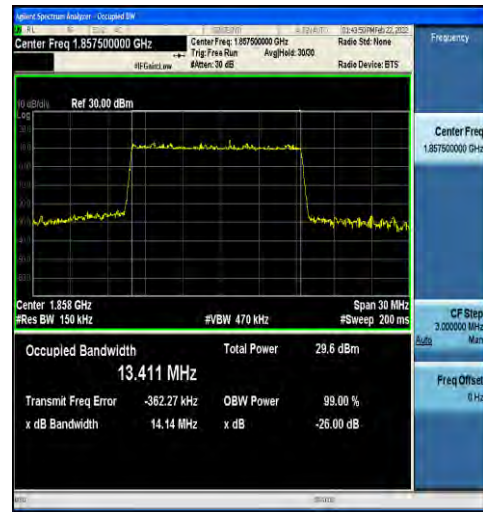
1-N2-15-15-L-4-DFT-64QAM-Outer_Full-75@0-Ant1- 13.411-14.14≤15-PASS
