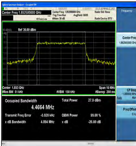
1-N2-15-5-L-7-CP-16QAM-Outer_Full-25@0-Ant1-4. 4664-4.894-≤5-PASS
