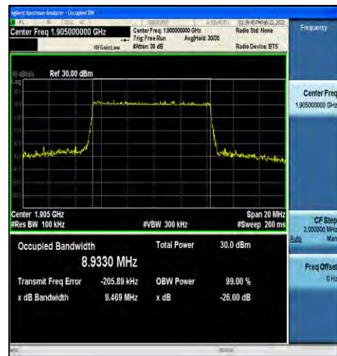
1-N2-15-10-H-3-DFT-16QAM-Outer_Full-50@0-Ant1 -8.9330-9.469-≤10-PASS
