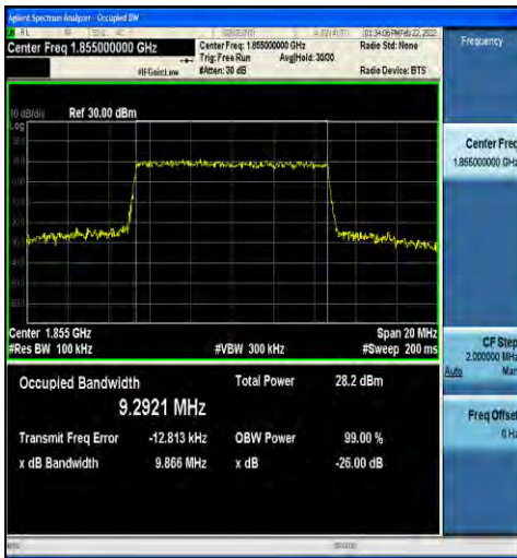
1-N2-15-10-L-8-CP-64QAM-Outer_Full-52@0-Ant1-9. 9.2921-9.866-≤10-PASS
