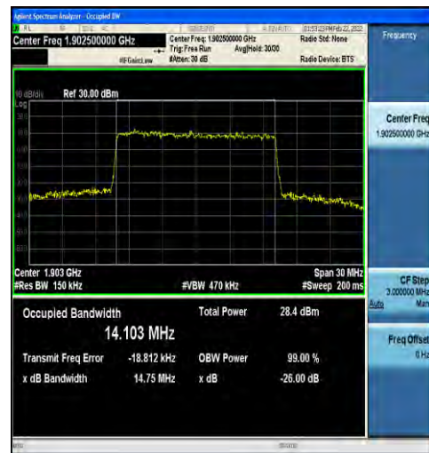
1-N2-15-15-H-8-CP-64QAM-Outer_Full-79@0-Ant1- 14.103-14.75-≤15-PASS
