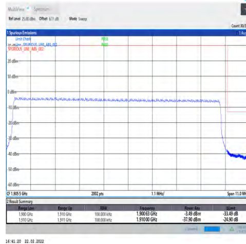
1-N2-15-10-H-6-CP-QPSK-Outer_Full-52@0-Ant1 -seegraph-PASS-see graph
