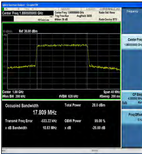
1-N2-15-20-M-5-DFT-256QAM-Outer_Full-100@0-A nt1-17.809-18.63-≤20-PASS
