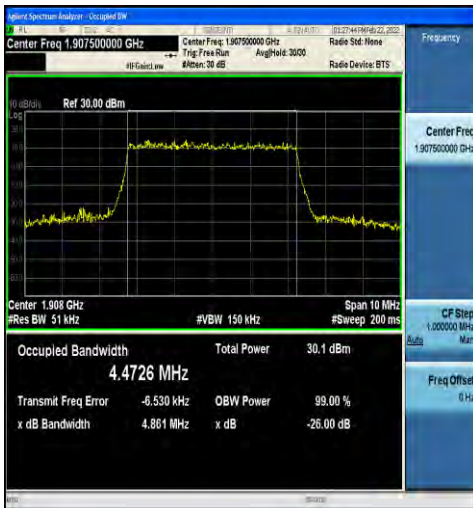
1-N2-15-5-H-1-DFT-QPSK-Outer_Full-25@0-Ant1-4. 4726-4.861-≤5-PASS
