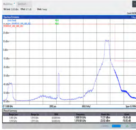
1-N2-15-5-H-2-DFT-PI2BPSK-Edge_1RB_Right-1@24-Ant1-seegraph-PASS-see graph
