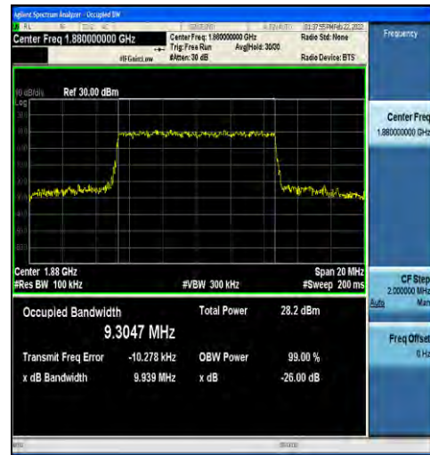
1-N2-15-10-M-8-CP-64QAM-Outer_Full-52@0-Ant1- 9.3047-9.939-≤10-PASS
