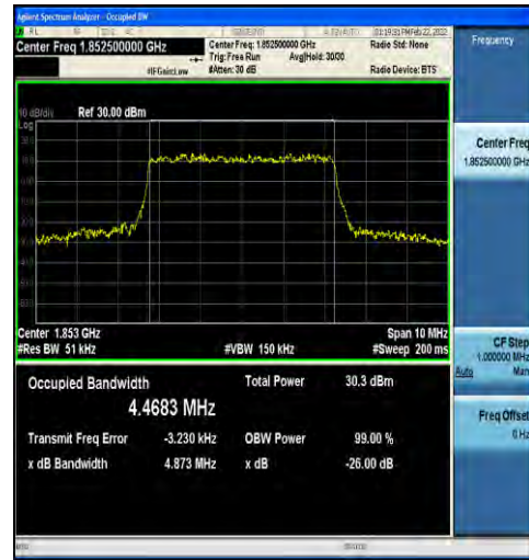
1-N2-15-5-L-2-DFT-P12BPSK-Outer_Full-25@0-Ant1 -4.4683-4.873-≤5-PASS
