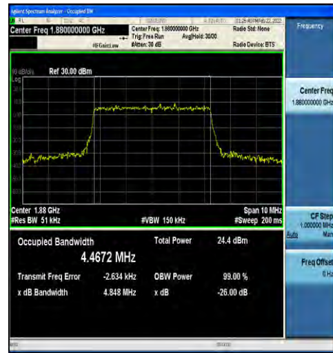
1-N2-15-5-M-9-CP-256QAM-Outer_Full-25@0-Ant1-4 4.4672-4.848-≤5-PASS
