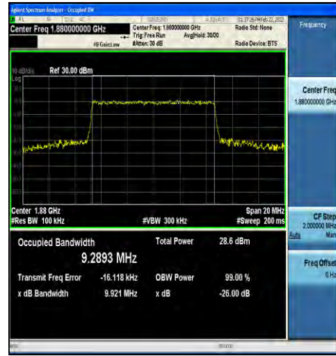
1-N2-15-10-M-6-CP-QPSK-Outer_Full-52@0-Ant1-9. 2893-9.921-≤10-PASS
