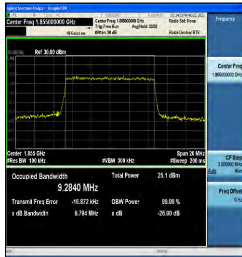
1-N2-15-10-L-9-CP-256QAM-Outer_Full-52@0-Ant1-9. 9.2840-9.794-≤10-PASS
