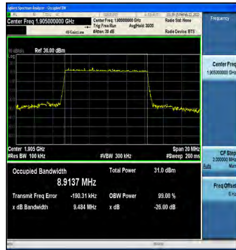
1-N2-15-10-H-1-DFT-QPSK-Outer_Full-50@0-Ant1 8.9137-9.484-≤10-PASS
