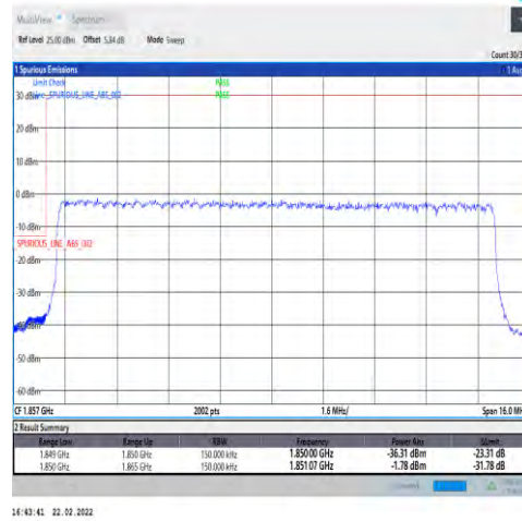
1-N2-15-15-L-3-DFT-PI2BPSK-Outer_Full-75@0-Ant1-seegraph-PASS-see graph
