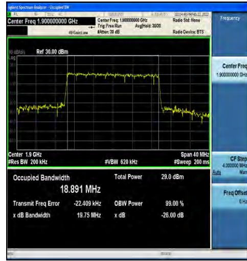
1-N2-15-20-H-7-CP-16QAM-Outer_Full-106@0-Ant1 -18.891-19.75-≤20-PASS
