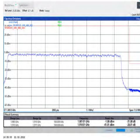
1-N2-15-10-H-3-DFT-PI2BPSK-Outer_Full-50@0-Ant1-seegraph-PASS-see graph
