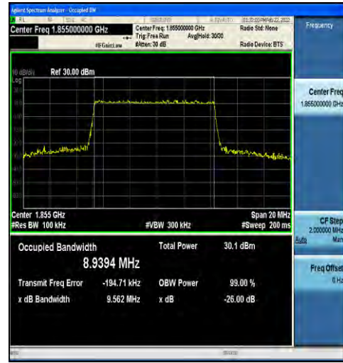
1-N2-15-10-L-3-DFT-16QAM-Outer_Full-50@0-Ant1 8.9394-9.562-≤10-PASS
