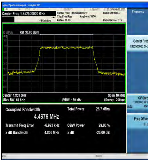
1-N2-15-5-L-5-DFT-256QAM-Outer_Full-25@0-Ant1 -4.4676-4.856-≤5-PASS
