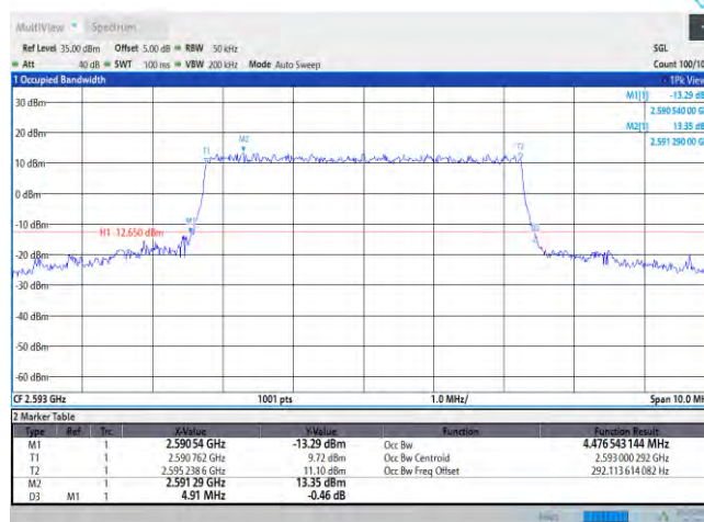
Band41-5MHz-QPSK-40620-25RB#0
