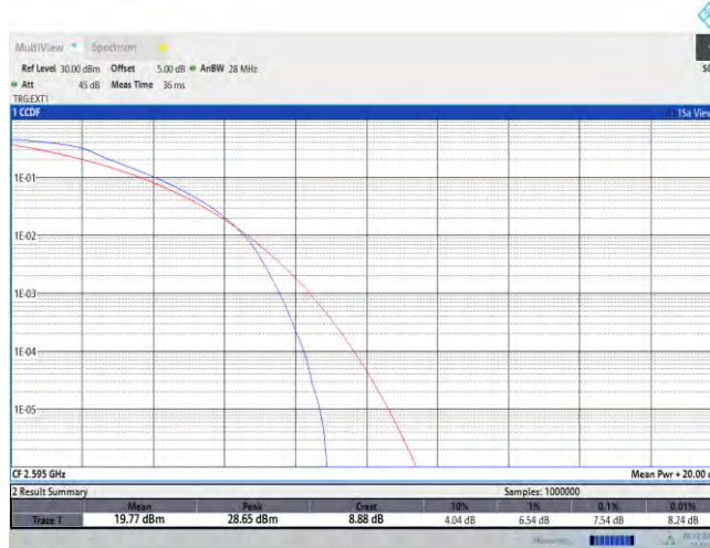
Band38-20MHz-QPSK-38000-100RB#0
