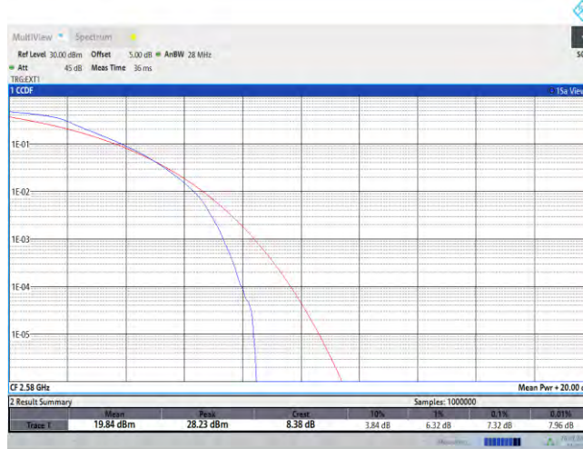
Band38-20MHz-QPSK-37850-100RB#0
