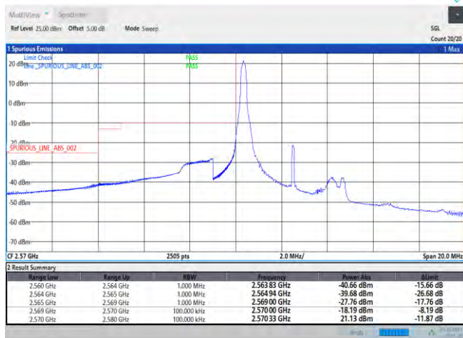
Band38-5MHz-QPSK-37775-25RB#0
