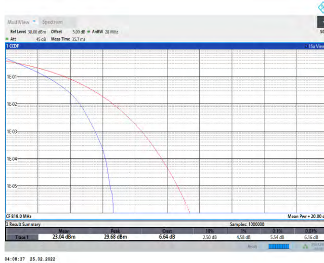
Band26-10MHz-16QAM-26740-50RB#0
