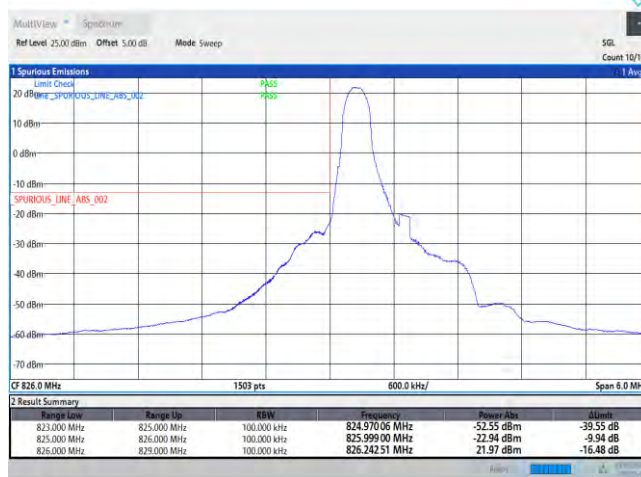
Band5-1.4MHz-QPSK-20427-6RB#0
