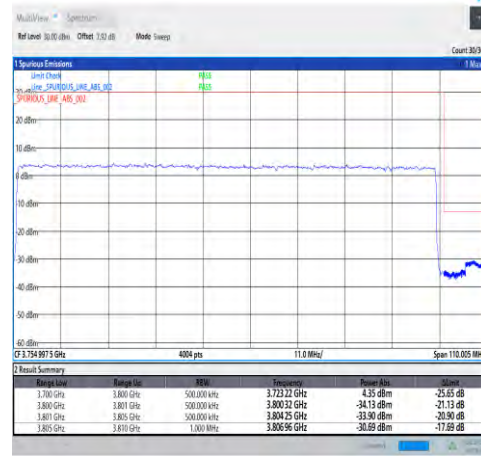
1-N78-3700-3800-30-100-H-3-DFT-PI2BPSK-Outer_Full-270@0-Ant1-PASS-see graph
