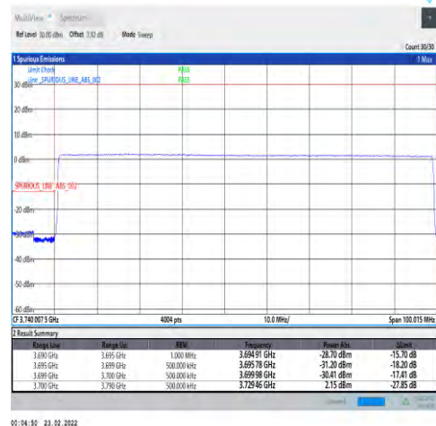
1-N78-3700-3800-30-90-L-6-CP-QPSK-Outer_Full -245@0-Ant1-PASS-see graph
