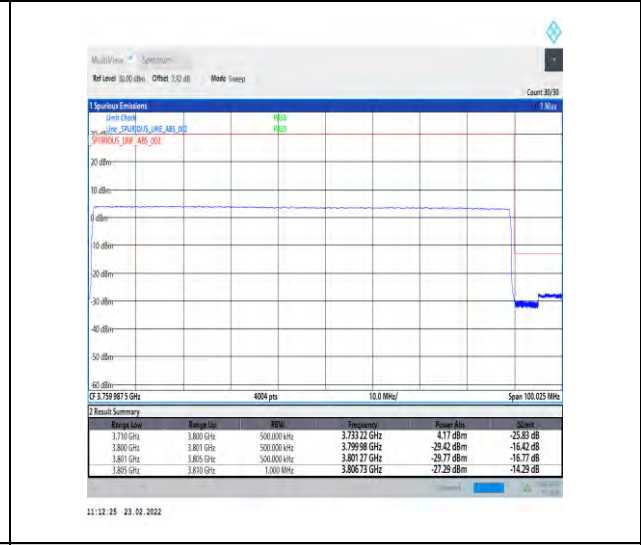
1-N78-3700-3800-30-90-H-6-CP-QPSK-Outer_Full-245@0-Ant1-PASS-see graph
