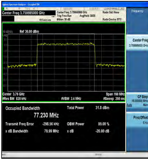
1-N78-3700-3800-30-80-H-3-DFT-16QAM-Outer_Ful I-216@0-Ant1-77.230-79.99-≤80-PASS
