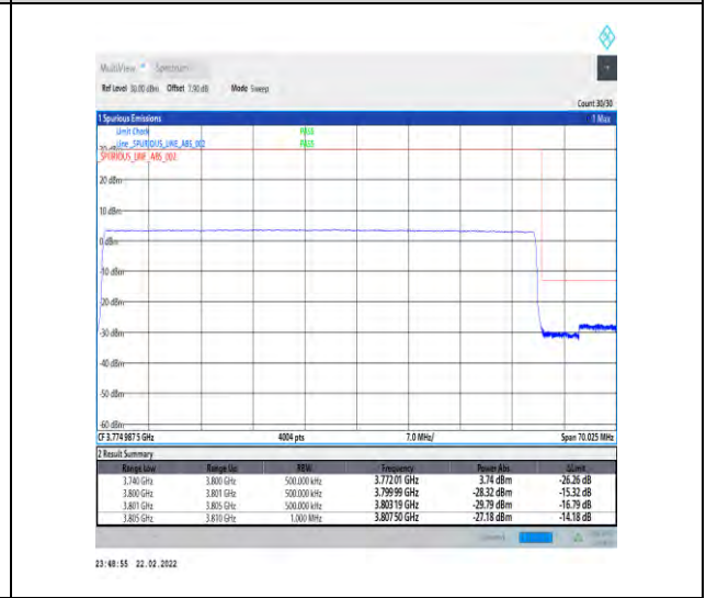
1-N78-3700-3800-30-60-H-6-CP-QPSK-Outer_Full-162@0-Ant1-PASS-see graph
