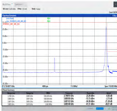
1-N78-3700-3800-30-100-H-2-DFT-PI2BPSK-Edge_1R_B_Right-1@272-Ant1-PASS-see graph
