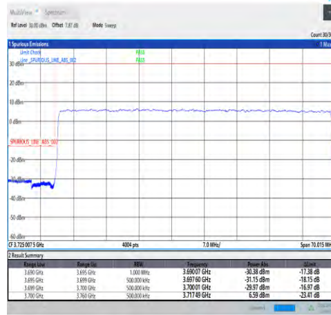
1-N78-3700-3800-30-60-L-3-DFT-PI2BPSK-Outer_Full-162@0-Ant1-PASS-see graph
