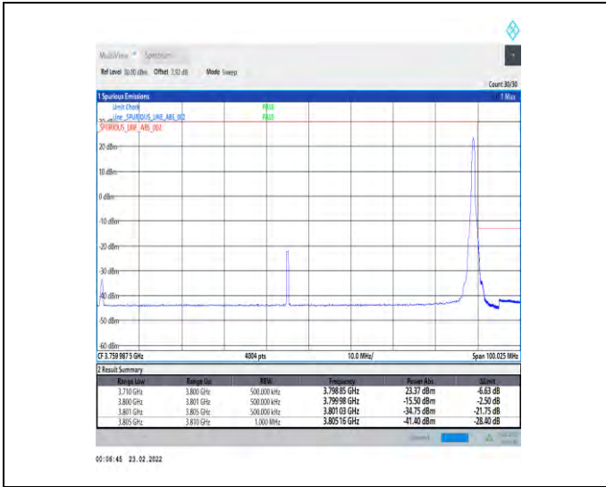
1-N78-3700-3800-30-90-H-2-DFT-PI2BPSK-Edge_1R_B_Right-1@244-Ant1-PASS-see graph
