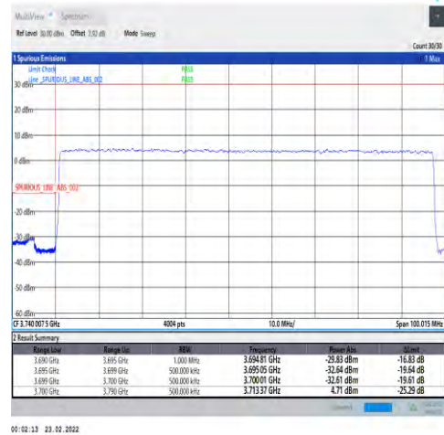
1-N78-3700-3800-30-90-L-3-DFT-PI2BPSK-Outer_Full-240@0-Ant1-PASS-see graph
