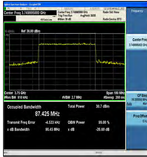
1-N78-3700-3800-30-90-M-6-CP-QPSK-Outer_Full-245@0-Ant1-87.425-90.45-≤90-PASS
