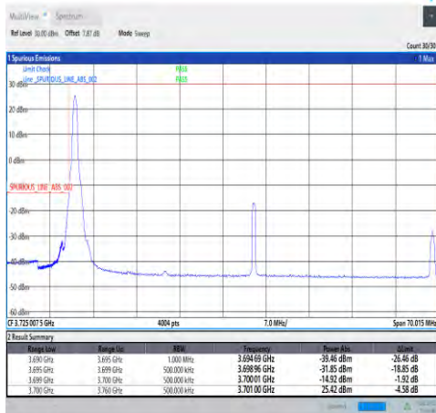
1-N78-3700-3800-30-60-L-4-CP-QPSK-Edge_1RB_Lef t-1@0-Ant1-PASS-see graph
