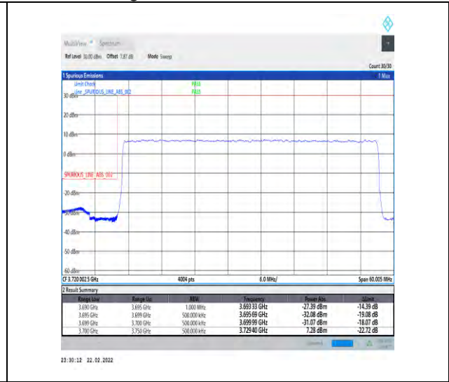
1-N78-3700-3800-30-50-L-3-DFT-PI2BPSK-Outer_Full-128@0-Ant1-PASS-see graph
