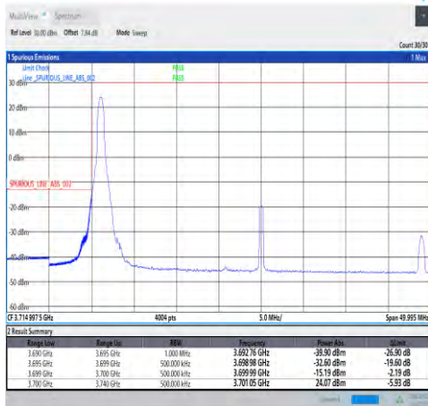
1-N78-3700-3800-30-40-L-4-CP-QPSK-Edge_1RB_Lef t-1@0-Ant1-PASS-see graph
