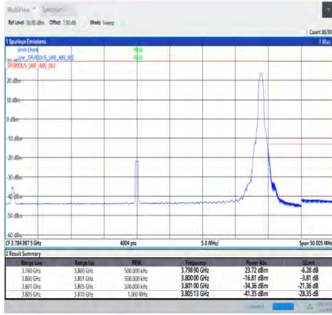
1-N78-3700-3800-30-40-H-2-DFT-PI2BPSK-Edge_1R_B_Right-1@105-Ant1-PASS-see graph
