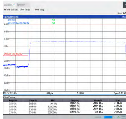
1-N78-3700-3800-30-40-L-6-CP-QPSK-Outer_Full -106@0-Ant1-PASS-see graph
