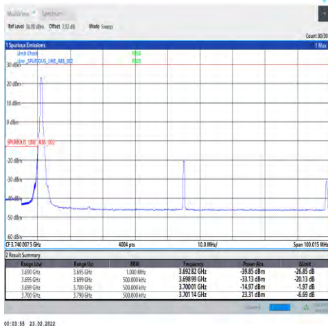
1-N78-3700-3800-30-90-L-4-CP-QPSK-Edge_1RB_Lef t-1@0-Ant1-PASS-see graph
