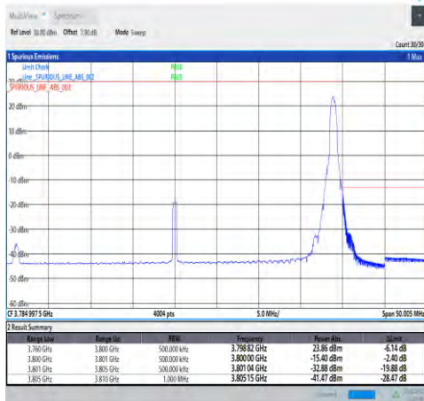
1-N78-3700-3800-30-40-H-5-CP-QPSK-Edge_1RB_Right-1@105-Ant1-PASS-see graph
