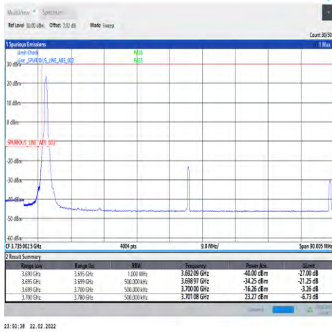
1-N78-3700-3800-30-80-L-1-DFT-PI2BPSK-Edge_1RB_Left-1@0-Ant1-PASS-see graph
