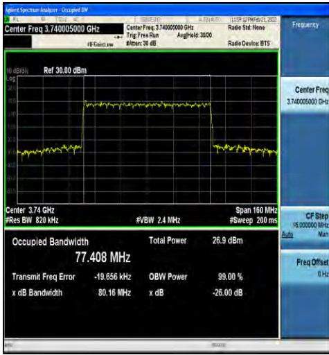
1-N78-3700-3800-30-80-L-9-CP-256QAM-Outer_Full -217@0-Ant1-77.408-80.16-<80-PASS
