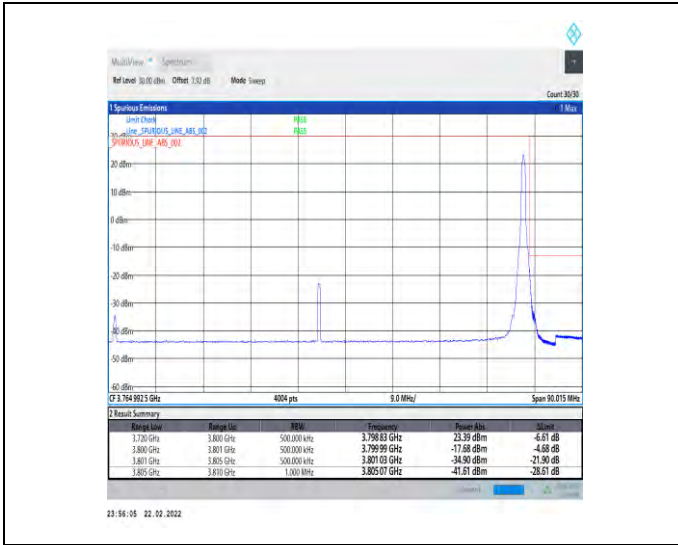
1-N78-3700-3800-30-80-H-2-DFT-PI2BPSK-Edge_1R_B_Right-1@216-Ant1-PASS-see graph
