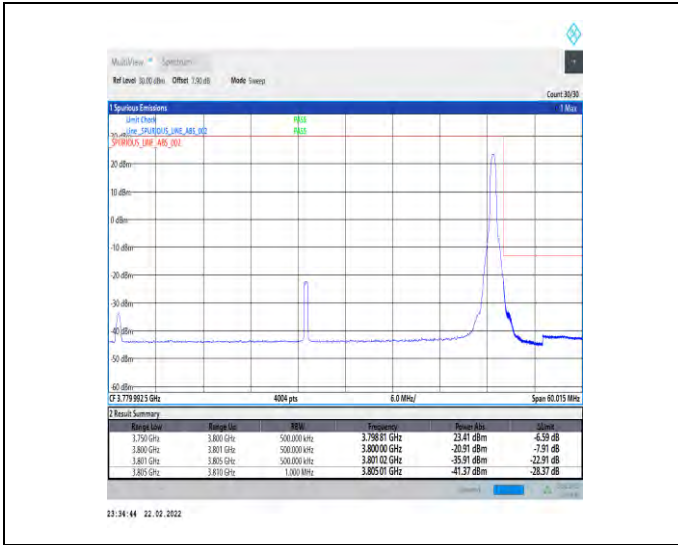
1-N78-3700-3800-30-50-H-2-DFT-PI2BPSK-Edge_1R_B_Right-1@132-Ant1-PASS-see graph
