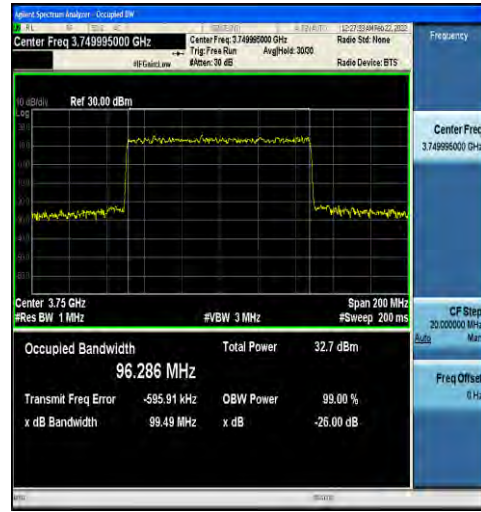
1-N78-3700-3800-30-100-H-2-DFT-PI2BPSK-Outer_Full -270@0-Ant1-96.286-99.49-≤100-PASS
