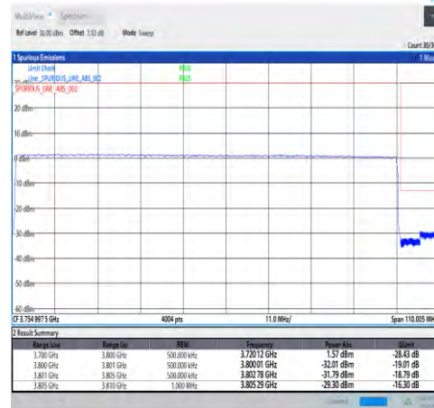
1-N78-3700-3800-30-100-H-6-CP-QPSK-Outer_Full-273@0-Ant1-PASS-see graph
