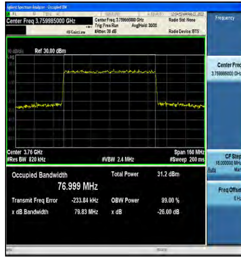
1-N78-3700-3800-30-80-H-4-DFT-64QAM-Outer_Ful I-216@0-Ant1-76.999-79.83-≤80-PASS
