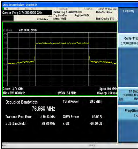
1-N78-3700-3800-30-80-L-5-DFT-256QAM-Outer_Fu II-216@0-Ant1-76.960-79.78-≤80-PASS
