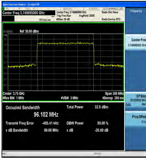
1-N78-3700-3800-30-100-H-1-DFT-QPSK-Outer_Full -270@0-Ant1-96.102-99.66-≤100-PASS
