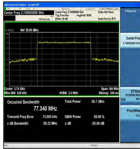
1-N78-3700-3800-30-80-L-6-CP-QPSK-Outer_Full-2 17@0-Ant1-77.340-80.22-≤80-PASS
