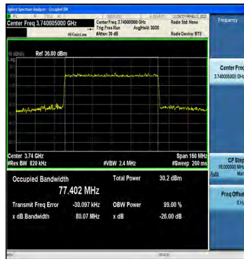
1-N78-3700-3800-30-80-L-8-CP-64QAM-Outer_Full-217@0-Ant1-77.402-80.07-≤80-PASS
