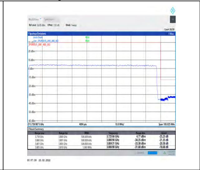
1-N78-3700-3800-30-90-H-3-DFT-PI2BPSK-Outer_Full-240@0-Ant1-PASS-see graph
