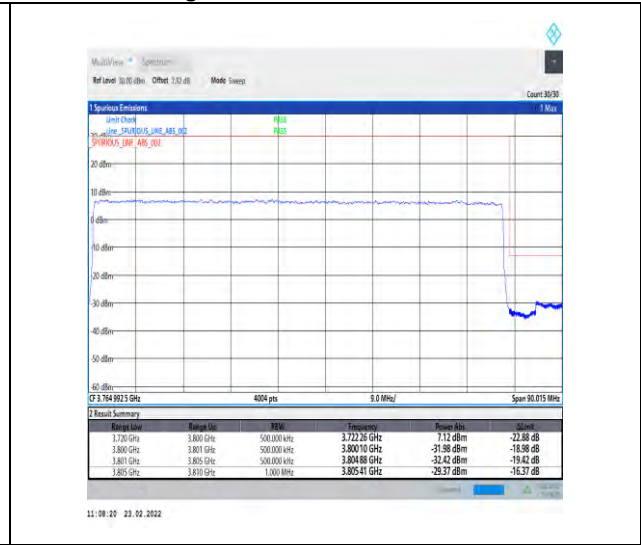
1-N78-3700-3800-30-80-H-3-DFT-PI2BPSK-Outer_Full-216@0-Ant1-PASS-see graph
