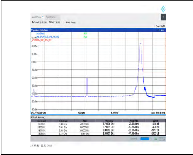
1-N78-3700-3800-30-50-H-5-CP-QPSK-Edge_1RB_Right-1@132-Ant1-PASS-see graph
