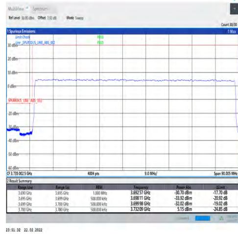
1-N78-3700-3800-30-80-L-3-DFT-PI2BPSK-Outer_Full-216@0-Ant1-PASS-see graph
