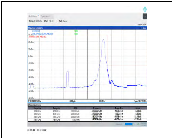
1-N78-3700-3800-30-20-H-2-DFT-PI2BPSK-Edge_1R_B_Right-1@50-Ant1-PASS-see graph
