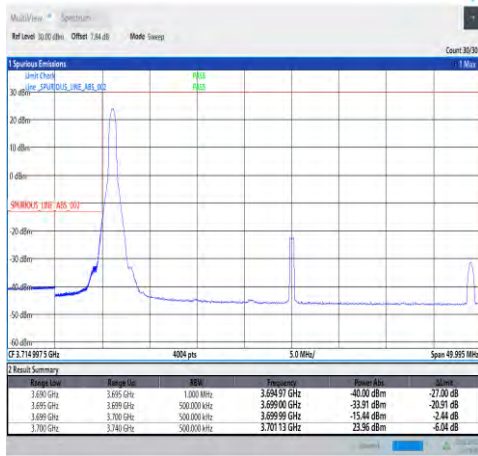
1-N78-3700-3800-30-40-L-1-DFT-PI2BPSK-Edge_1RB _Left-1@0-Ant1-PASS-see graph
