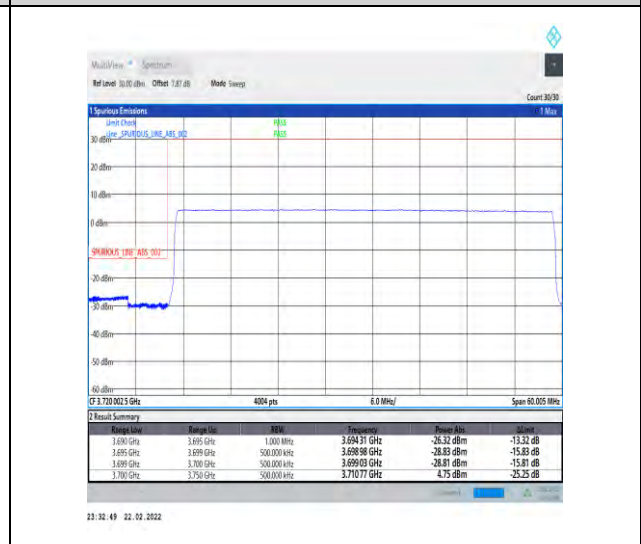
1-N78-3700-3800-30-50-L-6-CP-QPSK-Outer_Full -133@0-Ant1-PASS-see graph
