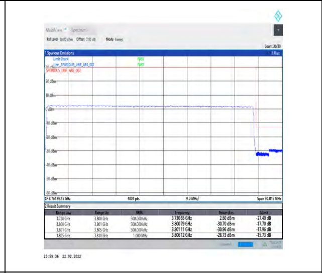
1-N78-3700-3800-30-80-H-6-CP-QPSK-Outer_Full-217@0-Ant1-PASS-see graph
