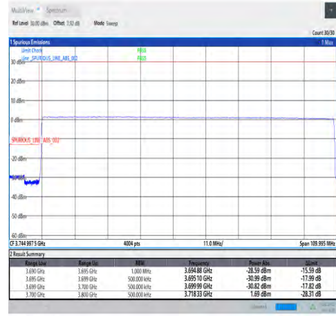
1-N78-3700-3800-30-100-L-6-CP-QPSK-Outer_Fu ll-273@0-Ant1-PASS-see graph
