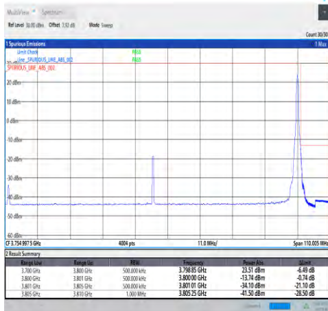
1-N78-3700-3800-30-100-H-5-CP-QPSK-Edge_1RB_Right-1@272-Ant1-PASS-see graph
