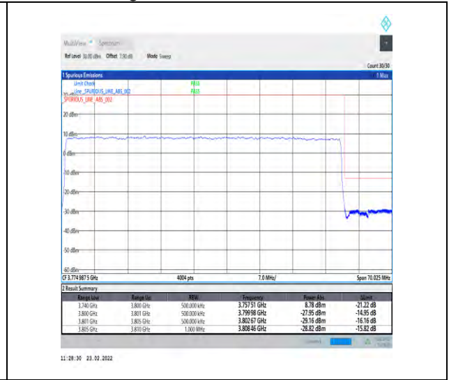
1-N78-3700-3800-30-60-H-3-DFT-PI2BPSK-Outer_Full-162@0-Ant1-PASS-see graph
