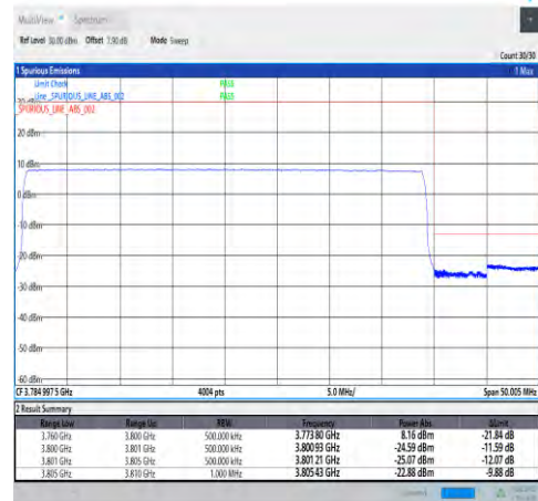
1-N78-3700-3800-30-40-H-6-CP-QPSK-Outer_Full-106@0-Ant1-PASS-see graph
