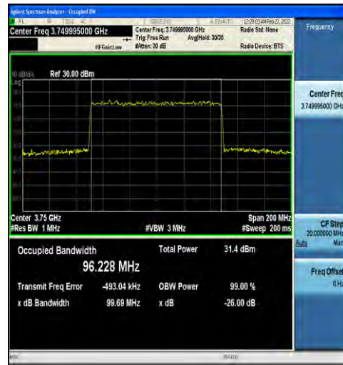
1-N78-3700-3800-30-100-H-4-DFT-64QAM-Outer_Full -270@0-Ant1-96.228-99.69-≤100-PASS
