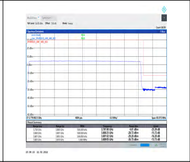
1-N78-3700-3800-30-50-H-6-CP-QPSK-Outer_Full-133@0-Ant1-PASS-see graph
