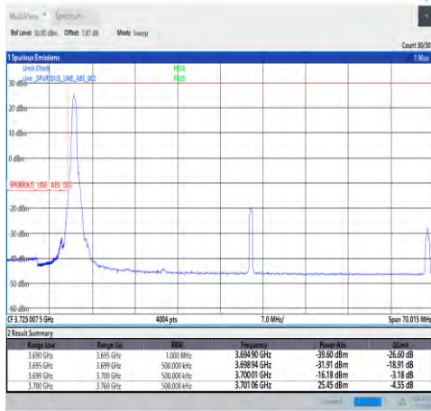
1-N78-3700-3800-30-60-L-1-DFT-PI2BPSK-Edge_1RB_Left-1@0-Ant1-PASS-see graph
