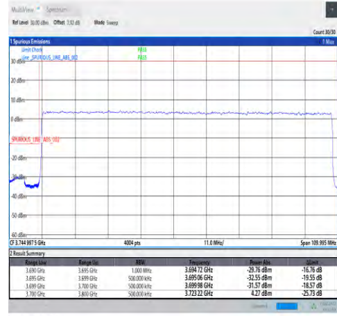
1-N78-3700-3800-30-100-L-3-DFT-PI2BPSK-Outer_Full-270@0-Ant1-PASS-see graph
