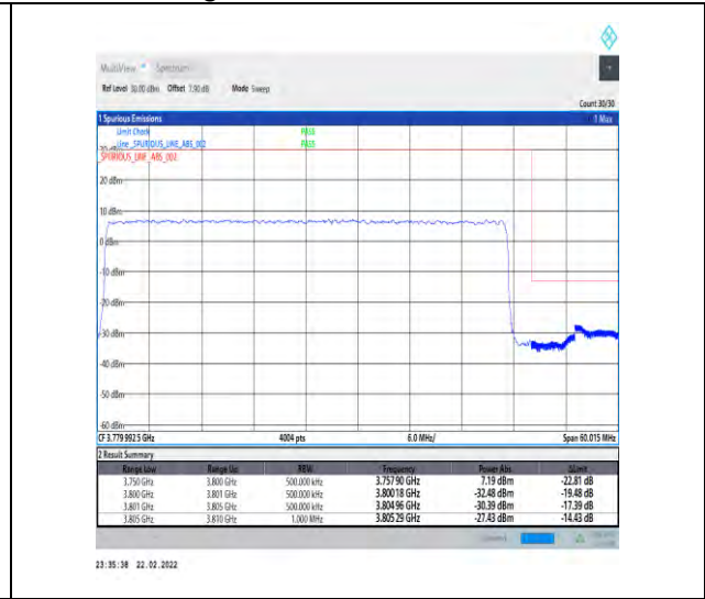
1-N78-3700-3800-30-50-H-3-DFT-PI2BPSK-Outer_Full-128@0-Ant1-PASS-see graph
