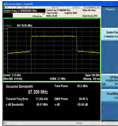
1-N78-3700-3800-30-90-M-8-CP-64QAM-Outer_Full-245@0-Ant1-87.309-90.61-≤90-PASS
