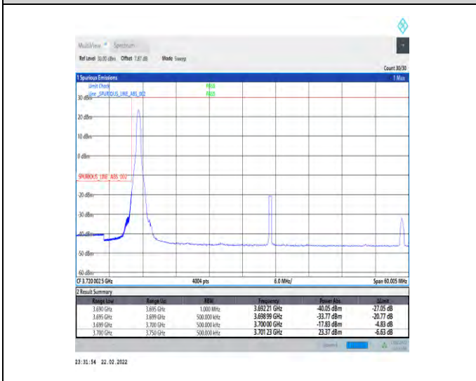
1-N78-3700-3800-30-50-L-4-CP-QPSK-Edge_1RB_Lef t-1@0-Ant1-PASS-see graph
