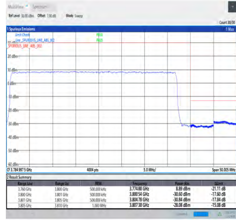
1-N78-3700-3800-30-40-H-3-DFT-PI2BPSK-Outer_Full-100@0-Ant1-PASS-see graph
