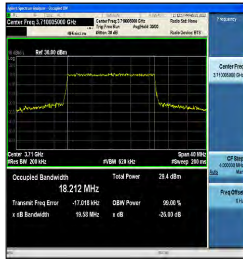
1-N78-3700-3800-30-20-L-6-CP-QPSK-Outer_Full-5 1@0-Ant1-18.212-19.58-<math>\leq 20</math>-PASS
