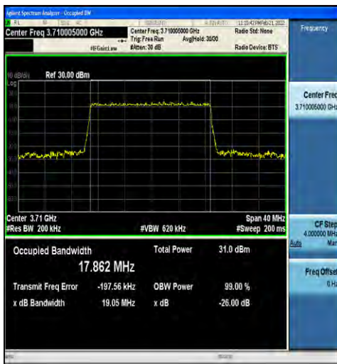
1-N78-3700-3800-30-20-L-3-DFT-16QAM-Outer_Full-50@0-Ant1-17.862-19.05-≤20-PASS
