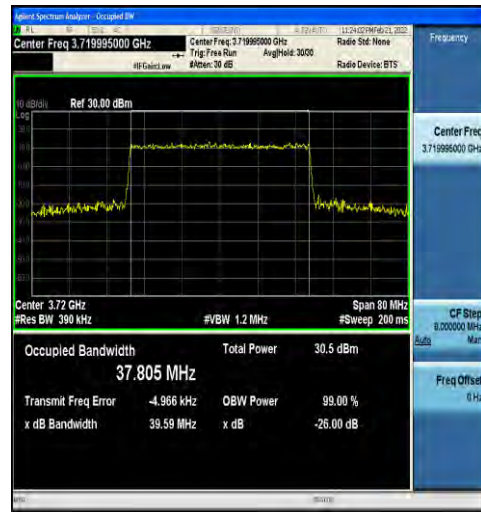
1-N78-3700-3800-30-40-L-7-CP-16QAM-Outer_Full-106@0-Ant1-37.805-39.59-≤40-PASS
