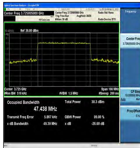
1-N78-3700-3800-30-50-L-6-CP-QPSK-Outer_Full-1 33@0-Ant1-47.438-49.39- \leq 50 -PASS
