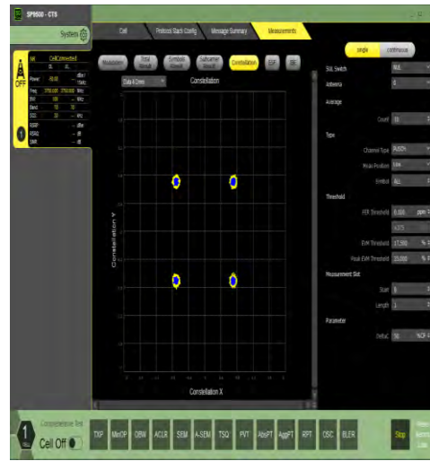
1-N78-3700-3800-30-100-M-6-CP-QPSK-Outer_Full-273@0-Ant1-see graph-PASS
