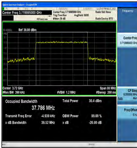
1-N78-3700-3800-30-40-L-6-CP-QPSK-Outer_Full-106@0-Ant1-37.786-39.52-≤40-PASS
