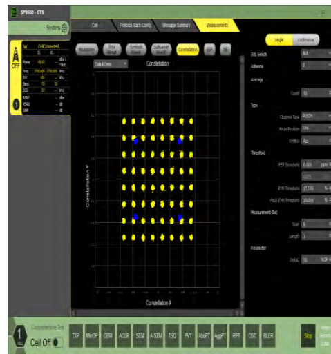
1-N78-3700-3800-30-100-M-8-CP-64QAM-Outer_Full-273@0-Ant1-see graph-PASS
