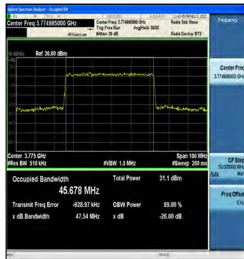
1-N78-3700-3800-30-50-H-4-DFT-64QAM-Outer_Full-128@0-Ant1-45.678-47.54-<math>\leq 50</math>-PASS
