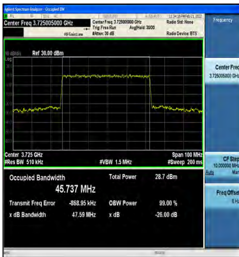
1-N78-3700-3800-30-50-L-5-DFT-256QAM-Outer_Fu II-128@0-Ant1-45.737-47.59- \leq 50 -PASS
