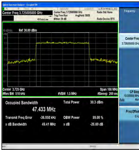
1-N78-3700-3800-30-50-L-7-CP-16QAM-Outer_Full-133@0-Ant1-47.433-49.41-<math>\leq 50</math>-PASS
