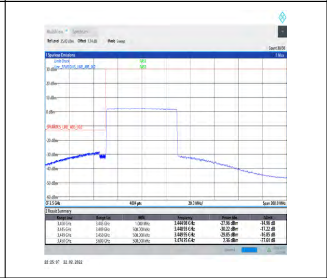
1-N78-3450-3550-30-60-L-6-CP-QPSK-Outer_Full -162@0-Ant1-PASS-see graph
