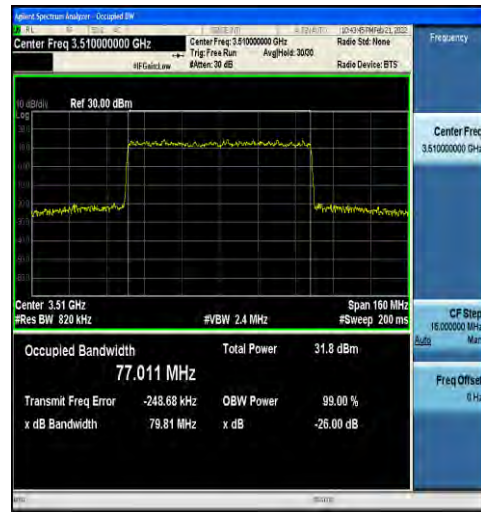
1-N78-3450-3550-30-80-H-4-DFT-64QAM-Outer_Ful I-216@0-Ant1-77.011-79.81-<math>\leq 80</math>-PASS
