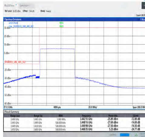
1-N78-3450-3550-30-50-L-6-CP-QPSK-Outer_Full -133@0-Ant1-PASS-see graph
