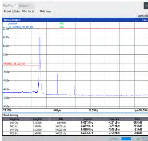
1-N78-3450-3550-30-50-L-4-CP-QPSK-Edge_1RB_Lef t-1@0-Ant1-PASS-see graph
