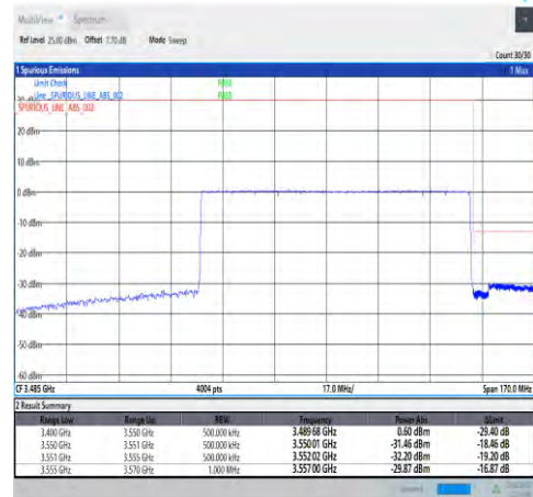
1-N78-3450-3550-30-90-H-6-CP-QPSK-Outer_Full-245@0-Ant1-PASS-see graph
