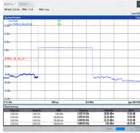
1-N78-3450-3550-30-80-L-3-DFT-PI2BPSK-Outer_Full-216@0-Ant1-PASS-see graph
