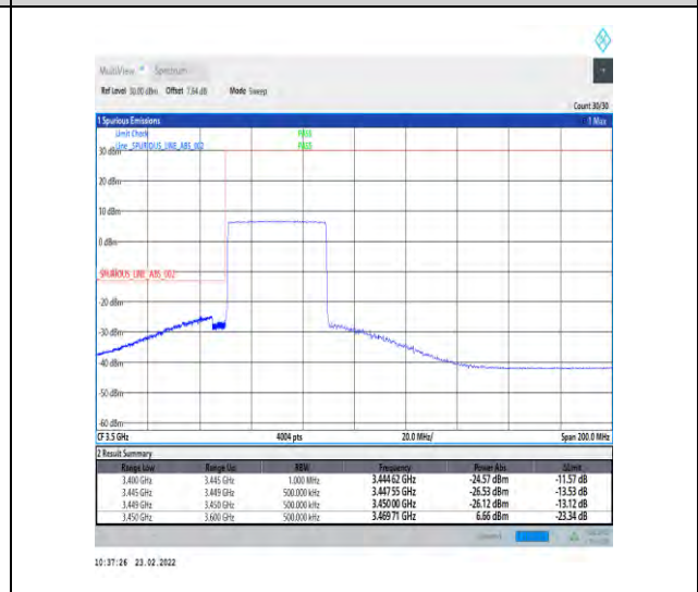
1-N78-3450-3550-30-40-L-6-CP-QPSK-Outer_Full -106@0-Ant1-PASS-see graph
