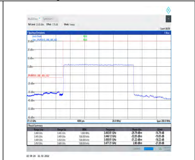
1-N78-3450-3550-30-100-L-3-DFT-PI2BPSK-Outer_Full-270@0-Ant1-PASS-see graph
