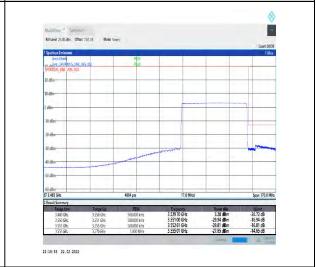
1-N78-3450-3550-30-50-H-6-CP-QPSK-Outer_Full-133@0-Ant1-PASS-see graph
