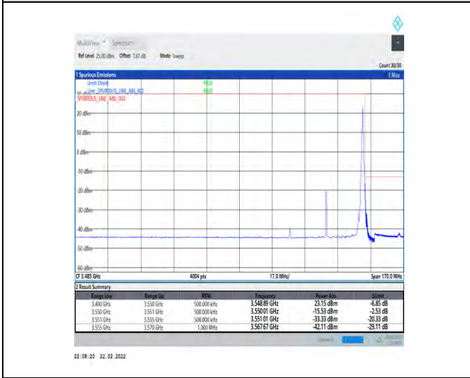
1-N78-3450-3550-30-40-H-5-CP-QPSK-Edge_1RB_Right-1@105-Ant1-PASS-see graph
