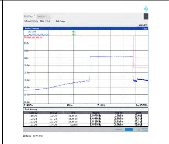
1-N78-3450-3550-30-60-H-6-CP-QPSK-Outer_Full-162@0-Ant1-PASS-see graph
