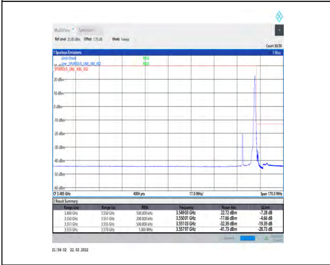
1-N78-3450-3550-30-20-H-5-CP-QPSK-Edge_1RB_Right-1@50-Ant1-PASS-see graph
