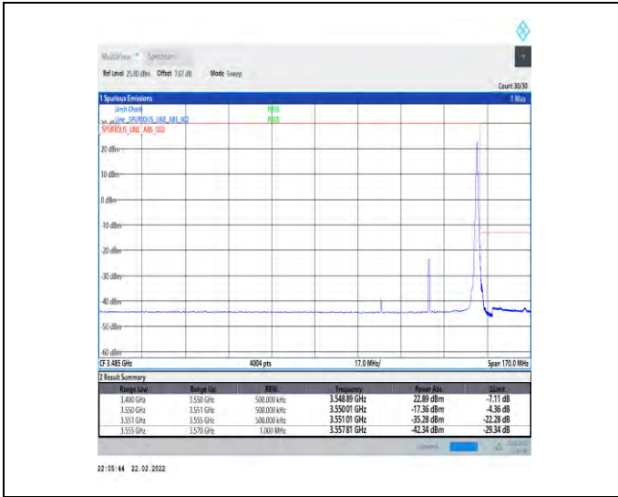
1-N78-3450-3550-30-40-H-2-DFT-PI2BPSK-Edge_1R_B_Right-1@105-Ant1-PASS-see graph
