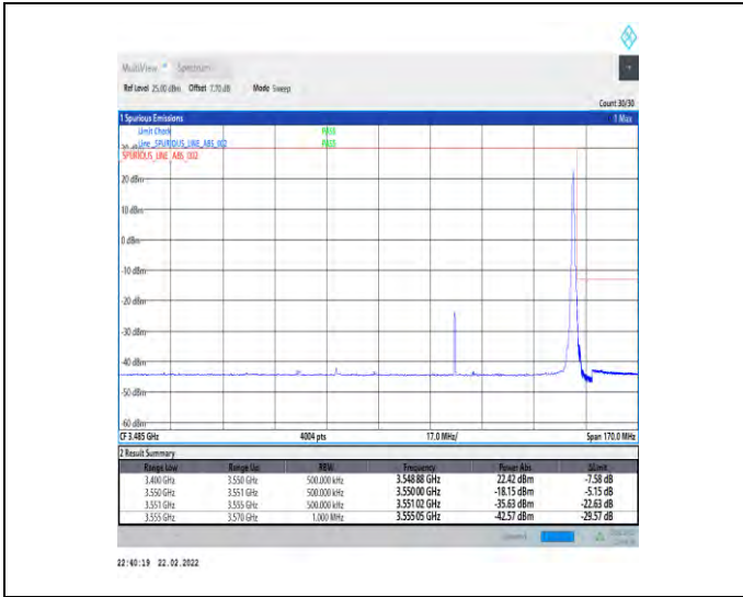
1-N78-3450-3550-30-80-H-2-DFT-PI2BPSK-Edge_1R_B_Right-1@216-Ant1-PASS-see graph
