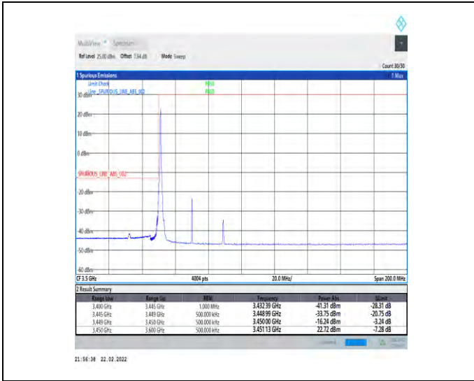
1-N78-3450-3550-30-40-L-1-DFT-PI2BPSK-Edge_1RB_Left-1@0-Ant1-PASS-see graph
