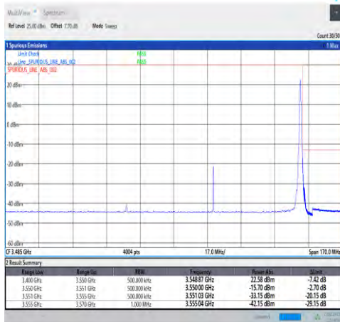
1-N78-3450-3550-30-90-H-5-CP-QPSK-Edge_1RB_Right-1@244-Ant1-PASS-see graph
