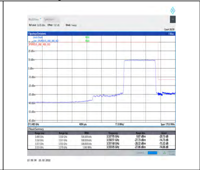
1-N78-3450-3550-30-40-H-3-DFT-PI2BPSK-Outer_Full-100@0-Ant1-PASS-see graph
