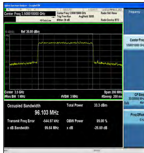
1-N78-3450-3550-30-100-M-1-DFT-QPSK-Outer_Ful l-270@0-Ant1-96.103-99.64-≤100-PASS
