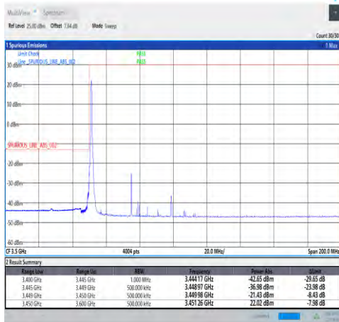
1-N78-3450-3550-30-50-L-1-DFT-PI2BPSK-Edge_1RB_Left-1@0-Ant1-PASS-see graph
