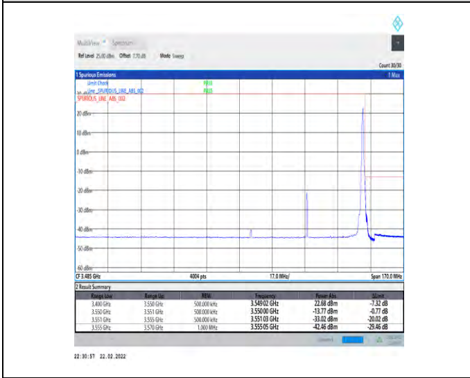
1-N78-3450-3550-30-60-H-5-CP-QPSK-Edge_1RB_Right-1@161-Ant1-PASS-see graph
