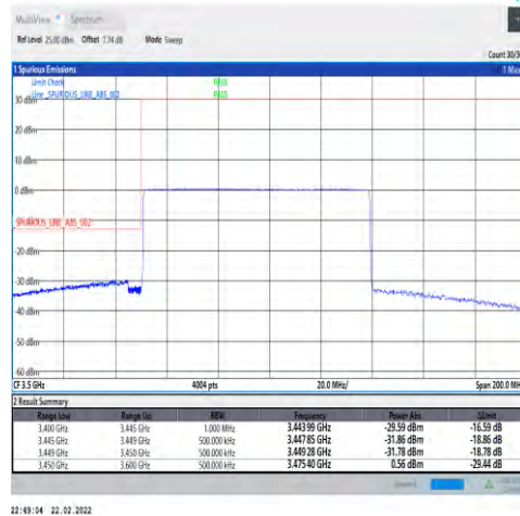
1-N78-3450-3550-30-90-L-6-CP-QPSK-Outer_Full -245@0-Ant1-PASS-see graph
