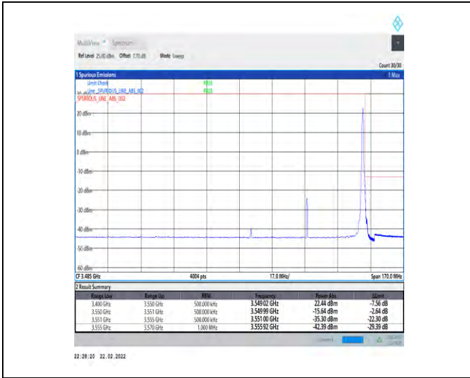
1-N78-3450-3550-30-60-H-2-DFT-PI2BPSK-Edge_1R_B_Right-1@161-Ant1-PASS-see graph
