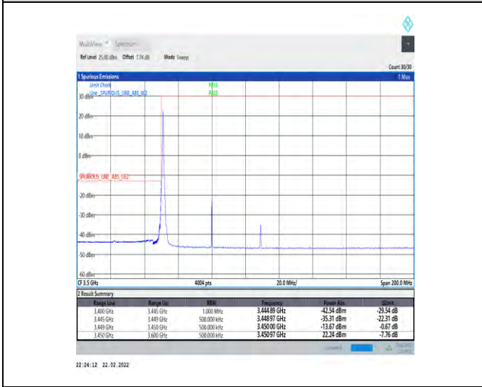
1-N78-3450-3550-30-60-L-4-CP-QPSK-Edge_1RB_Lef t-1@0-Ant1-PASS-see graph
