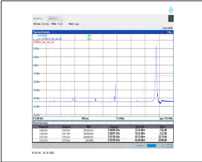
1-N78-3450-3550-30-100-H-2-DFT-PI2BPSK-Edge_1R_B_Right-1@272-Ant1-PASS-see graph
