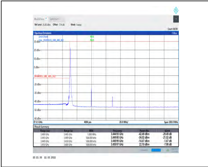
1-N78-3450-3550-30-60-L-1-DFT-PI2BPSK-Edge_1RB_Left-1@0-Ant1-PASS-see graph
