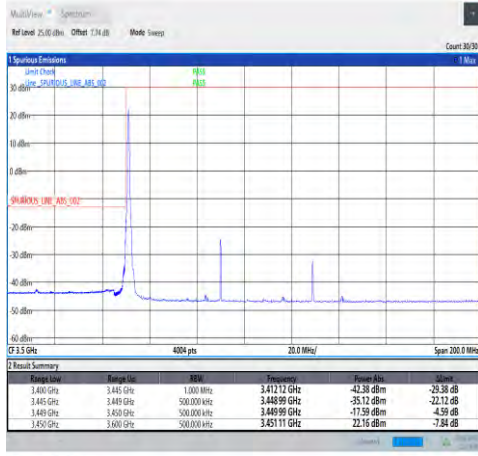
1-N78-3450-3550-30-80-L-1-DFT-PI2BPSK-Edge_1RB_Left-1@0-Ant1-PASS-see graph
