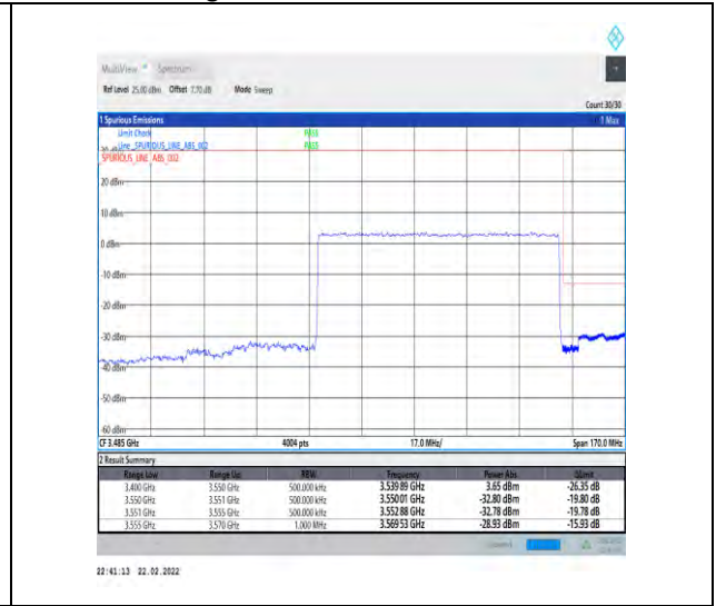
1-N78-3450-3550-30-80-H-3-DFT-PI2BPSK-Outer_Full-216@0-Ant1-PASS-see graph
