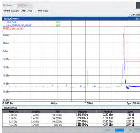
1-N78-3450-3550-30-90-H-2-DFT-PI2BPSK-Edge_1R_B_Right-1@244-Ant1-PASS-see graph
