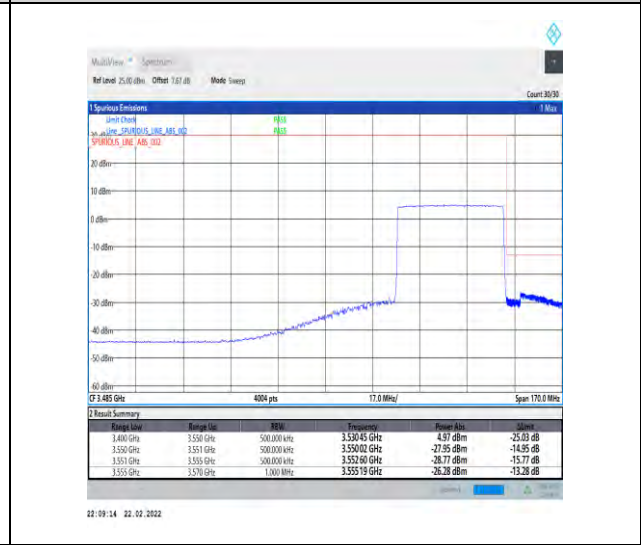
1-N78-3450-3550-30-40-H-6-CP-QPSK-Outer_Full-106@0-Ant1-PASS-see graph
