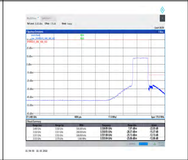
1-N78-3450-3550-30-20-H-6-CP-QPSK-Outer_Full-51@0-Ant1-PASS-see graph
