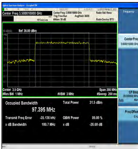
1-N78-3450-3550-30-100-H-7-CP-16QAM-Outer_Ful I-273@0-Ant1-97.395-100.7-≤100-PASS
