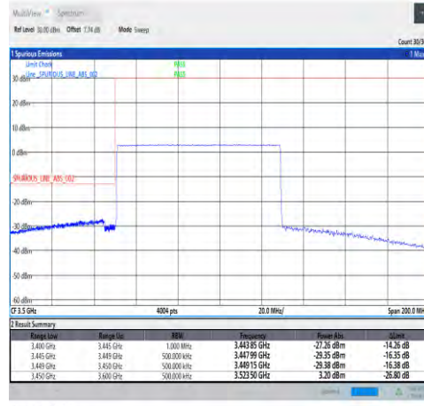
1-N78-3450-3550-30-80-L-6-CP-QPSK-Outer_Full -217@0-Ant1-PASS-see graph
