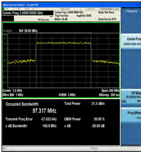
1-N78-3450-3550-30-100-L-7-CP-16QAM-Outer_Full -273@0-Ant1-97.317-100.6-≤100-PASS
