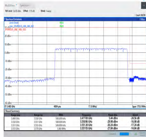
1-N78-3450-3550-30-90-H-3-DFT-PI2BPSK-Outer_Full-240@0-Ant1-PASS-see graph
