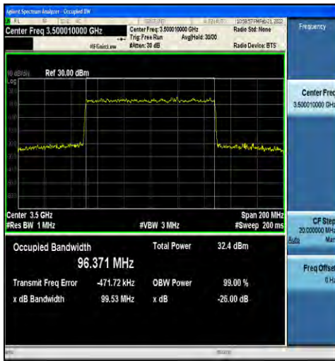
1-N78-3450-3550-30-100-L-3-DFT-16QAM-Outer_Fu ll-270@0-Ant1-96.371-99.53-≤100-PASS
