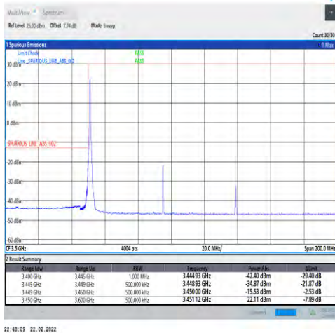
1-N78-3450-3550-30-90-L-4-CP-QPSK-Edge_1RB_Lef t-1@0-Ant1-PASS-see graph
