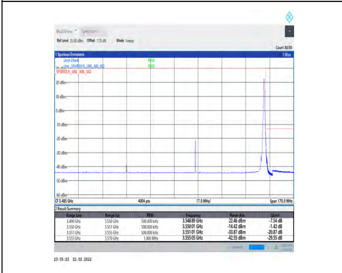
1-N78-3450-3550-30-100-H-5-CP-QPSK-Edge_1RB_Right-1@272-Ant1-PASS-see graph
