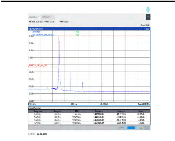
1-N78-3450-3550-30-40-L-4-CP-QPSK-Edge_1RB_Lef t-1@0-Ant1-PASS-see graph
