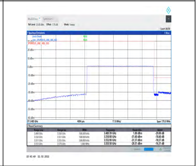
1-N78-3450-3550-30-80-H-6-CP-QPSK-Outer_Full-217@0-Ant1-PASS-see graph
