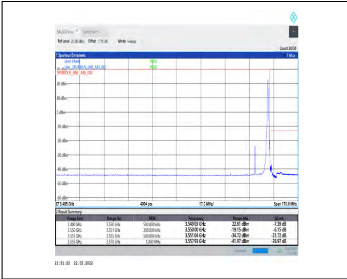
1-N78-3450-3550-30-20-H-2-DFT-PI2BPSK-Edge_1R_B_Right-1@50-Ant1-PASS-see graph
