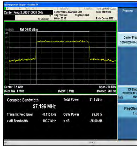
1-N78-3450-3550-30-100-L-8-CP-64QAM-Outer_Full -273@0-Ant1-97.196-100.7-≤100-PASS
