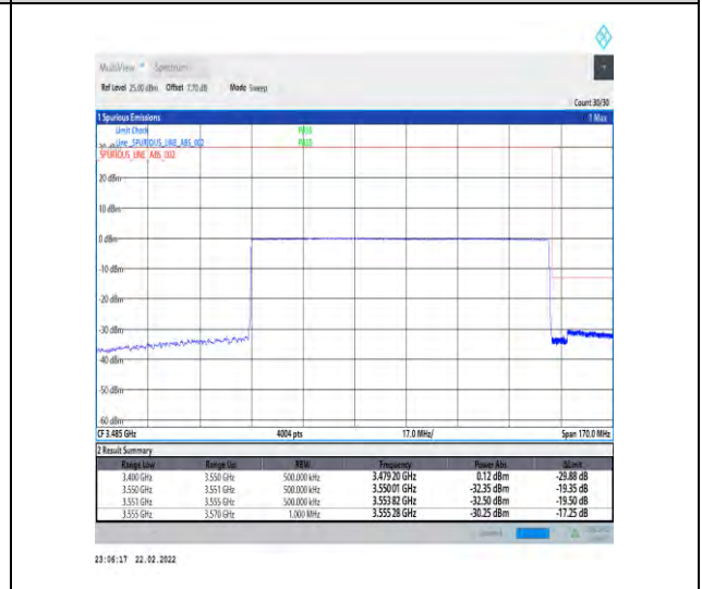
1-N78-3450-3550-30-100-H-6-CP-QPSK-Outer_Full-273@0-Ant1-PASS-see graph
