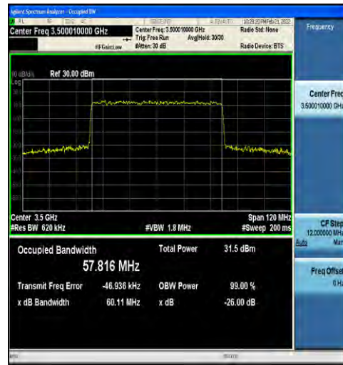
1-N78-3450-3550-30-60-M-4-DFT-64QAM-Outer_Ful I-162@0-Ant1-57.816-60.11-≤60-PASS
