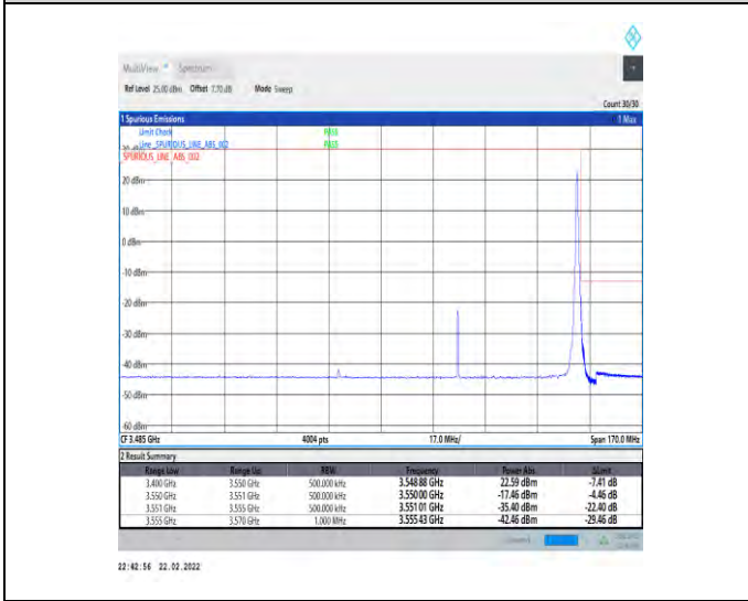
1-N78-3450-3550-30-80-H-5-CP-QPSK-Edge_1RB_Right-1@216-Ant1-PASS-see graph
