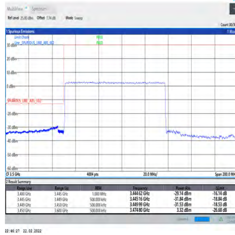
1-N78-3450-3550-30-90-L-3-DFT-PI2BPSK-Outer_Full-240@0-Ant1-PASS-see graph
