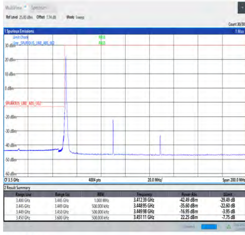
1-N78-3450-3550-30-80-L-4-CP-QPSK-Edge_1RB_Lef t-1@0-Ant1-PASS-see graph
