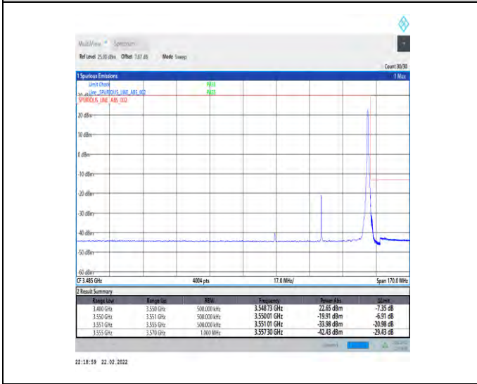
1-N78-3450-3550-30-50-H-5-CP-QPSK-Edge_1RB_Right-1@132-Ant1-PASS-see graph
