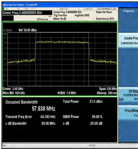
1-N78-3450-3550-30-60-L-4-DFT-64QAM-Outer_Full -162@0-Ant1-57.838-60.08-<math>\leq 60</math>-PASS
