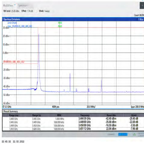
1-N78-3450-3550-30-90-L-1-DFT-PI2BPSK-Edge_1RB_Left-1@0-Ant1-PASS-see graph
