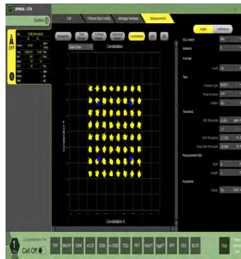
1-N78-3450-3550-30-100-M-8-CP-64QAM-Outer_Full-273@0-Ant1-see graph-PASS
