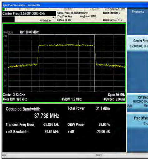
1-N78-3450-3550-30-40-H-8-CP-64QAM-Outer_Full-106@0-Ant1-37.738-39.61-≤40-PASS
