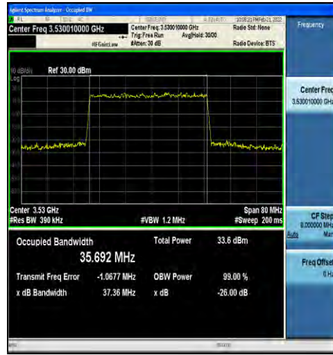
1-N78-3450-3550-30-40-H-1-DFT-QPSK-Outer_Full-100@0-Ant1-35.692-37.36-≤40-PASS
