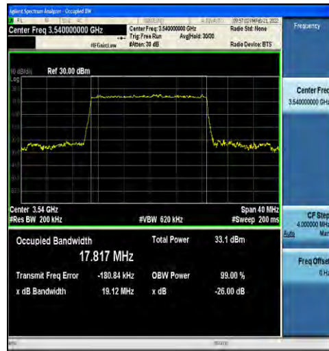
1-N78-3450-3550-30-20-H-2-DFT-PI2BPSK-Outer_Full-50@0-Ant1-17.817-19.12-≤20-PASS
