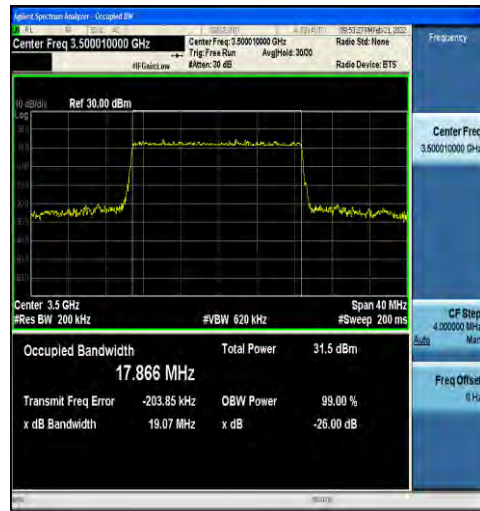
1-N78-3450-3550-30-20-M-3-DFT-16QAM-Outer_Full-50@0-Ant1-17.866-19.07-≤20-PASS
