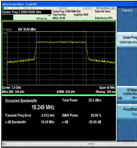
1-N78-3450-3550-30-20-M-8-CP-64QAM-Outer_Full-51@0-Ant1-18.249-19.49-≤20-PASS
