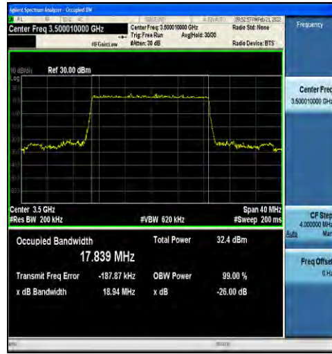
1-N78-3450-3550-30-20-M-1-DFT-QPSK-Outer_Full-50@0-Ant1-17.839-18.94-≤20-PASS
