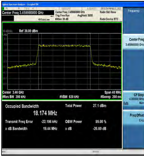
1-N78-3450-3550-30-20-L-9-CP-256QAM-Outer_Full-51@0-Ant1-18.174-19.44-≤20-PASS
