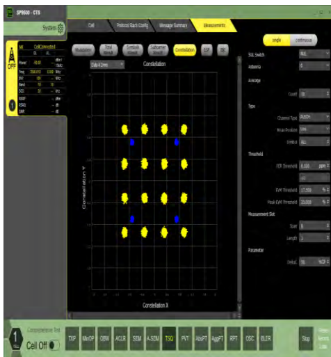
1-N78-3450-3550-30-100-M-7-CP-16QAM-Outer_Full-273@0-Ant1-see graph-PASS
