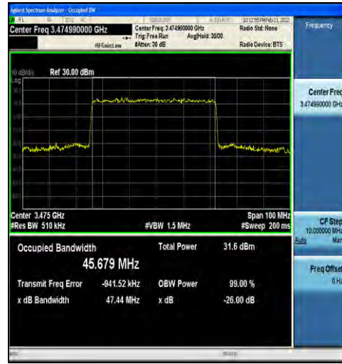
1-N78-3450-3550-30-50-L-4-DFT-64QAM-Outer_Full -128@0-Ant1-45.679-47.44-≤50-PASS
