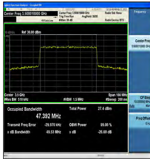
1-N78-3450-3550-30-50-M-9-CP-256QAM-Outer_Full-133@0-Ant1-47.392-49.53-≤50-PASS
