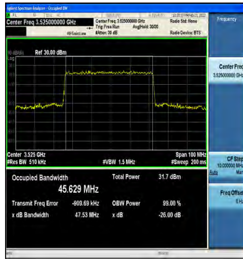
1-N78-3450-3550-30-50-H-4-DFT-64QAM-Outer_Full-128@0-Ant1-45.629-47.53-≤50-PASS
