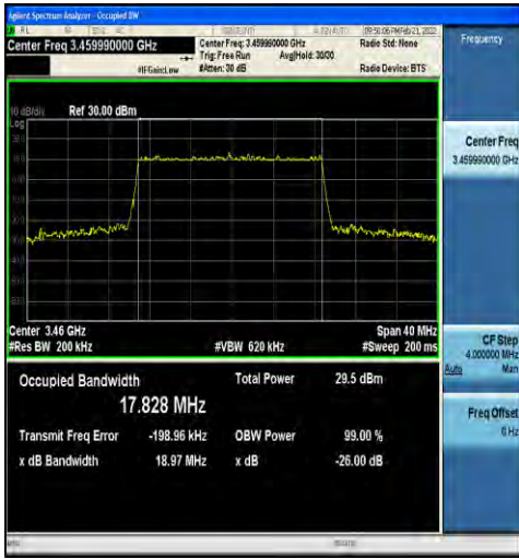
1-N78-3450-3550-30-20-L-5-DFT-256QAM-Outer_Fu II-50@0-Ant1-17.828-18.97- \leq 20 -PASS
