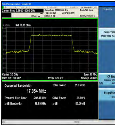
1-N78-3450-3550-30-20-M-4-DFT-64QAM-Outer_Full-50@0-Ant1-17.854-18.85-≤20-PASS
