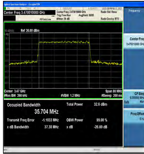
1-N78-3450-3550-30-40-L-3-DFT-16QAM-Outer_Full-100@0-Ant1-35.704-37.38-≤40-PASS
