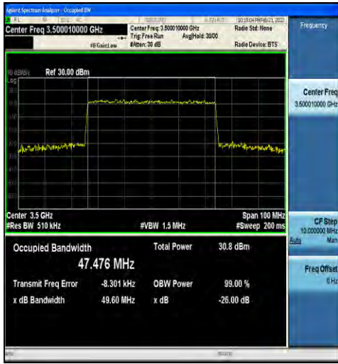
1-N78-3450-3550-30-50-M-6-CP-QPSK-Outer_Full-133@0-Ant1-47.476-49.60-≤50-PASS
