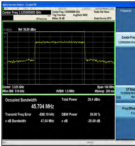
1-N78-3450-3550-30-50-H-5-DFT-256QAM-Outer_Full-128@0-Ant1-45.704-47.64-≤50-PASS
