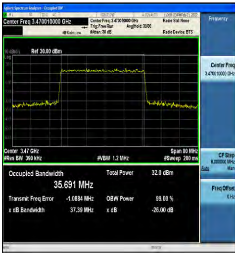
1-N78-3450-3550-30-40-L-4-DFT-64QAM-Outer_Full-100@0-Ant1-35.691-37.39-≤40-PASS
