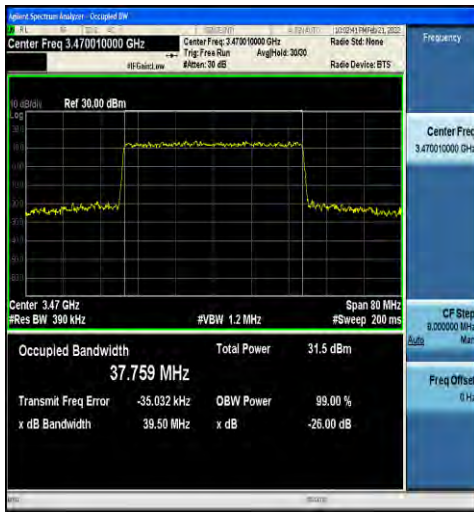
1-N78-3450-3550-30-40-L-6-CP-QPSK-Outer_Full-106@0-Ant1-37.759-39.50-≤40-PASS
