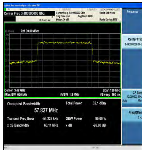
1-N78-3450-3550-30-60-L-3-DFT-16QAM-Outer_Full-162@0-Ant1-57.827-60.14- \leq 60 -PASS
