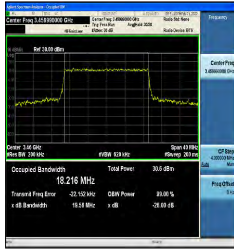
1-N78-3450-3550-30-20-L-6-CP-QPSK-Outer_Full-5 1@0-Ant1-18.216-19.56- \leq 20 -PASS
