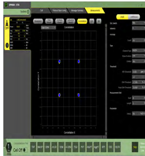
1-N78-3450-3550-30-100-M-6-CP-QPSK-Outer_Full-273@0-Ant1-see graph-PASS
