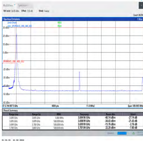
1-N77-3700-3980-30-100-L-1-DFT-PI2BPSK-Edge_1R_B_Left-1@0-Ant1-PASS-see graph
