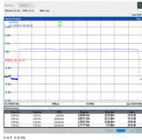
1-N77-3700-3980-30-90-L-3-DFT-PI2BPSK-Outer_Full-240@0-Ant1-PASS-see graph
