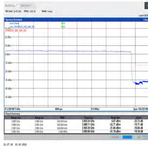
1-N77-3700-3980-30-90-H-3-DFT-PI2BPSK-Outer_Full-240@0-Ant1-PASS-see graph
