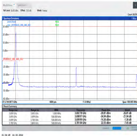
1-N77-3700-3980-30-100-L-4-CP-QPSK-Edge_1RB_L_eft-1@0-Ant1-PASS-see graph
