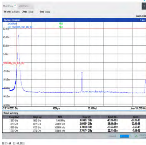
1-N77-3700-3980-30-90-L-4-CP-QPSK-Edge_1RB_Lef t-1@0-Ant1-PASS-see graph
