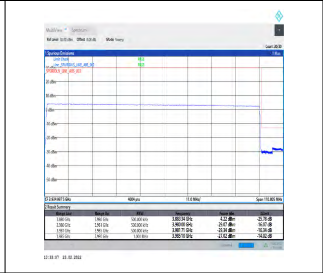
1-N77-3700-3980-30-100-H-6-CP-QPSK-Outer_Full-273@0-Ant1-PASS-see graph
