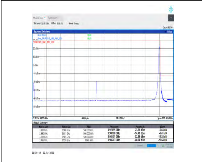
1-N77-3700-3980-30-100-H-5-CP-QPSK-Edge_1RB_Right-1@272-Ant1-PASS-see graph
