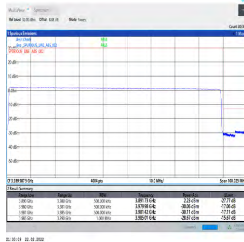
1-N77-3700-3980-30-90-H-6-CP-QPSK-Outer_Full-245@0-Ant1-PASS-see graph
