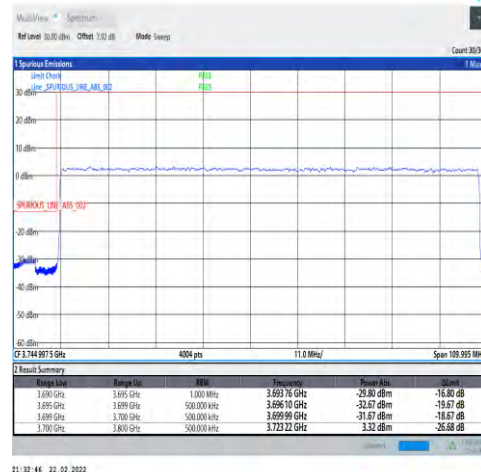
1-N77-3700-3980-30-100-L-3-DFT-PI2BPSK-Outer_Full-270@0-Ant1-PASS-see graph
