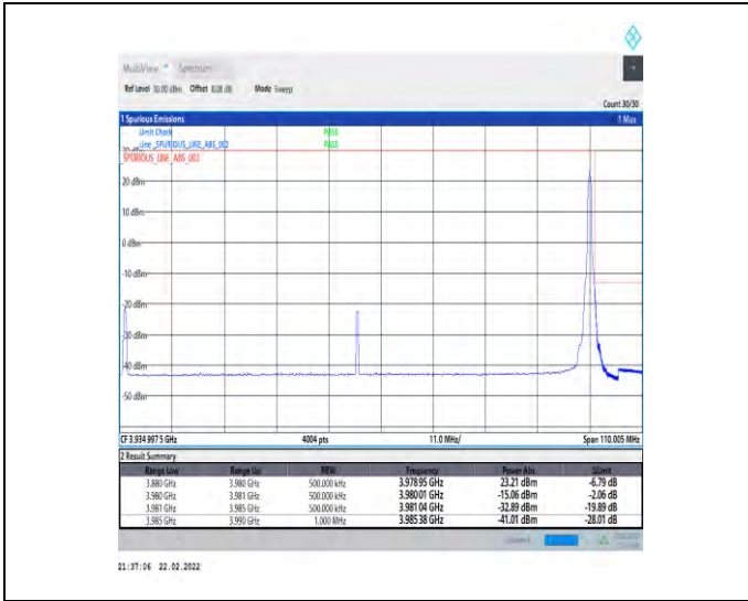
1-N77-3700-3980-30-100-H-2-DFT-PI2BPSK-Edge_1R_B_Right-1@272-Ant1-PASS-see graph
