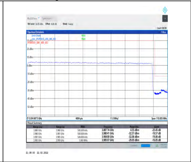
1-N77-3700-3980-30-100-H-3-DFT-PI2BPSK-Outer_Full-270@0-Ant1-PASS-see graph
