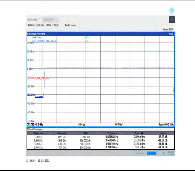
1-N77-3700-3980-30-80-L-6-CP-QPSK-Outer_Full -217@0-Ant1-PASS-see graph
