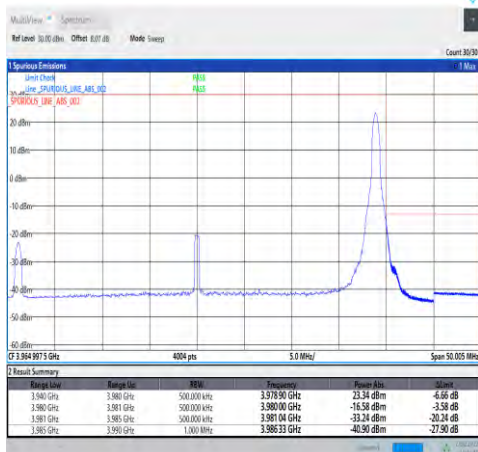
1-N77-3700-3980-30-40-H-5-CP-QPSK-Edge_1RB_Right-1@105-Ant1-PASS-see graph
