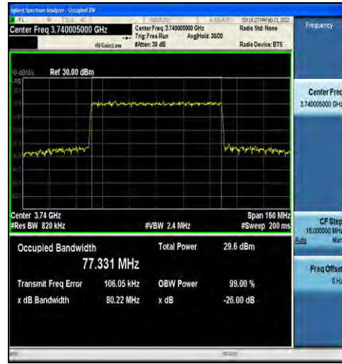
1-N77-3700-3980-30-80-L-6-CP-QPSK-Outer_Full-2 17@0-Ant1-77.331-80.22-≤80-PASS
