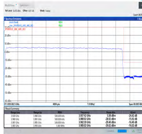
1-N77-3700-3980-30-60-H-3-DFT-PI2BPSK-Outer_Full-162@0-Ant1-PASS-see graph
