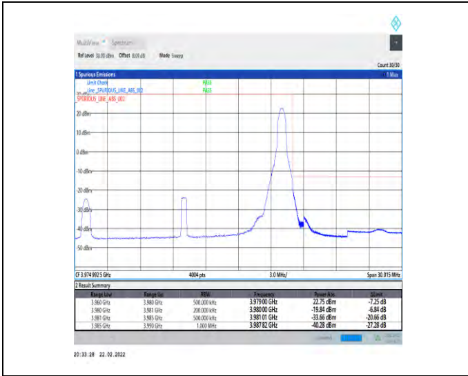
1-N77-3700-3980-30-20-H-2-DFT-PI2BPSK-Edge_1R_B_Right-1@50-Ant1-PASS-see graph
