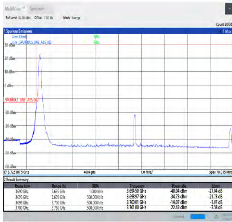
1-N77-3700-3980-30-60-L-4-CP-QPSK-Edge_1RB_Left-1@0-Ant1-PASS-see graph
