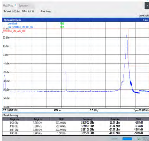
1-N77-3700-3980-30-60-H-5-CP-QPSK-Edge_1RB_Right-1@161-Ant1-PASS-see graph
