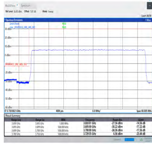
1-N77-3700-3980-30-50-L-3-DFT-PI2BPSK-Outer_Full-128@0-Ant1-PASS-see graph
