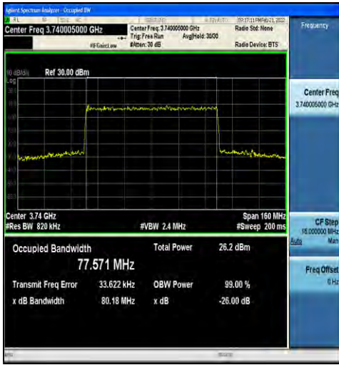
1-N77-3700-3980-30-80-L-9-CP-256QAM-Outer_Full -217@0-Ant1-77.571-80.18-≤80-PASS
