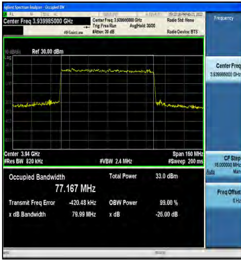
1-N77-3700-3980-30-80-H-3-DFT-16QAM-Outer_Ful I-216@0-Ant1-77.167-79.99-≤80-PASS
