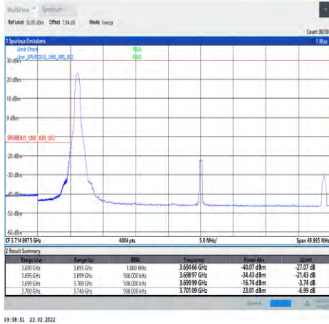
1-N77-3700-3980-30-40-L-1-DFT-PI2BPSK-Edge_1RB _Left-1@0-Ant1-PASS-see graph
