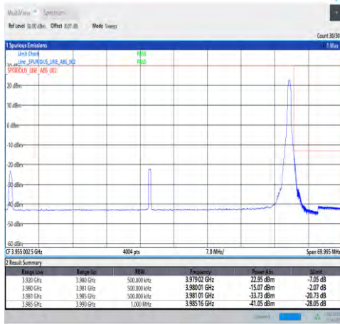
1-N77-3700-3980-30-60-H-2-DFT-PI2BPSK-Edge_1R_B_Right-1@161-Ant1-PASS-see graph
