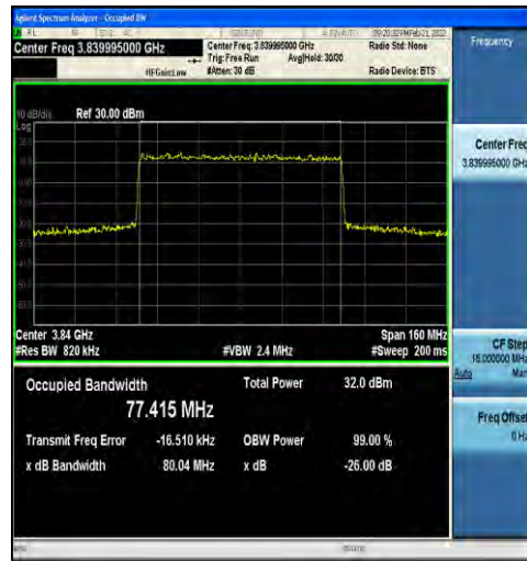
1-N77-3700-3980-30-80-M-7-CP-16QAM-Outer_Full -217@0-Ant1-77.415-80.04-≤80-PASS
