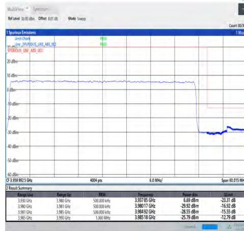
1-N77-3700-3980-30-50-H-3-DFT-PI2BPSK-Outer_Full-128@0-Ant1-PASS-see graph
