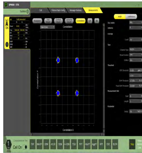
1-N77-3700-3980-30-100-M-6-CP-QPSK-Outer_Full-273@0-Ant1-see graph-PASS
