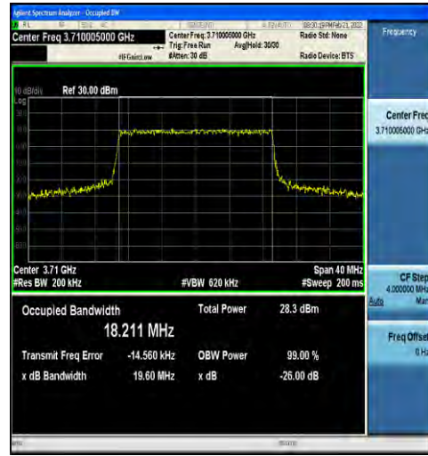
1-N77-3700-3980-30-20-L-6-CP-QPSK-Outer_Full-5 1@0-Ant1-18.211-19.60-≤20-PASS
