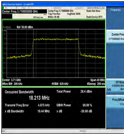
1-N77-3700-3980-30-20-L-7-CP-16QAM-Outer_Full-51@0-Ant1-18.213-19.44-≤20-PASS
