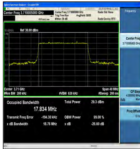
1-N77-3700-3980-30-20-L-4-DFT-64QAM-Outer_Full-50@0-Ant1-17.834-18.76-≤20-PASS
