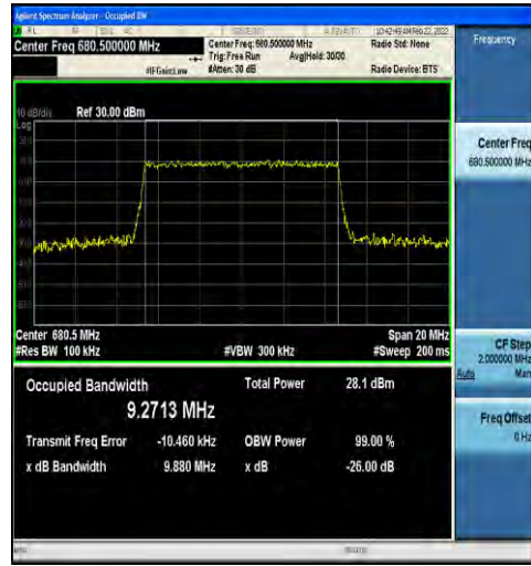
1-N71-15-10-M-6-CP-QPSK-Outer_Full-52@0-Ant1- 9.2713-9.880-≤10-PASS
