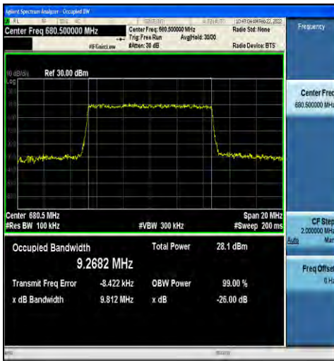
1-N71-15-10-M-7-CP-16QAM-Outer_Full-52@0-Ant 1-9.2682-9.812-≤10-PASS
