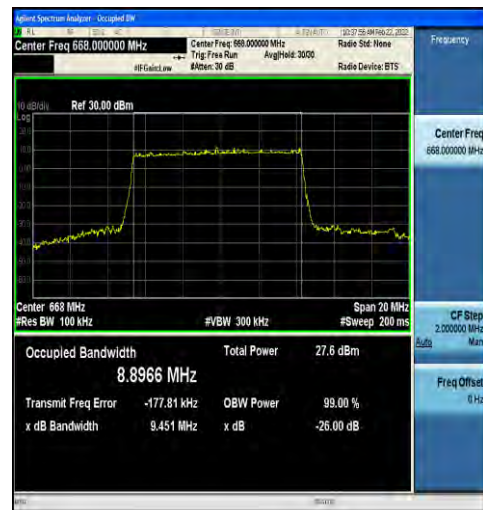
1-N71-15-10-L-5-DFT-256QAM-Outer_Full-50@0-Ant t1-8.8966-9.451-≤10-PASS
