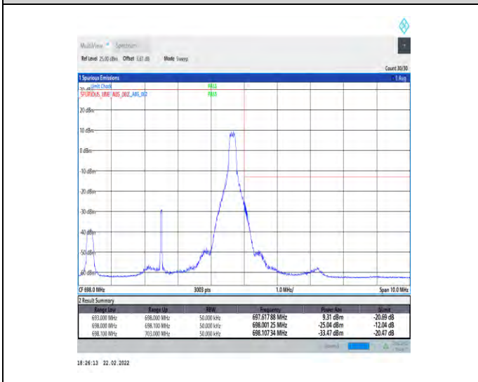
1-N71-15-5-H-5-CP-QPSK-Edge_1RB_Right-1@24-Ant1-PASS-see graph
