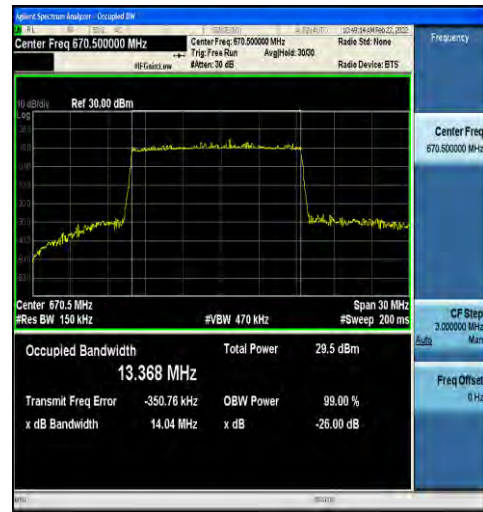
1-N71-15-15-L-4-DFT-64QAM-Outer_Full-75@0-Ant 1-13.368-14.04-≤15-PASS
