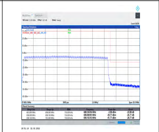
1-N71-15-15-H-6-CP-QPSK-Outer_Full-79@0-Ant1-PASS-see graph
