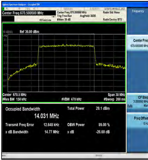
1-N71-15-15-L-7-CP-16QAM-Outer_Full-79@0-Ant1 -14.031-14.77-≤15-PASS
