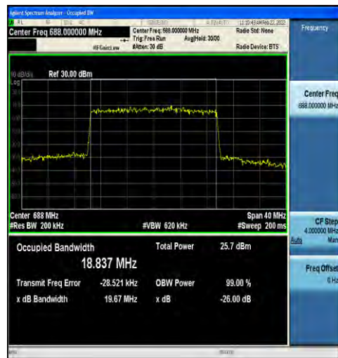
1-N71-15-20-H-9-CP-256QAM-Outer_Full-106@0-Ant1 1-18.837-19.67-≤20-PASS
