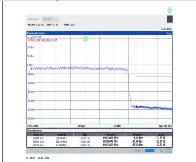
1-N71-15-15-H-3-DFT-P12BPSK-Outer_Full-75@0-Ant1-PASS-see graph
