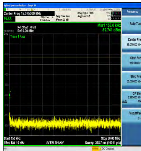
1-N71-15-20-M-1-DFT-PI2BPSK-Inner_1RB_Left-1@ 1-0.15-30-Ant1--62.74--23-PASS
