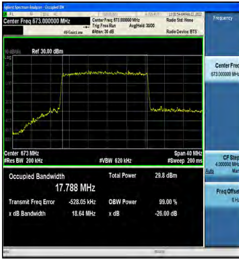
1-N71-15-20-L-4-DFT-64QAM-Outer_Full-100@0-An t1-17.788-18.64-≤20-PASS
