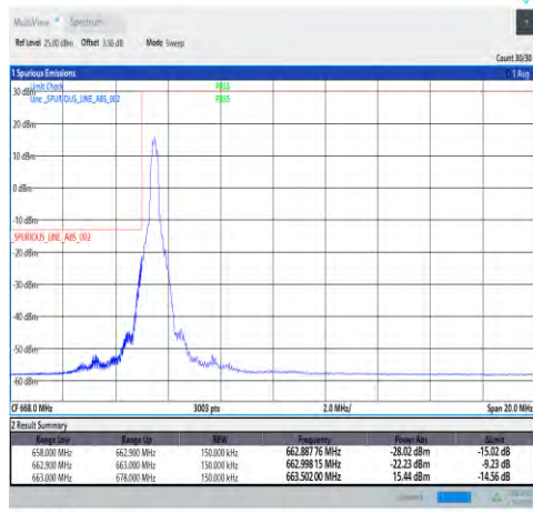
1-N71-15-15-L-1-DFT-PI2BPSK-Edge_1RB_Left-1@0-Ant1-PASS-see graph
