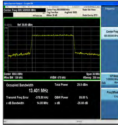
1-N71-15-15-M-3-DFT-16QAM-Outer_Full-75@0-Ant 1-13.401-14.08-≤15-PASS
