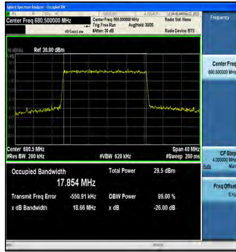
1-N71-15-20-M-4-DFT-64QAM-Outer_Full-100@0-A nt1-17.854-18.66-≤20-PASS
