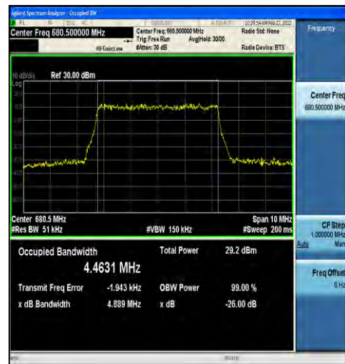
1-N71-15-5-M-3-DFT-16QAM-Outer_Full-25@0-Ant1 -4.4631-4.889-≤5-PASS
