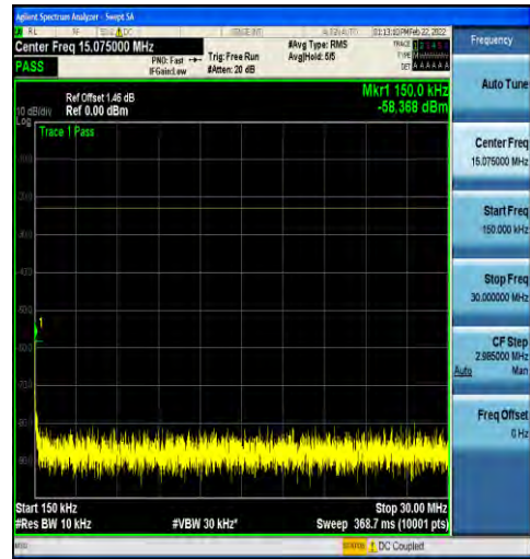
1-N71-15-20-L-1-DFT-PI2BPSK-Inner_1RB_Left-1@ 1-0.15-30-Ant1--58.37--23-PASS
