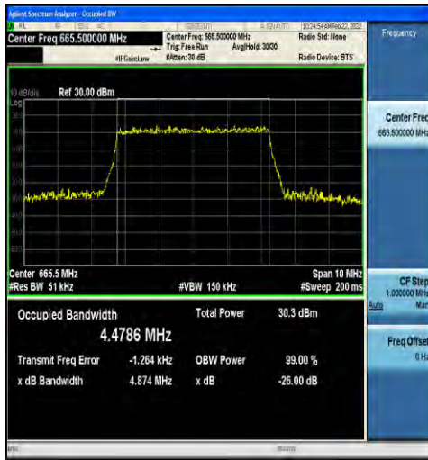
1-N71-15-5-L-1-DFT-QPSK-Outer_Full-25@0-Ant1-4 .4786-4.874-≤5-PASS
