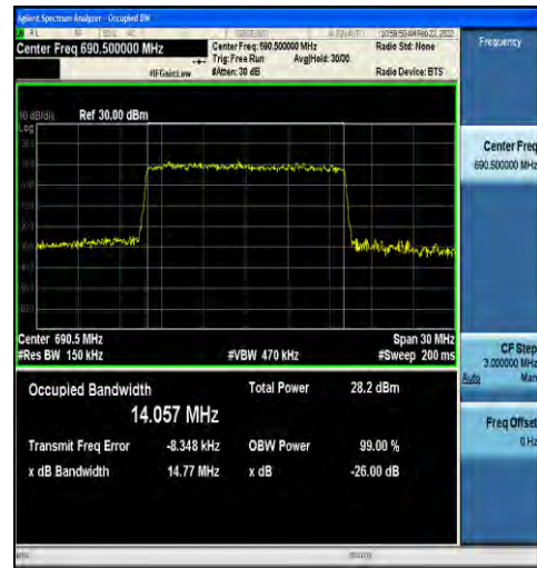
1-N71-15-15-H-8-CP-64QAM-Outer_Full-79@0-Ant1 -14.057-14.77-≤15-PASS
