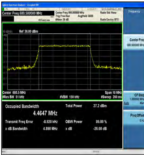
1-N71-15-5-M-6-CP-QPSK-Outer_Full-25@0-Ant1-4 .4647-4.890-≤5-PASS
