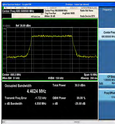
1-N71-15-5-M-2-DFT-P12BPSK-Outer_Full-25@0-An t1-4.4624-4.858-≤5-PASS
