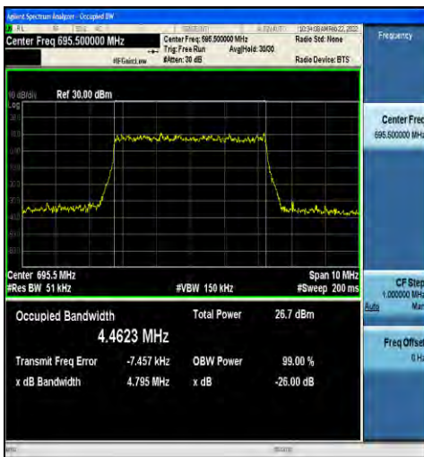
1-N71-15-5-H-5-DFT-256QAM-Outer_Full-25@0-Ant 1-4.4623-4.795-≤5-PASS
