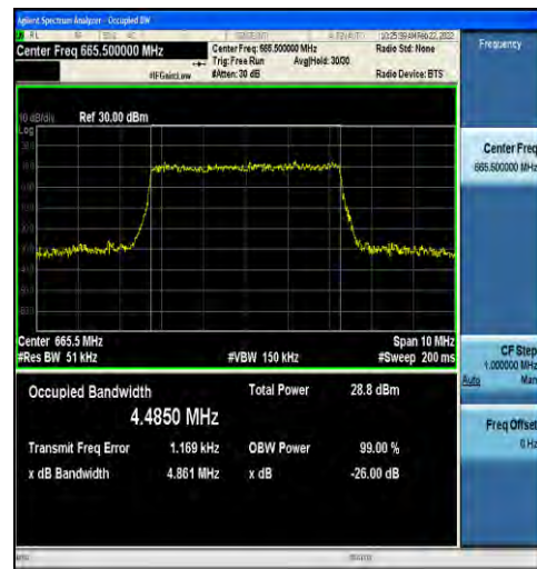
1-N71-15-5-L-4-DFT-64QAM-Outer_Full-25@0-Ant1- 4.4850-4.861-≤5-PASS
