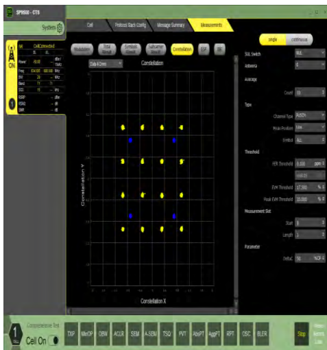
1-N71-15-20-M-7-CP-16QAM-Outer_Full-106@0-Ant1-see graph-PASS
