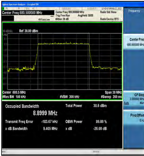
1-N71-15-10-M-1-DFT-QPSK-Outer_Full-50@0-Ant1 -8.8999-9.405≤10-PASS
