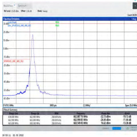
1-N71-15-20-L-1-DFT-PI2BPSK-Edge_1RB_Left-1@0-Ant1-PASS-see graph
