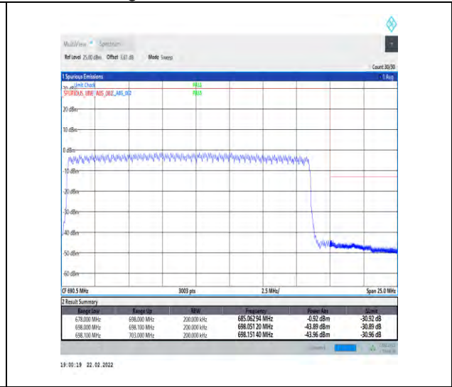
1-N71-15-20-H-3-DFT-PI2BPSK-Outer_Full-100@0-Ant1-PASS-see graph
