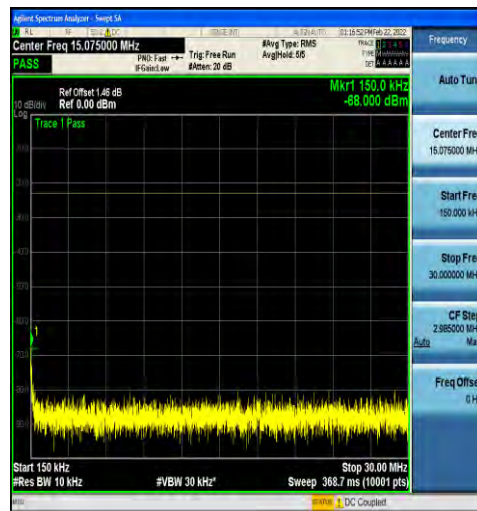
1-N71-15-20-H-1-DFT-PI2BPSK-Inner_1RB_Left-1@ 1-0.15-30-Ant1--68.00--23-PASS
