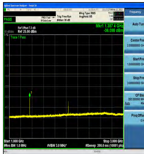
1-N71-15-20-H-1-DFT-PI2BPSK-Inner_1RB_Left-1@ 1-1000-3000-Ant1--36.10--13-PASS
