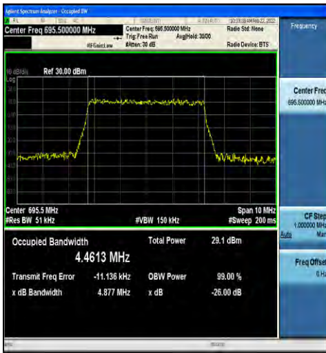
1-N71-15-5-H-3-DFT-16QAM-Outer_Full-25@0-Ant1 -4.4613-4.877-≤5-PASS
