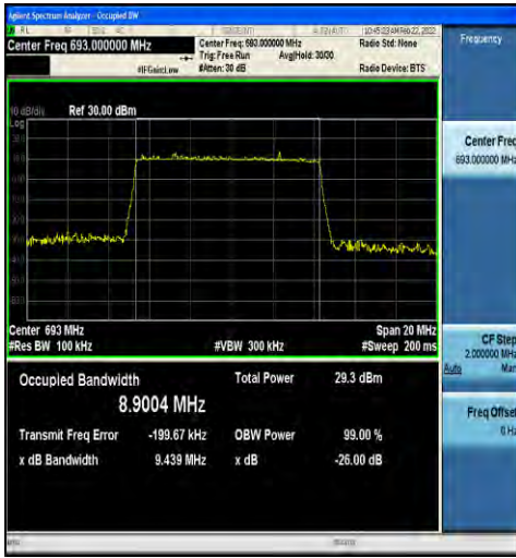
1-N71-15-10-H-4-DFT-64QAM-Outer_Full-50@0-Ant 1-8.9004-9.439-≤10-PASS
