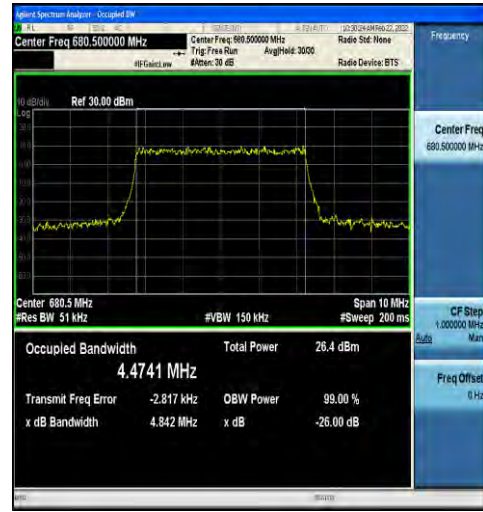
1-N71-15-5-M-5-DFT-256QAM-Outer_Full-25@0-Ant 1-4.4741-4.842-≤5-PASS
