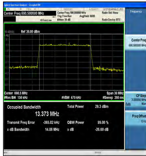
1-N71-15-15-H-4-DFT-64QAM-Outer_Full-75@0-Ant 1-13.373-14.06≤15-PASS
