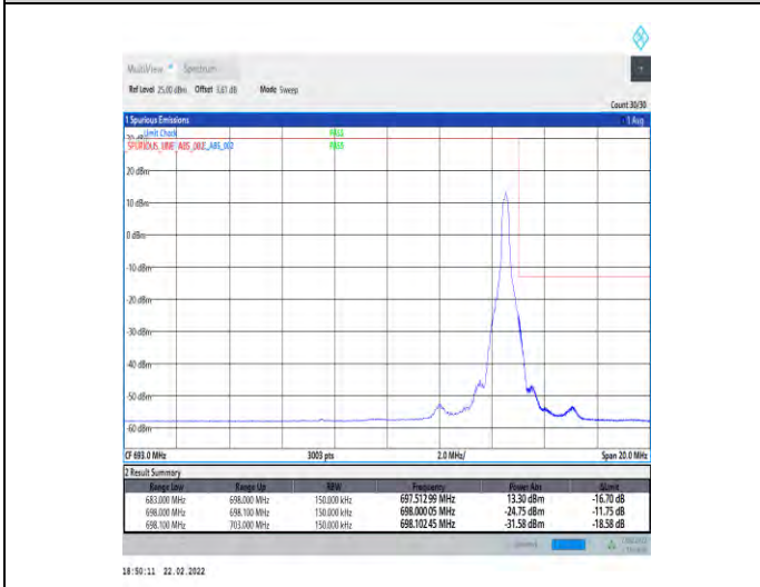
1-N71-15-15-H-5-CP-QPSK-Edge_1RB_Right-1@78-Ant1-PASS-see graph
