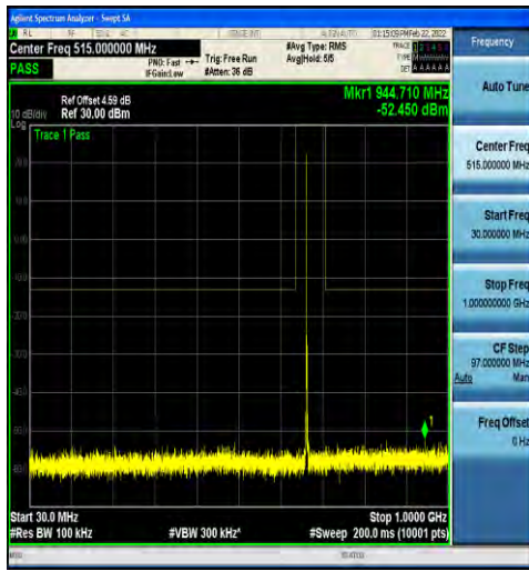
1-N71-15-20-M-1-DFT-PI2BPSK-Inner_1RB_Left-1 @1-30-1000-Ant1--52.45--13-PASS
