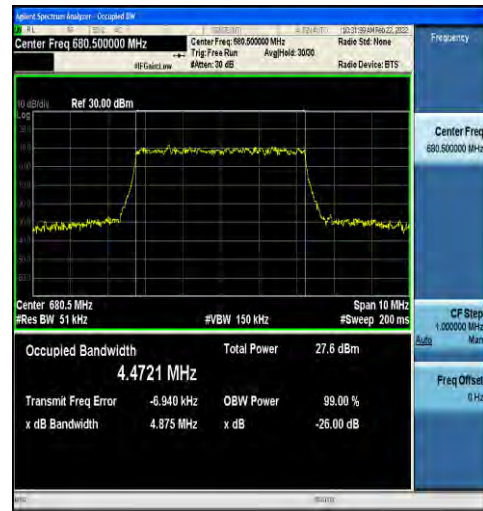
1-N71-15-5-M-7-CP-16QAM-Outer_Full-25@0-Ant1- 4.4721-4.875-≤5-PASS
