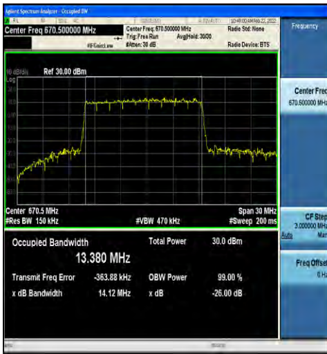
1-N71-15-15-L-3-DFT-16QAM-Outer_Full-75@0-Ant 1-13.380-14.12-≤15-PASS
