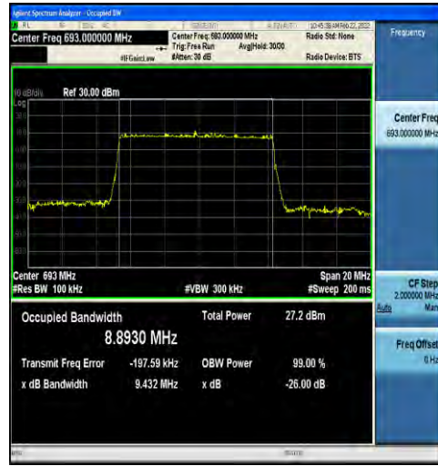
1-N71-15-10-H-5-DFT-256QAM-Outer_Full-50@0-A nt1-8.8930-9.432-≤10-PASS
