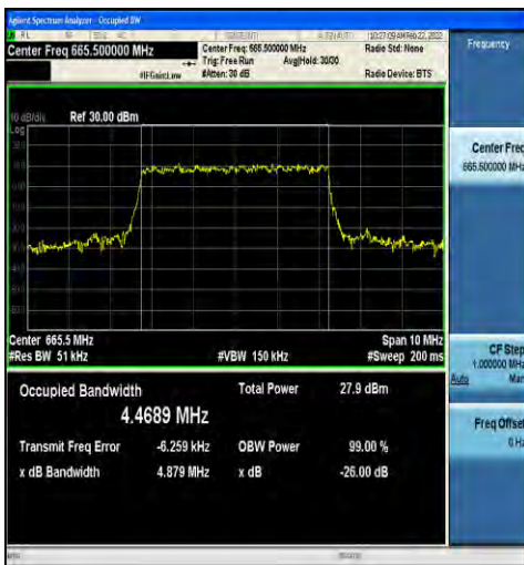
1-N71-15-5-L-7-CP-16QAM-Outer_Full-25@0-Ant1- 4.4689-4.879-≤5-PASS
