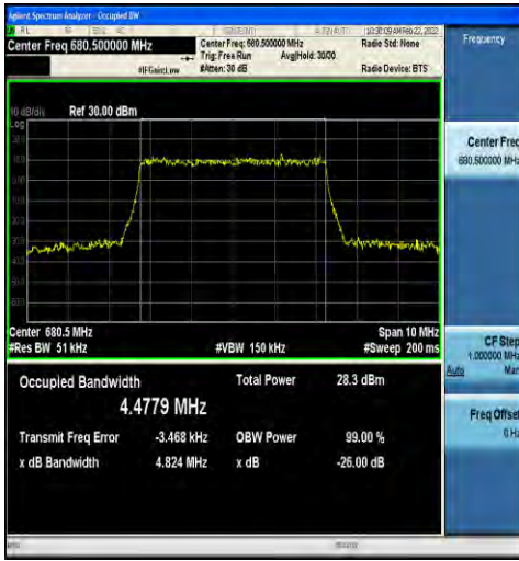
1-N71-15-5-M-4-DFT-64QAM-Outer_Full-25@0-Ant1 -4.4779-4.824-≤5-PASS
