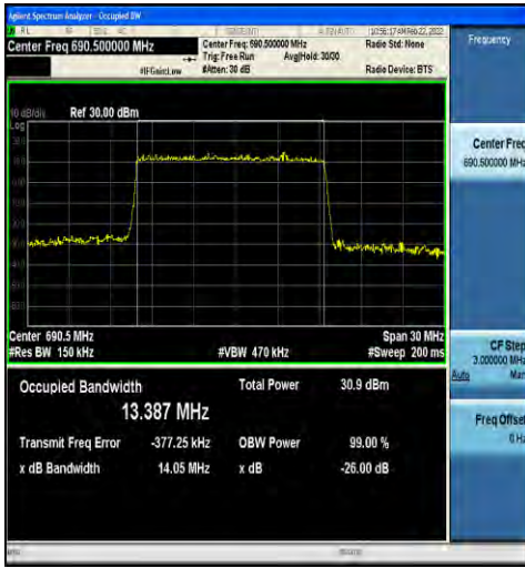
1-N71-15-15-H-1-DFT-QPSK-Outer_Full-75@0-Ant1 -13.387-14.05≤15-PASS
