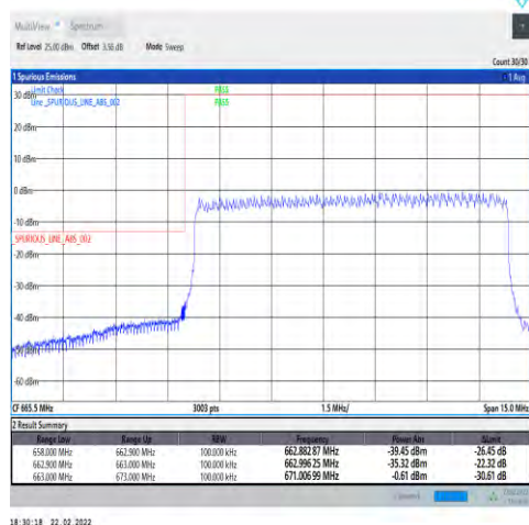
1-N71-15-10-L-3-DFT-PI2BPSK-Outer_Full-50@0-Ant1-PASS-see graph
