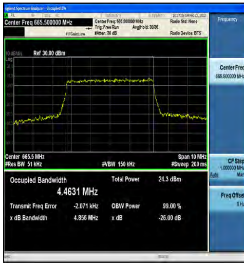
1-N71-15-5-L-9-CP-256QAM-Outer_Full-25@0-Ant1 -4.4631-4.856-≤5-PASS
