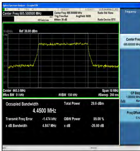
1-N71-15-5-L-3-DFT-16QAM-Outer_Full-25@0-Ant1 -4.4500-4.847-≤5-PASS
