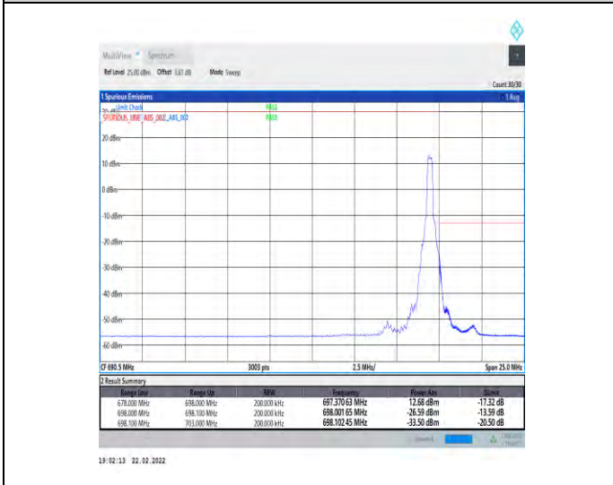
1-N71-15-20-H-5-CP-QPSK-Edge_1RB_Right-1@105-Ant1-PASS-see graph
