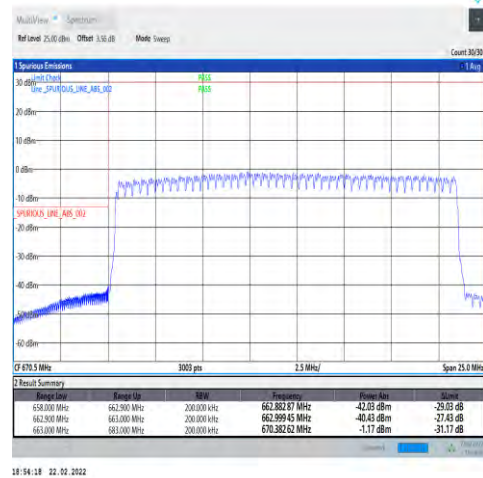
1-N71-15-20-L-3-DFT-PI2BPSK-Outer_Full-100@0-Ant1-PASS-see graph
