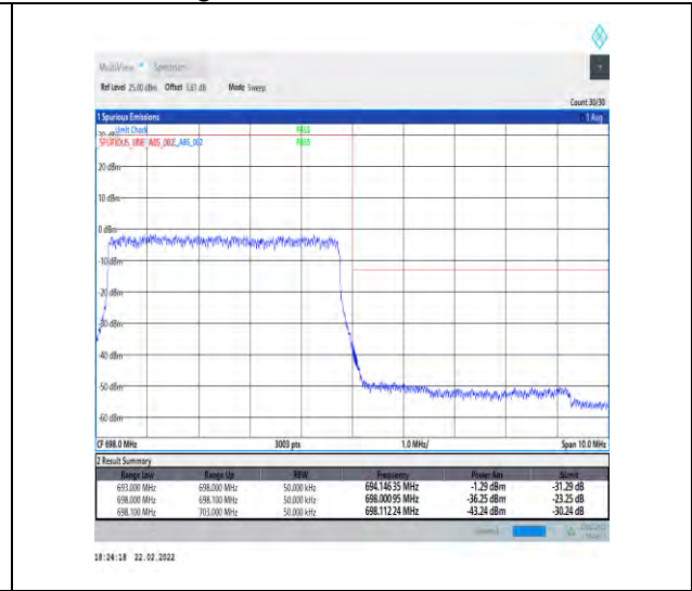
1-N71-15-5-H-3-DFT-PI2BPSK-Outer_Full-25@0-Ant1-PASS-see graph
