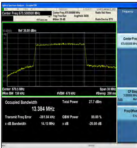
1-N71-15-15-L-5-DFT-256QAM-Outer_Full-75@0-Ant t1-13.384-14.13-≤15-PASS
