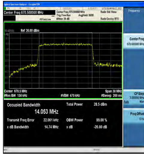
1-N71-15-15-L-8-CP-64QAM-Outer_Full-79@0-Ant1 -14.053-14.74-≤15-PASS
