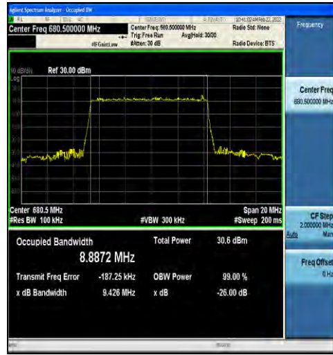
1-N71-15-10-M-2-DFT-PI2BPSK-Outer_Full-50@0-Ant1 -8.8872-9.426≤10-PASS
