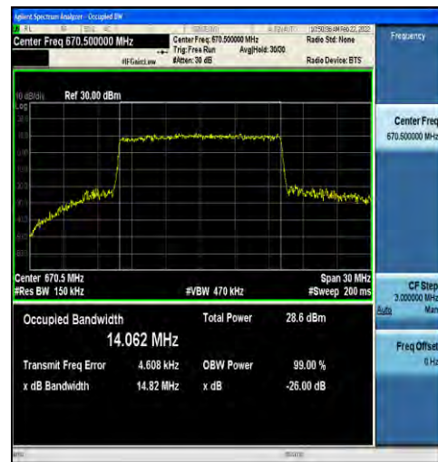
1-N71-15-15-L-6-CP-QPSK-Outer_Full-79@0-Ant1-1 4.062-14.82-≤15-PASS
