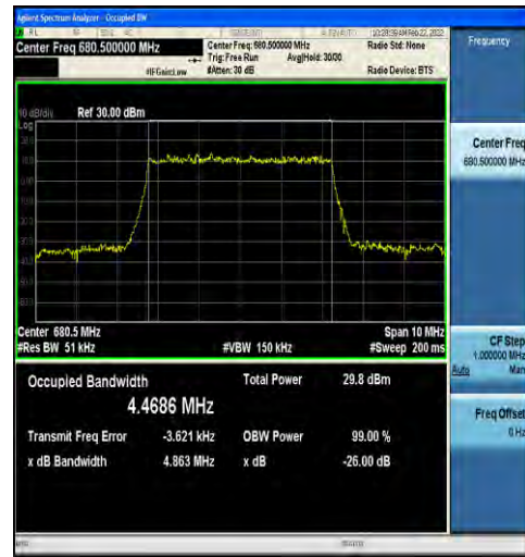
1-N71-15-5-M-1-DFT-QPSK-Outer_Full-25@0-Ant1- 4.4686-4.863-≤5-PASS
