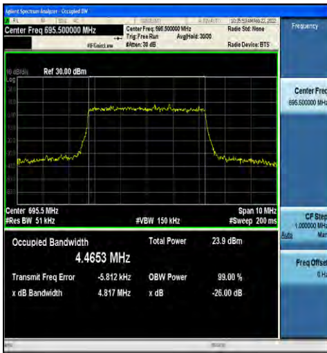
1-N71-15-5-H-9-CP-256QAM-Outer_Full-25@0-Ant1-4.4653-4.817-≤5-PASS
