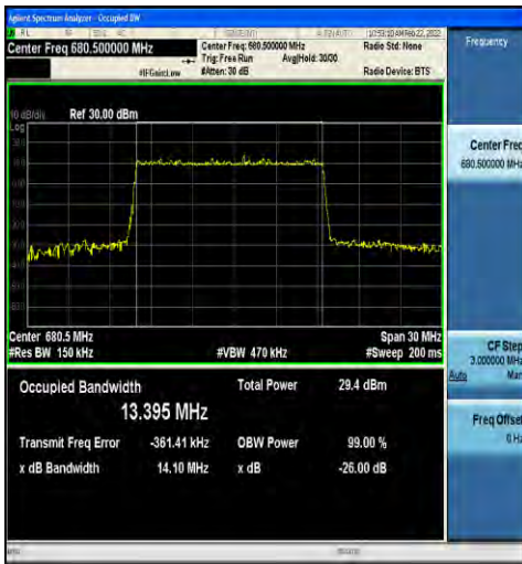
1-N71-15-15-M-4-DFT-64QAM-Outer_Full-75@0-Ant 1-13.395-14.10-≤15-PASS
