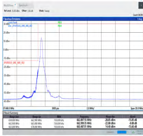
1-N71-15-15-L-4-CP-QPSK-Edge_1RB_Left-1@0-Ant1-PASS-see graph
