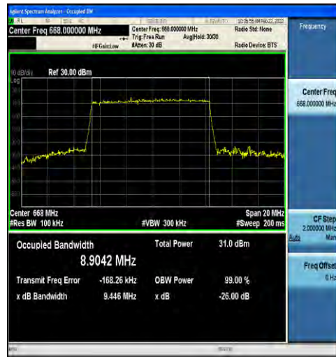
1-N71-15-10-L-1-DFT-QPSK-Outer_Full-50@0-Ant1-8.9042-9.446-≤10-PASS
