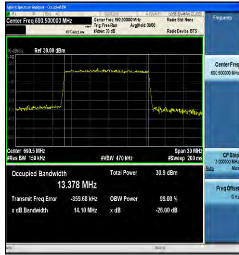
1-N71-15-15-H-2-DFT-PI2BPSK-Outer_Full-75@0-Ant1 -13.378-14.10≤15-PASS
