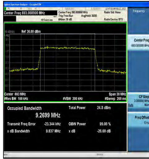
1-N71-15-10-H-9-CP-256QAM-Outer_Full-52@0-Ant1 1-9.2699-9.837-≤10-PASS
