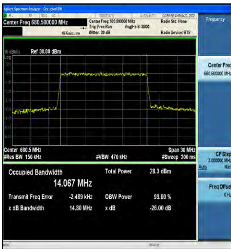
1-N71-15-15-M-8-CP-64QAM-Outer_Full-79@0-Ant 1-14.067-14.80-≤15-PASS
