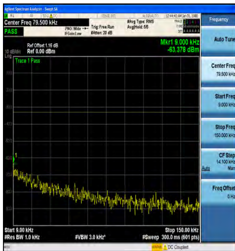
1-N71-15-20-M-1-DFT-PI2BPSK-Inner_1RB_Left-1 @1-0.009-0.15-Ant1--63.38--33-PASS
