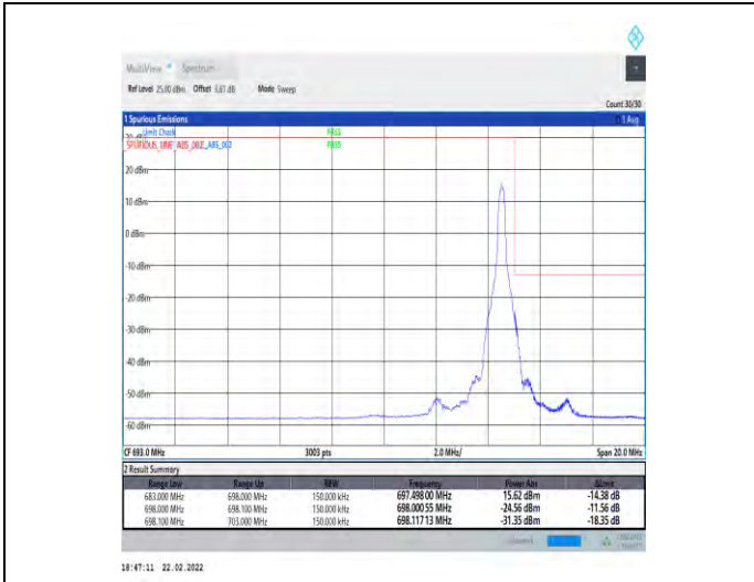
1-N71-15-15-H-2-DFT-P12BPSK-Edge_1RB_Right-1@78-Ant1-PASS-see graph
