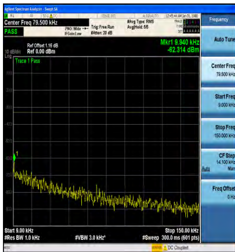
1-N71-15-20-H-1-DFT-PI2BPSK-Inner_1RB_Left-1 @1-0.009-0.15-Ant1--62.31--33-PASS
