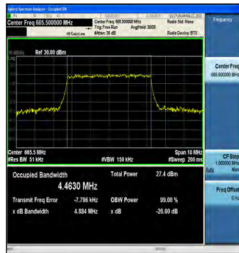
1-N71-15-5-L-8-CP-64QAM-Outer_Full-25@0-Ant1-4 .4630-4.884-≤5-PASS
