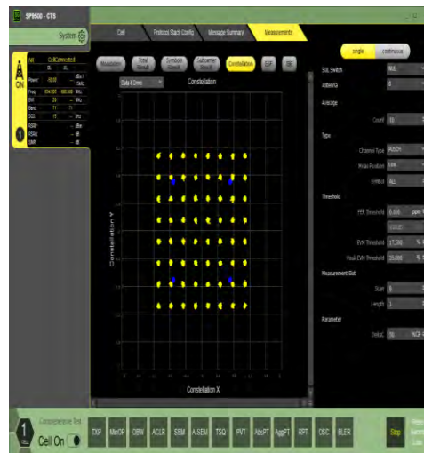
1-N71-15-20-M-8-CP-64QAM-Outer_Full-106@0-Ant1-see graph-PASS
