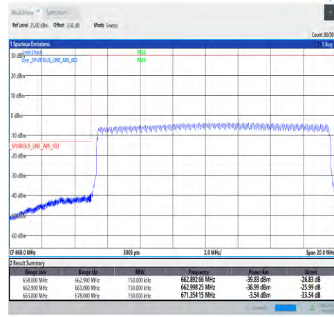
1-N71-15-15-L-6-CP-QPSK-Outer_Full-79@0-Ant1-PASS-see graph
