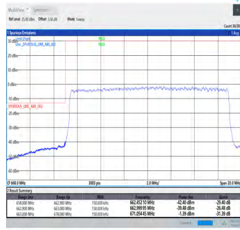
1-N71-15-15-L-3-DFT-PI2BPSK-Outer_Full-75@0-Ant1-PASS-see graph
