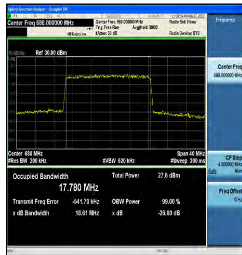
1-N71-15-20-H-5-DFT-256QAM-Outer_Full-100@0-Ant1-17.780-18.61-≤20-PASS
