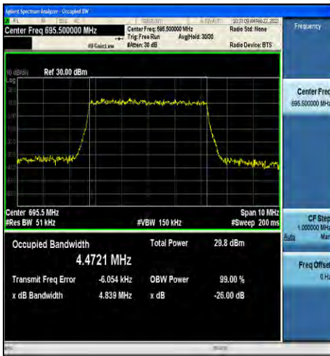
1-N71-15-5-H-1-DFT-QPSK-Outer_Full-25@0-Ant1-4.4721-4.839-≤5-PASS
