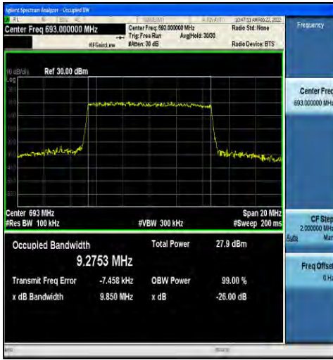
1-N71-15-10-H-8-CP-64QAM-Outer_Full-52@0-Ant1 -9.2753-9.850-≤10-PASS
