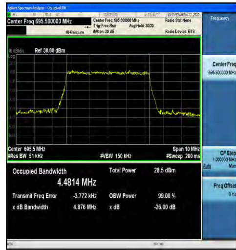
1-N71-15-5-H-4-DFT-64QAM-Outer_Full-25@0-Ant1 -4.4814-4.876-≤5-PASS
