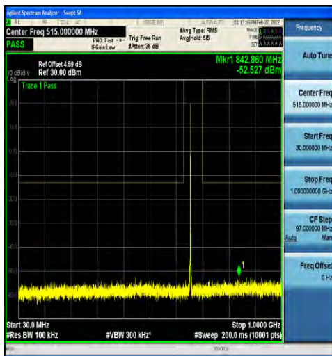
1-N71-15-20-L-1-DFT-PI2BPSK-Inner_1RB_Left-1@ 1-30-1000-Ant1--52.53--13-PASS
