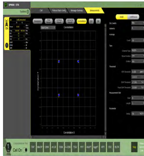
1-N71-15-20-M-6-CP-QPSK-Outer_Full-106@0-Ant1-see graph-PASS
