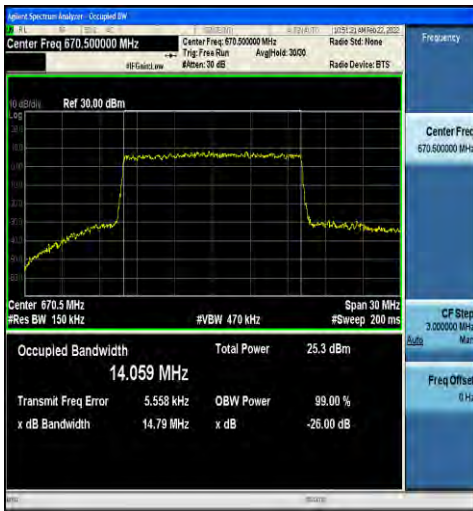
1-N71-15-15-L-9-CP-256QAM-Outer_Full-79@0-Ant 1-14.059-14.79-≤15-PASS
