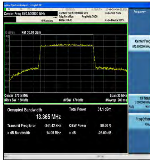
1-N71-15-15-L-2-DFT-PI2BPSK-Outer_Full-75@0-A nt1-13.365-14.09-≤15-PASS
