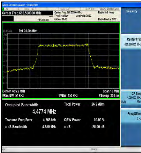
1-N71-15-5-L-5-DFT-256QAM-Outer_Full-25@0-Ant 1-4.4774-4.850-≤5-PASS
