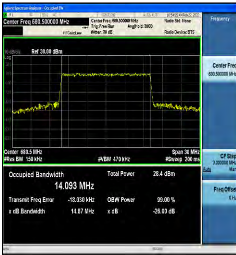
1-N71-15-15-M-6-CP-QPSK-Outer_Full-79@0-Ant1-14.093-14.87-≤15-PASS
