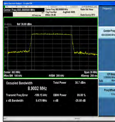
1-N71-15-10-H-1-DFT-QPSK-Outer_Full-50@0-Ant1-8.9002-9.470-≤10-PASS
