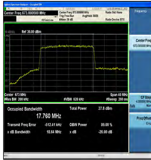
1-N71-15-20-L-5-DFT-256QAM-Outer_Full-100@0-A nt1-17.760-18.64-≤20-PASS
