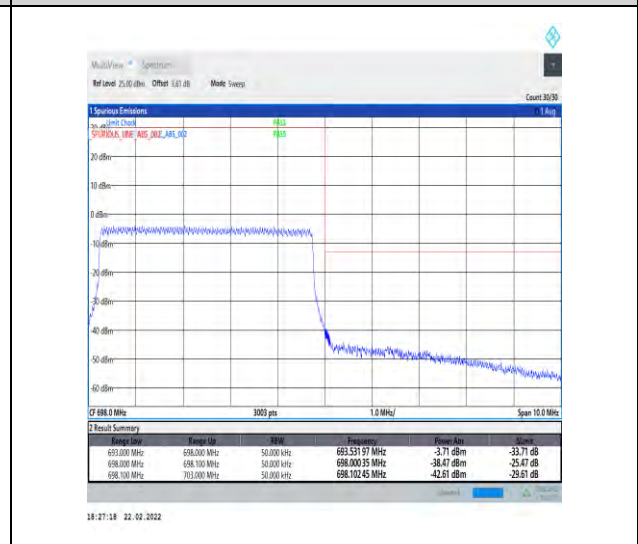
1-N71-15-5-H-6-CP-QPSK-Outer_Full-25@0-Ant1-PASS-see graph
