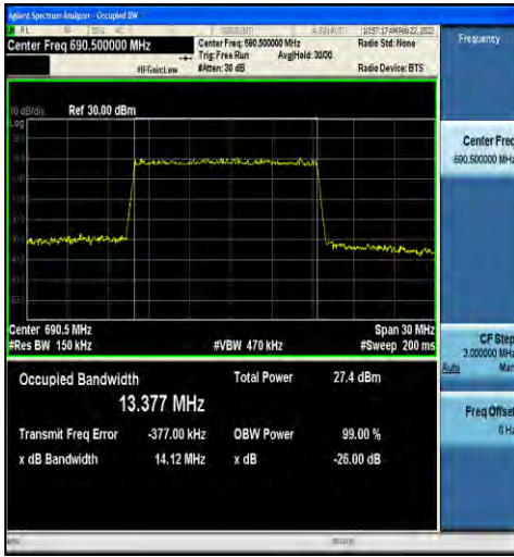
1-N71-15-15-H-5-DFT-256QAM-Outer_Full-75@0-A nt1-13.377-14.12-≤15-PASS
