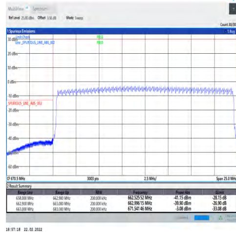
1-N71-15-20-L-6-CP-QPSK-Outer_Full-106@0-Ant1-PASS-see graph
