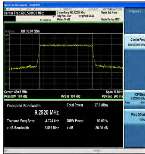
1-N71-15-10-M-8-CP-64QAM-Outer_Full-52@0-Ant1 -9.2920-9.857-≤10-PASS
