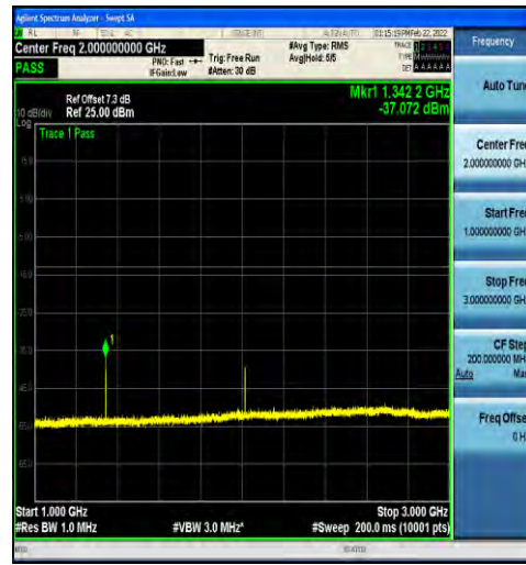
1-N71-15-20-M-1-DFT-PI2BPSK-Inner_1RB_Left-1@ 1-1000-3000-Ant1--37.07--13-PASS
