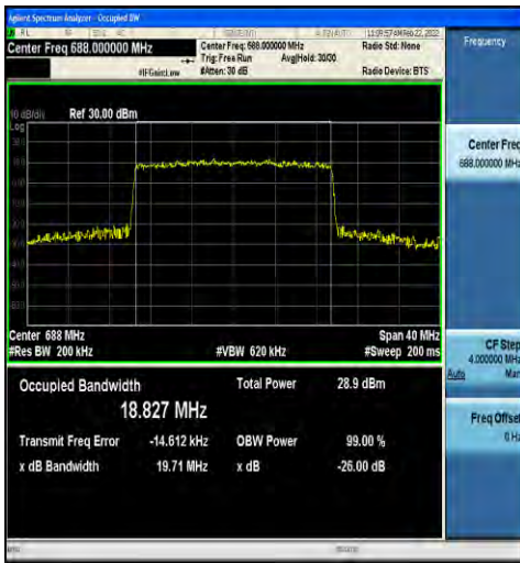
1-N71-15-20-H-6-CP-QPSK-Outer_Full-106@0-Ant1 -18.827-19.71-≤20-PASS
