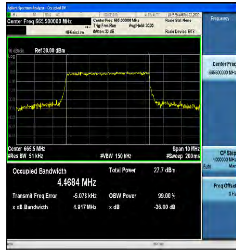
1-N71-15-5-L-6-CP-QPSK-Outer_Full-25@0-Ant1-4. 4684-4.917-≤5-PASS
