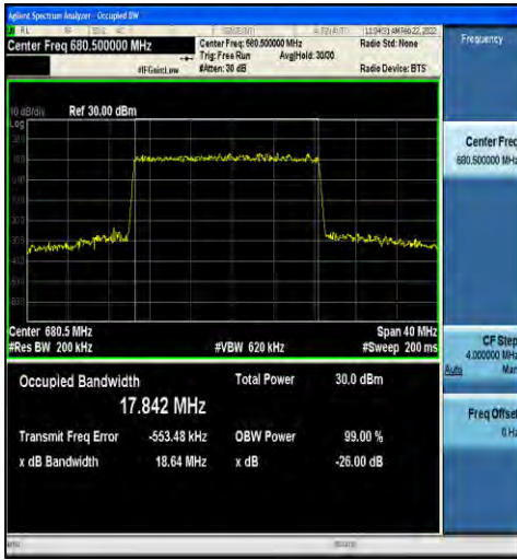
1-N71-15-20-M-3-DFT-16QAM-Outer_Full-100@0-A nt1-17.842-18.64-≤20-PASS
