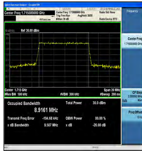
1-N66-15-10-L-3-DFT-16QAM-Outer_Full-50@0-Ant 1-8.9161-9.507-≤10-PASS
