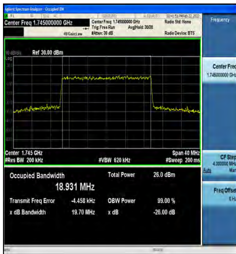
1-N66-15-20-M-9-CP-256QAM-Outer_Full-106@0-Ant nt1-18.931-19.70-≤20-PASS
