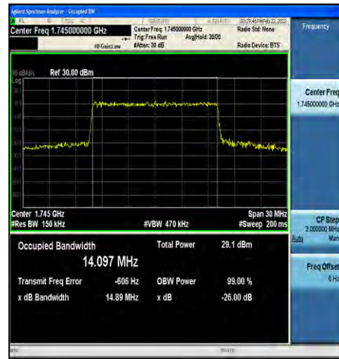
1-N66-15-15-M-7-CP-16QAM-Outer_Full-79@0-Ant1 -14.097-14.89-≤15-PASS
