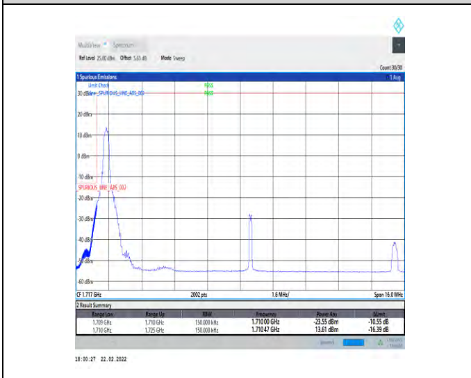
1-N66-15-15-L-4-CP-QPSK-Edge_1RB_Left-1@0-Ant1-seegraph-PASS-see graph
