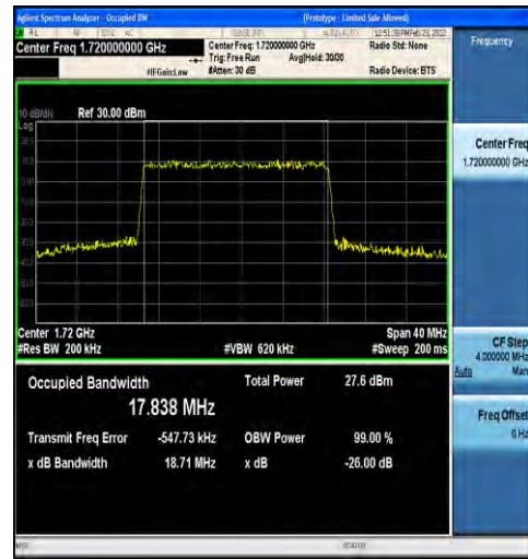
1-N66-15-20-L-5-DFT-256QAM-Outer_Full-100@0-A nt1-17.838-18.71- \leq 20 -PASS
