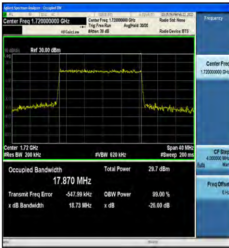
1-N66-15-20-L-4-DFT-64QAM-Outer_Full-100@0-An t1-17.870-18.73- \leq 20 -PASS
