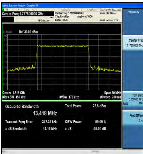
1-N66-15-15-L-5-DFT-256QAM-Outer_Full-75@0-Ant t1-13.418-14.16-≤15-PASS
