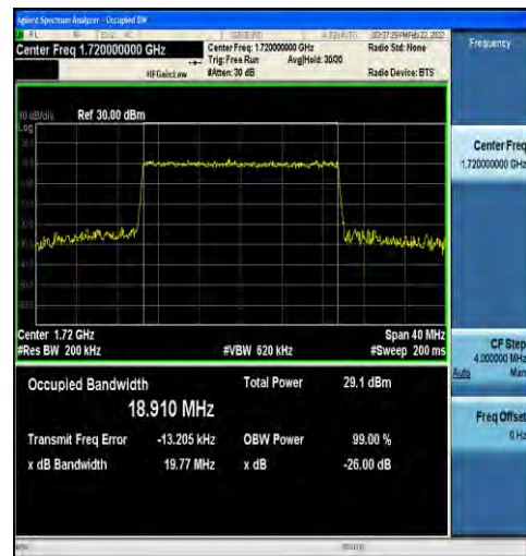
1-N66-15-20-L-7-CP-16QAM-Outer_Full-106@0-Ant 1-18.910-19.77- \leq 20 -PASS
