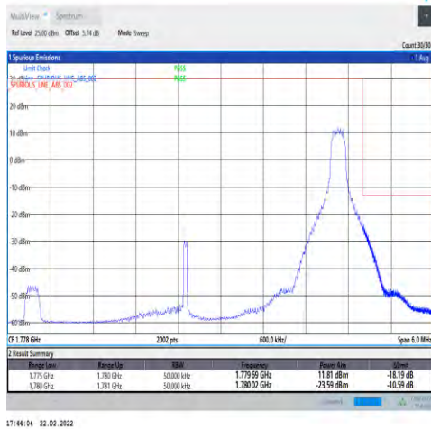
1-N66-15-5-H-2-DFT-PI2BPSK-Edge_1RB_Right-1@2 4-Ant1-seegraph-PASS-see graph
