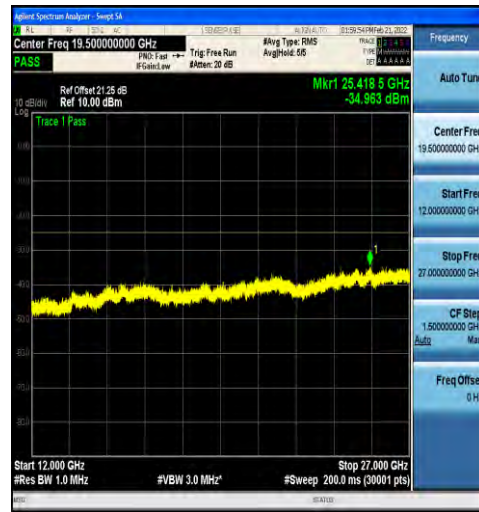
1-N41-30-100-H-1-DFT-PI2BPSK-Inner_1RB_Left-1 @1-12000-27000-Ant1--34.96--25-PASS
