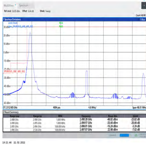
1-N41-30-40-L-1-DFT-PI2BPSK-Edge_1RB_Left-1@0-Ant1-PASS-see graph
