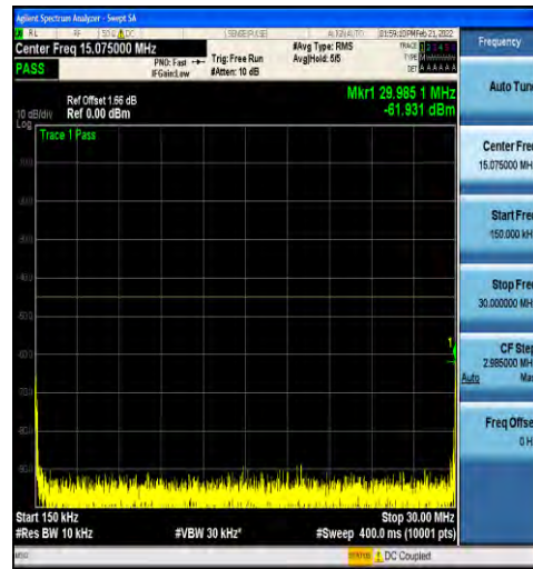
1-N41-30-100-H-1-DFT-PI2BPSK-Inner_1RB_Left-1 @1-0.15-30-Ant1--61.93--45-PASS
