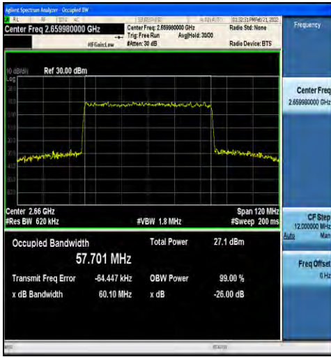
1-N41-30-60-H-9-CP-256QAM-Outer_Full-162@0-A nt1-57.701-60.10-≤60-PASS
