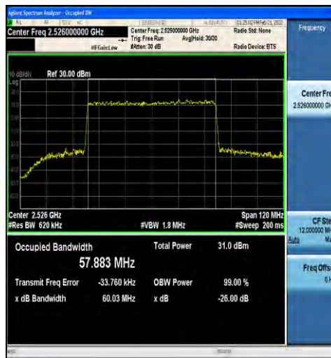
1-N41-30-60-L-8-CP-64QAM-Outer_Full-162@0-Ant 1-57.883-60.03-≤60-PASS
