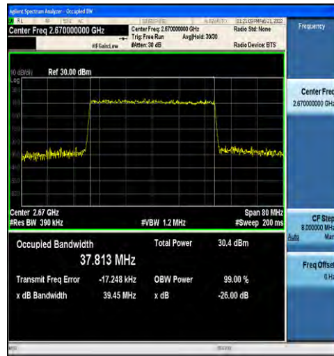
1-N41-30-40-H-7-CP-16QAM-Outer_Full-106@0-Ant1 1-37.813-39.45-≤40-PASS
