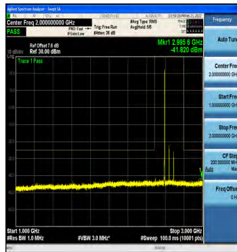
1-N41-30-100-H-1-DFT-PI2BPSK-Inner_1RB_Left-1 @1-1000-3000-Ant1--41.82--25-PASS
