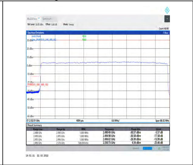
1-N41-30-80-L-3-DFT-PI2BPSK-Outer_Full-216@0-Ant1-PASS-see graph
