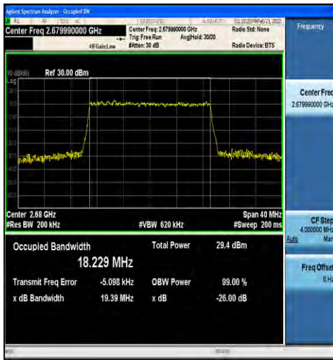
1-N41-30-20-H-7-CP-16QAM-Outer_Full-51@0-Ant1 -18.229-19.39-≤20-PASS
