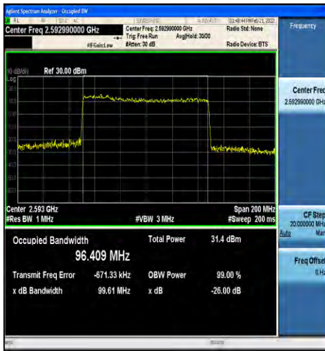
1-N41-30-100-M-4-DFT-64QAM-Outer_Full-270@0-Ant1-96.409-99.61-≤100-PASS
