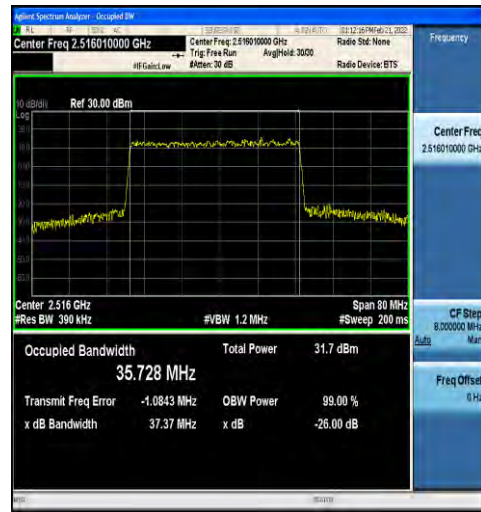
1-N41-30-40-L-3-DFT-16QAM-Outer_Full-100@0-Ant1-35.728-37.37-≤40-PASS
