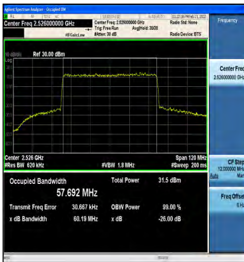
1-N41-30-60-L-1-DFT-QPSK-Outer_Full-162@0-Ant 1-57.692-60.19-≤60-PASS
