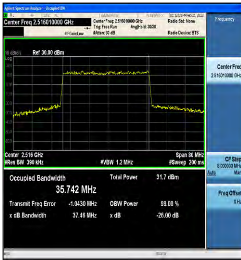
1-N41-30-40-L-2-DFT-PI2BPSK-Outer_Full-100@0-Ant1-35.742-37.46-≤40-PASS
