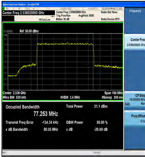
1-N41-30-80-L-8-CP-64QAM-Outer_Full-217@0-Ant 1-77.253-80.05-≤80-PASS
