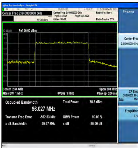
1-N41-30-100-H-1-DFT-QPSK-Outer_Full-270@0-A t1-96.027-99.67-≤100-PASS
