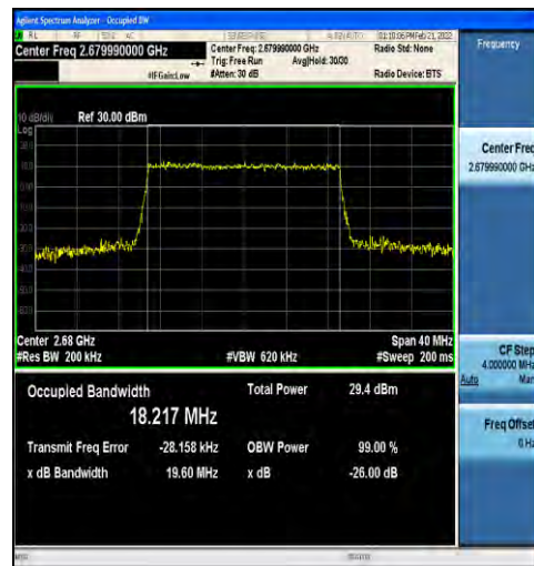
1-N41-30-20-H-6-CP-QPSK-Outer_Full-51@0-Ant1 18.217-19.60-≤20-PASS
