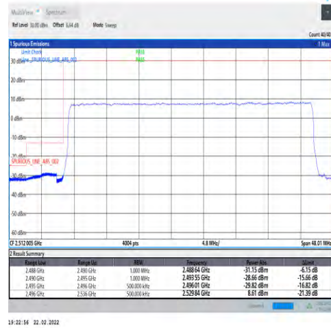
1-N41-30-40-L-3-DFT-PI2BPSK-Outer_Full-100@0-Ant1-PASS-see graph
