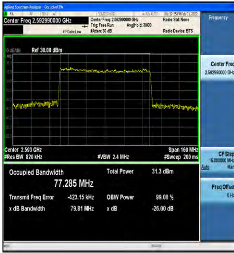
1-N41-30-80-M-3-DFT-16QAM-Outer_Full-216@0-A nt1-77.285-79.81-≤80-PASS
