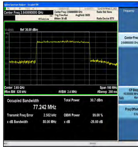
1-N41-30-80-H-7-CP-16QAM-Outer_Full-217@0-Ant1 1-77.242-80.06-≤80-PASS
