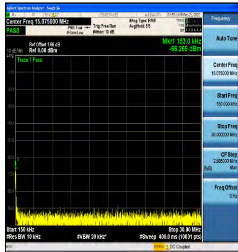
1-N41-30-100-M-1-DFT-PI2BPSK-Inner_1RB_Left-1 @1-0.15-30-Ant1--66.27--45-PASS
