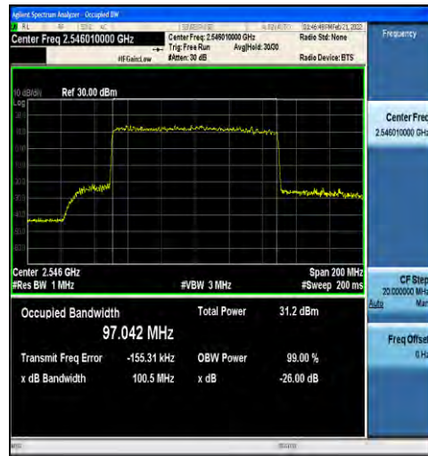
1-N41-30-100-L-8-CP-64QAM-Outer_Full-273@0-Ant 1-97.042-100.5-≤100-PASS
