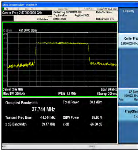
1-N41-30-40-H-8-CP-64QAM-Outer_Full-106@0-Ant 1-37.744-39.47-≤40-PASS
