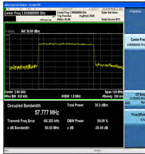
1-N41-30-60-H-4-DFT-64QAM-Outer_Full-162@0-Ant 1-57.777-60.05-≤60-PASS
