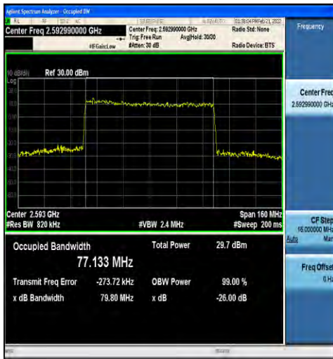
1-N41-30-80-M-5-DFT-256QAM-Outer_Full-216@0-A Ant1-77.133-79.80-≤80-PASS
