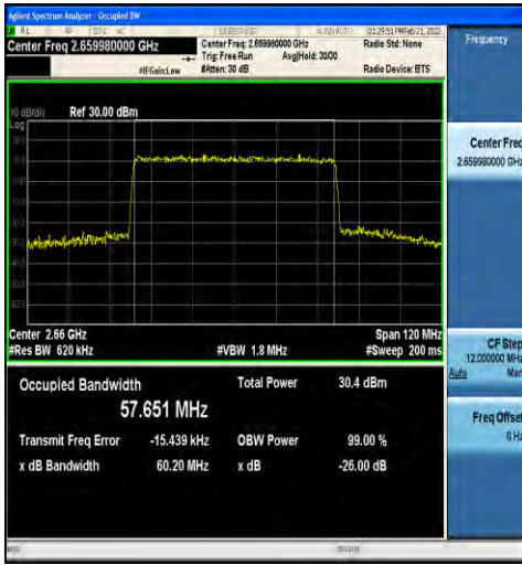
1-N41-30-60-H-1-DFT-QPSK-Outer_Full-162@0-Ant 1-57.651-60.20-≤60-PASS
