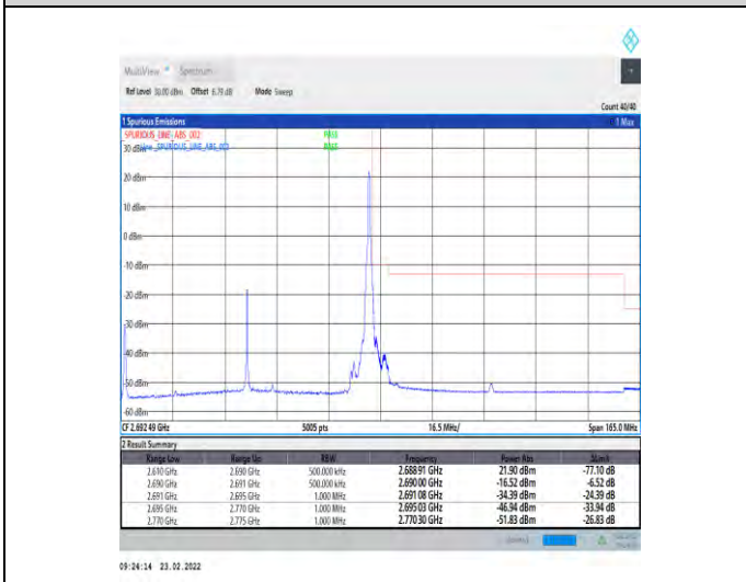
1-N41-30-80-H-5-CP-QPSK-Edge_1RB_Right-1@216-Ant1-PASS-see graph
