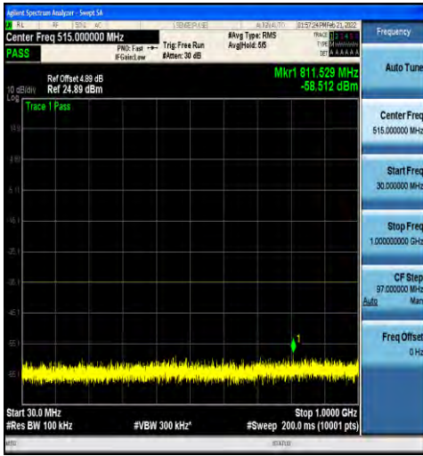
1-N41-30-100-M-1-DFT-PI2BPSK-Inner_1RB_Left-1 @1-30-1000-Ant1--58.51--35-PASS
