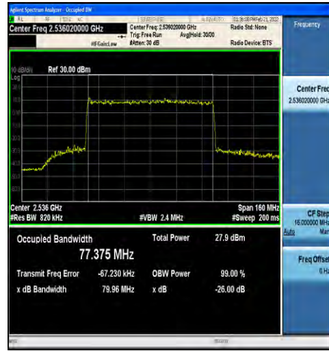
1-N41-30-80-L-9-CP-256QAM-Outer_Full-217@0-A nt1-77.375-79.96-≤80-PASS
