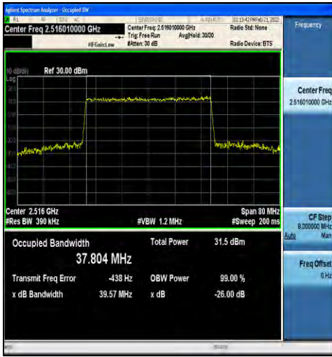
1-N41-30-40-L-6-CP-QPSK-Outer_Full-106@0-Ant1- 37.804-39.57-≤40-PASS
