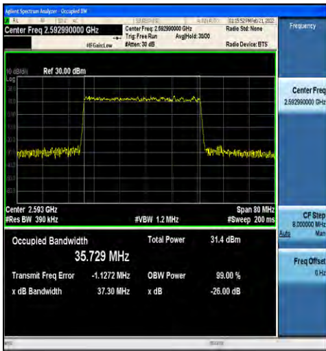
1-N41-30-40-M-3-DFT-16QAM-Outer_Full-100@0-A nt1-35.729-37.30-≤40-PASS
