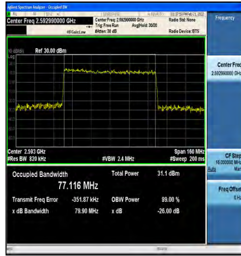
1-N41-30-80-M-4-DFT-64QAM-Outer_Full-216@0-A nt1-77.116-79.90-≤80-PASS
