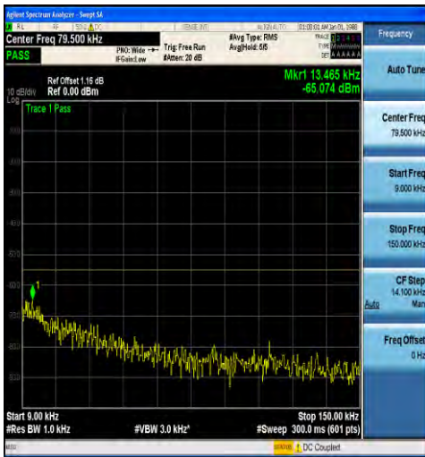
1-N41-30-100-M-1-DFT-PI2BPSK-Inner_1RB_Left-1 @1-0.009-0.15-Ant1--65.07--55-PASS
