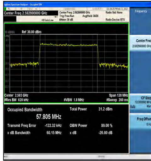
1-N41-30-60-M-7-CP-16QAM-Outer_Full-162@0-Ant1 -57.805-60.15-≤60-PASS
