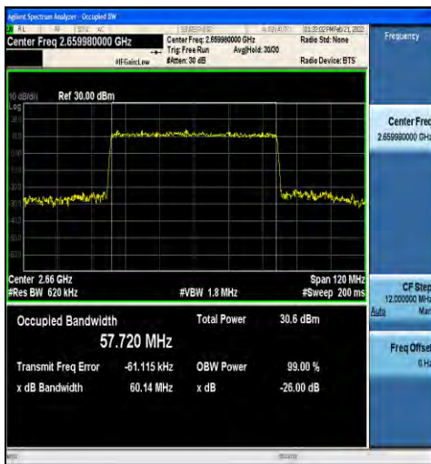
1-N41-30-60-H-7-CP-16QAM-Outer_Full-162@0-Ant 1-57.720-60.14-≤60-PASS
