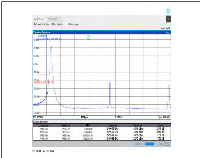
1-N41-30-60-L-1-DFT-PI2BPSK-Edge_1RB_Left-1@0-Ant1-PASS-see graph
