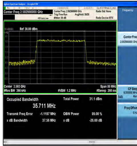
1-N41-30-40-M-2-DFT-PI2BPSK-Outer_Full-100@0-Ant 1-35.711-37.56-≤40-PASS
