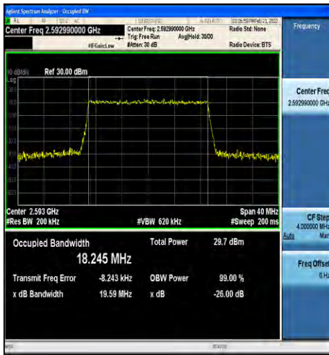
1-N41-30-20-M-8-CP-64QAM-Outer_Full-51@0-Ant1 -18.245-19.59-≤20-PASS
