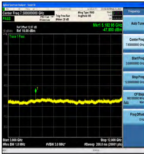
1-N41-30-100-H-1-DFT-PI2BPSK-Inner_1RB_Left-1 @1-3000-12000-Ant1--47.85--25-PASS
