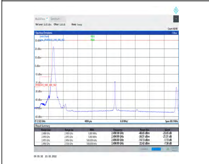
1-N41-30-60-L-4-CP-QPSK-Edge_1RB_Left-1@0-Ant1-PASS-see graph
