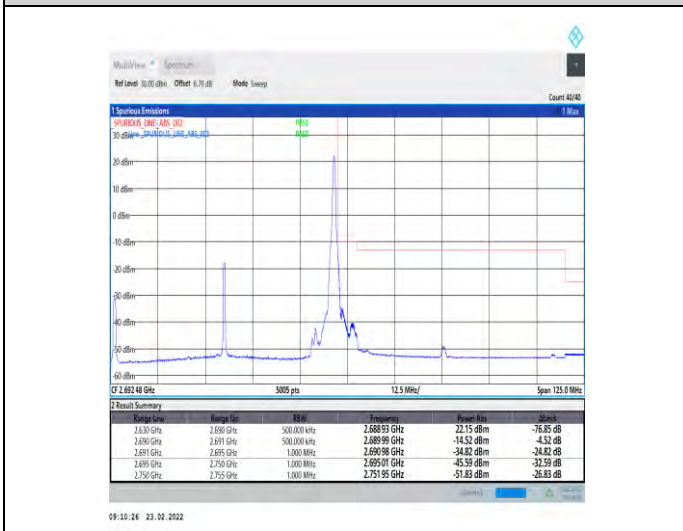
1-N41-30-60-H-5-CP-QPSK-Edge_1RB_Right-1@161-Ant1-PASS-see graph
