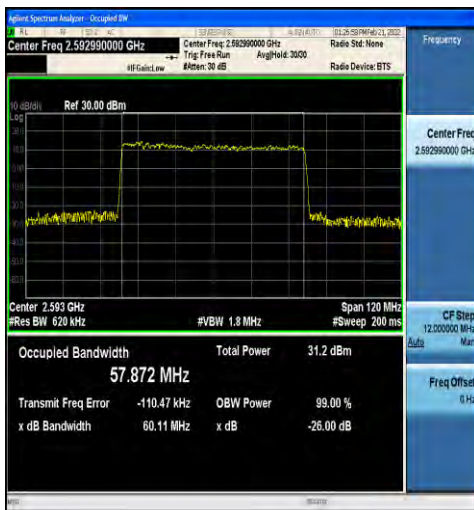
1-N41-30-60-M-4-DFT-64QAM-Outer_Full-162@0-Ant1-57.872-60.11-≤60-PASS
