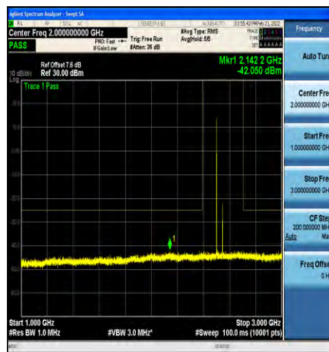
1-N41-30-100-L-1-DFT-PI2BPSK-Inner_1RB_Left-1 @1-1000-3000-Ant1--41.84--25-PASS
