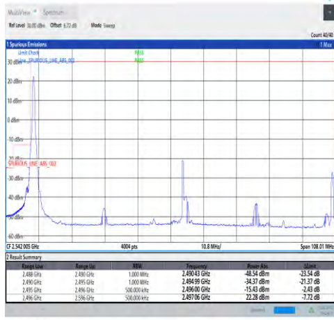
1-N41-30-100-L-1-DFT-PI2BPSK-Edge_1RB_Left-1@0-Ant1-PASS-see graph
