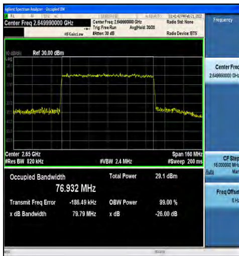
1-N41-30-80-H-5-DFT-256QAM-Outer_Full-216@0-Ant1-76.932-79.79-≤80-PASS
