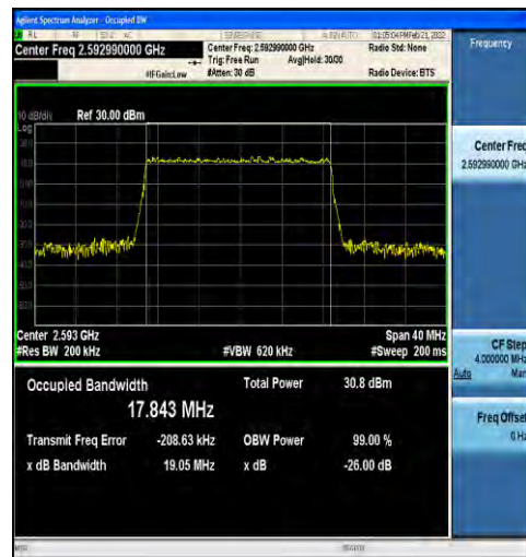
1-N41-30-20-M-3-DFT-16QAM-Outer_Full-50@0-Ant 1-17.843-19.05-≤20-PASS
