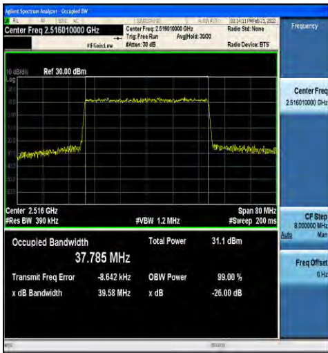
1-N41-30-40-L-8-CP-64QAM-Outer_Full-106@0-Ant1- 37.785-39.58-≤40-PASS
