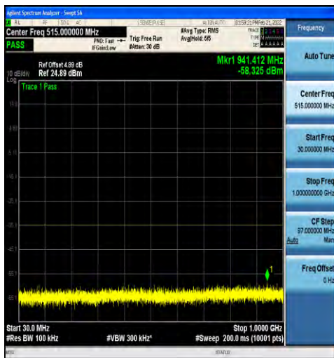
1-N41-30-100-H-1-DFT-PI2BPSK-Inner_1RB_Left-1 @1-30-1000-Ant1--58.32--35-PASS
