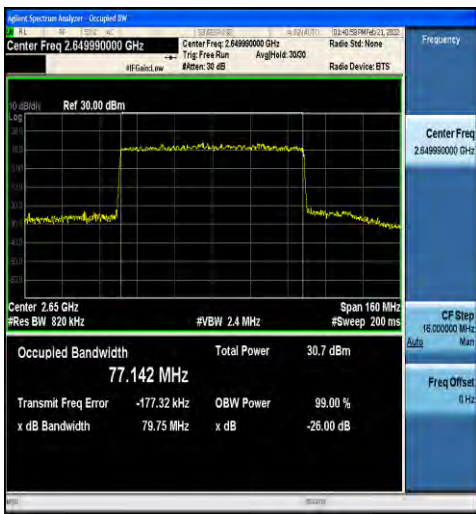
1-N41-30-80-H-2-DFT-P12BPSK-Outer_Full-216@0-Ant1-77.142-79.75-≤80-PASS
