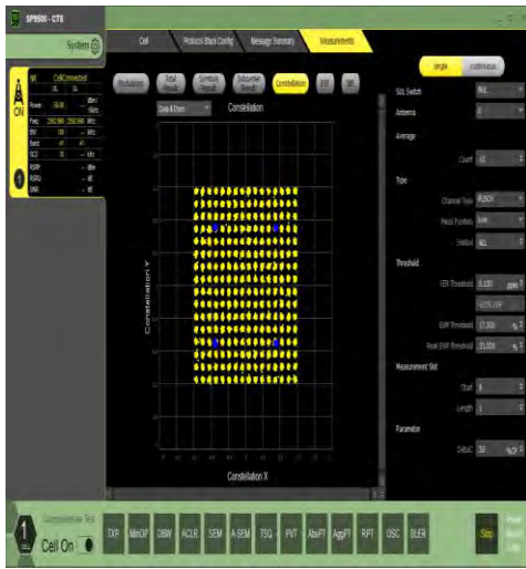
1-N41-30-100-M-9-CP-256QAM-Outer_Full-273@0-A nt1-see graph-PASS
