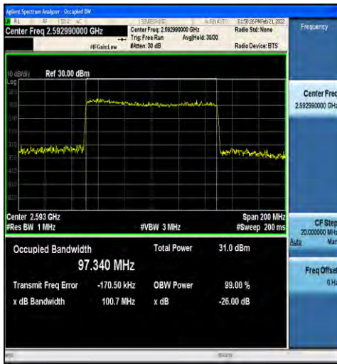
1-N41-30-100-M-8-CP-64QAM-Outer_Full-273@0-A nt1-97.340-100.7-≤100-PASS
