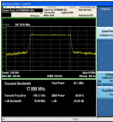
1-N41-30-20-H-3-DFT-16QAM-Outer_Full-50@0-Ant 1-17.898-18.99-≤20-PASS
