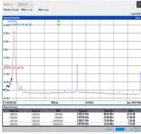
1-N41-30-100-L-4-CP-QPSK-Edge_1RB_Left-1@0-Ant1-PASS-see graph
