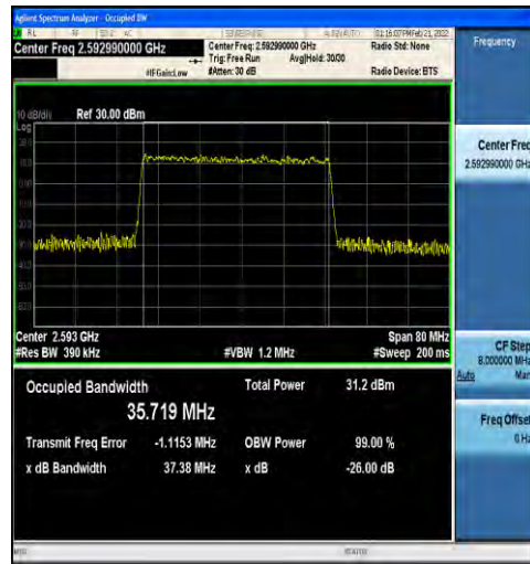
1-N41-30-40-M-4-DFT-64QAM-Outer_Full-100@0-A nt1-35.719-37.38-≤40-PASS
