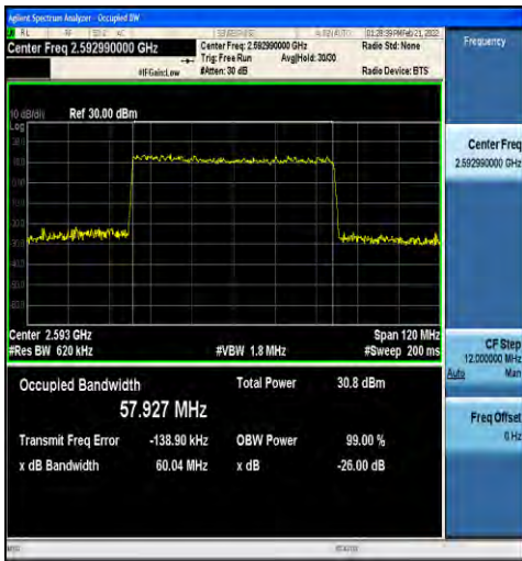
1-N41-30-60-M-8-CP-64QAM-Outer_Full-162@0-Ant1 -57.927-60.04-≤60-PASS
