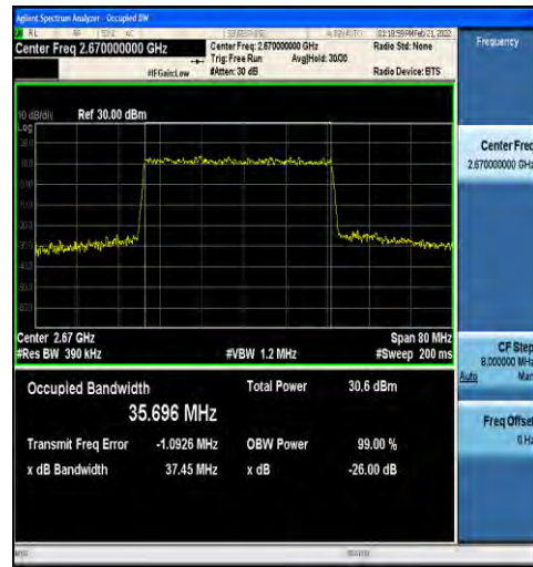
1-N41-30-40-H-1-DFT-QPSK-Outer_Full-100@0-Ant 1-35.696-37.45-≤40-PASS
