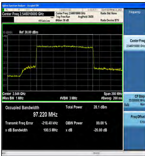
1-N41-30-100-L-9-CP-256QAM-Outer_Full-273@0-A nt1-97.220-100.5-≤100-PASS
