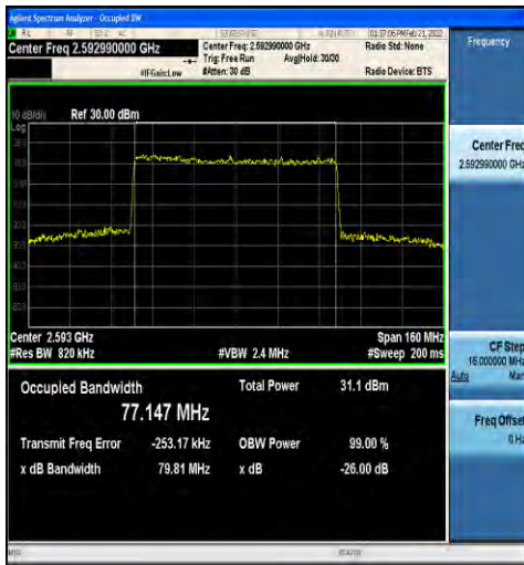
1-N41-30-80-M-1-DFT-QPSK-Outer_Full-216@0-Ant 1-77.147-79.81-≤80-PASS
