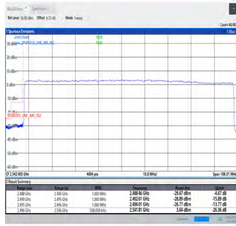
1-N41-30-100-L-3-DFT-PI2BPSK-Outer_Full-270@0-Ant1-PASS-see graph
