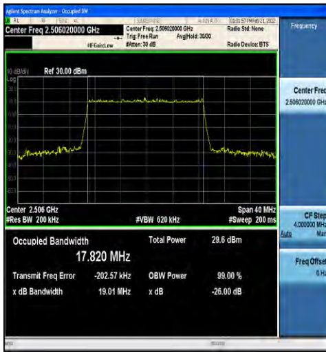
1-N41-30-20-L-5-DFT-256QAM-Outer_Full-50@0-Ant1-17.820-19.01-≤20-PASS
