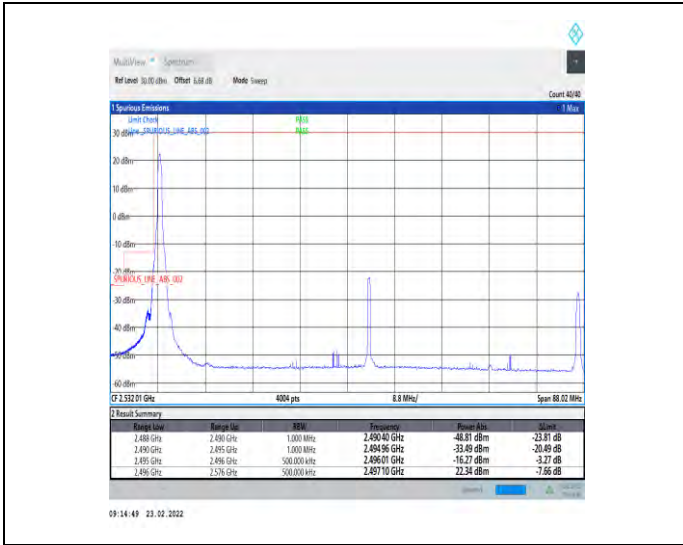
1-N41-30-80-L-1-DFT-PI2BPSK-Edge_1RB_Left-1@0-Ant1-PASS-see graph
