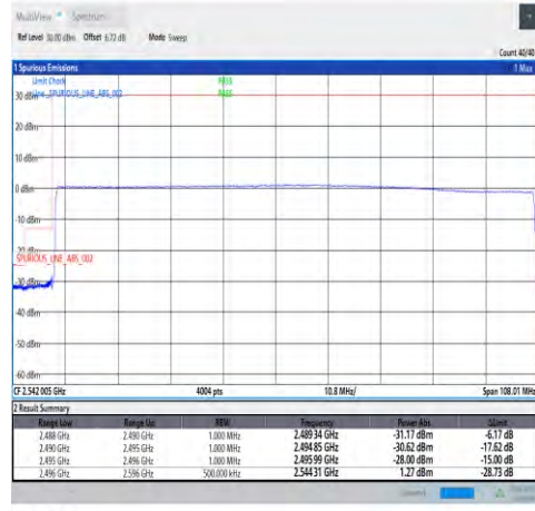
1-N41-30-100-L-6-CP-QPSK-Outer_Full-273@0-Ant1-PASS-see graph
