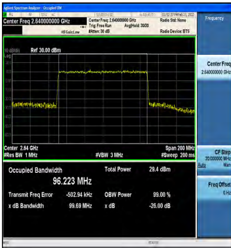
1-N41-30-100-H-5-DFT-256QAM-Outer_Full-270@0-Ant1-96.223-99.69-≤100-PASS
