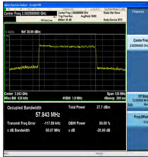
1-N41-30-60-M-9-CP-256QAM-Outer_Full-162@0-Ant1 -57.843-60.07-≤60-PASS
