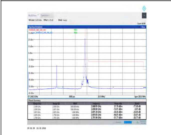
1-N41-30-100-H-5-CP-QPSK-Edge_1RB_Right-1@272 -Ant1-PASS-see graph
