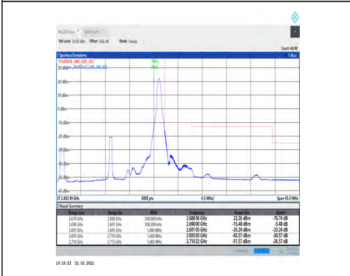
1-N41-30-20-H-5-CP-QPSK-Edge_1RB_Right-1@50-Ant1-PASS-see graph
