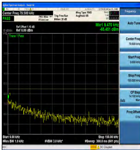
1-N41-30-100-L-1-DFT-PI2BPSK-Inner_1RB_Left-1 @1-0.009-0.15-Ant1--65.45--55-PASS
