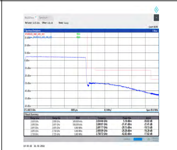
1-N41-30-40-H-6-CP-QPSK-Outer_Full-106@0-Ant1-PASS-see graph
