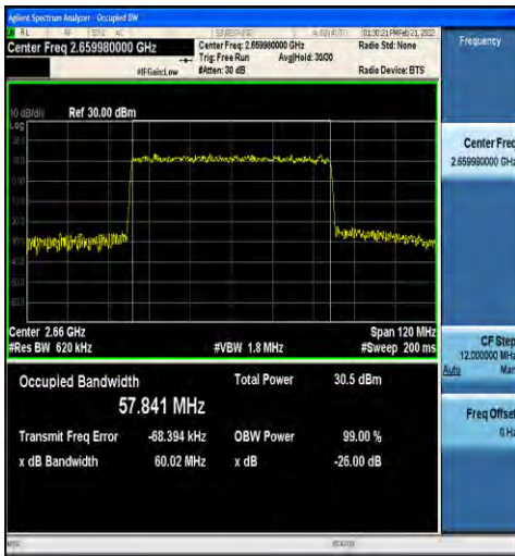
1-N41-30-60-H-3-DFT-16QAM-Outer_Full-162@0-Ant 1-57.841-60.02-≤60-PASS
