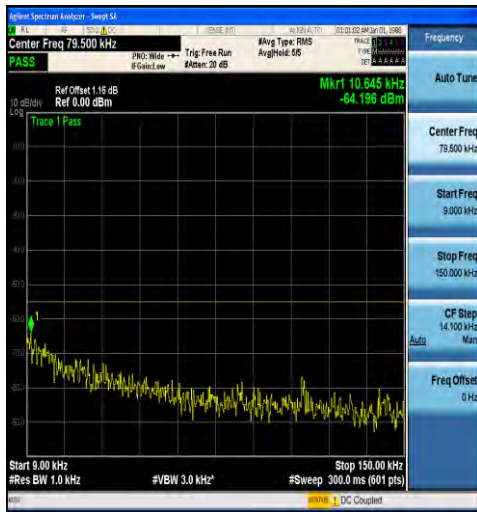
1-N41-30-100-H-1-DFT-PI2BPSK-Inner_1RB_Left-1 @1-0.009-0.15-Ant1--64.20--55-PASS
