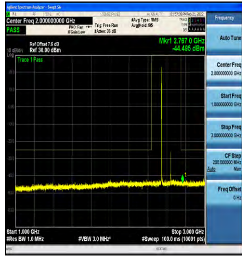
1-N41-30-100-M-1-DFT-PI2BPSK-Inner_1RB_Left-1 @1-1000-3000-Ant1--42.15--25-PASS
