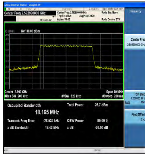
1-N41-30-20-M-9-CP-256QAM-Outer_Full-51@0-Ant1 t1-18.165-19.43-≤20-PASS
