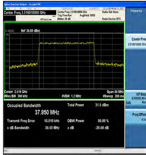
1-N41-30-40-L-7-CP-16QAM-Outer_Full-106@0-Ant1- 37.850-39.50-≤40-PASS
