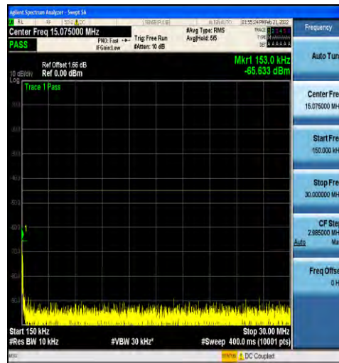
1-N41-30-100-L-1-DFT-PI2BPSK-Inner_1RB_Left-1 @1-0.15-30-Ant1--65.63--45-PASS
