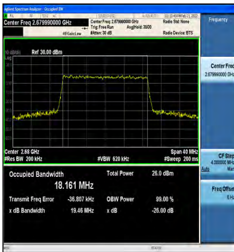
1-N41-30-20-H-9-CP-256QAM-Outer_Full-51@0-Ant 1-18.161-19.46-≤20-PASS
