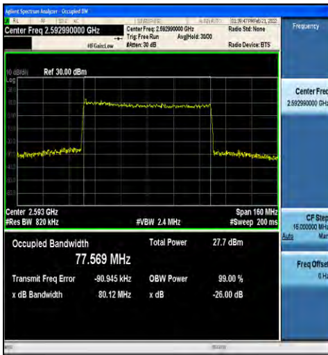
1-N41-30-80-M-9-CP-256QAM-Outer_Full-217@0-A nt1-77.569-80.12-≤80-PASS
