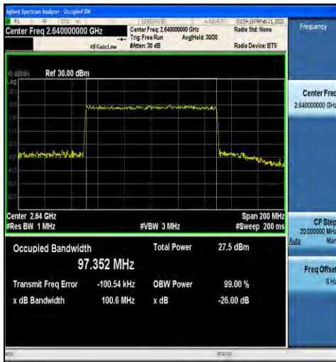
1-N41-30-100-H-9-CP-256QAM-Outer_Full-273@0- Ant1-97.352-100.6-≤100-PASS
