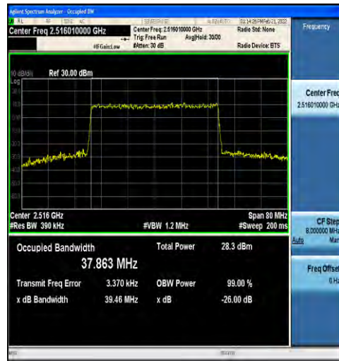
1-N41-30-40-L-9-CP-256QAM-Outer_Full-106@0-Ant1- 37.863-39.46-≤40-PASS
