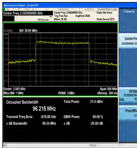
1-N41-30-100-M-1-DFT-QPSK-Outer_Full-270@0-A nt1-96.215-99.54-≤100-PASS
