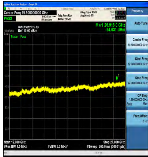
1-N41-30-100-L-1-DFT-PI2BPSK-Inner_1RB_Left-1 @1-12000-27000-Ant1--34.63--25-PASS
