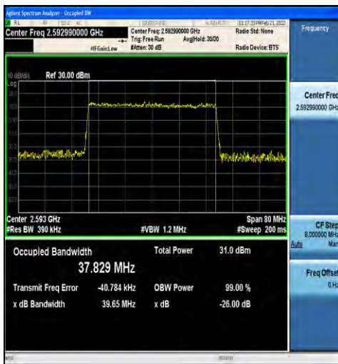
1-N41-30-40-M-7-CP-16QAM-Outer_Full-106@0-Ant1-37.829-39.65-≤40-PASS
