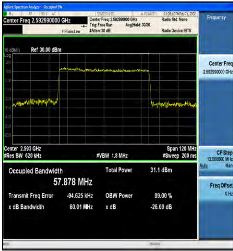
1-N41-30-60-M-6-CP-QPSK-Outer_Full-162@0-Ant1 -57.878-60.01-≤60-PASS
