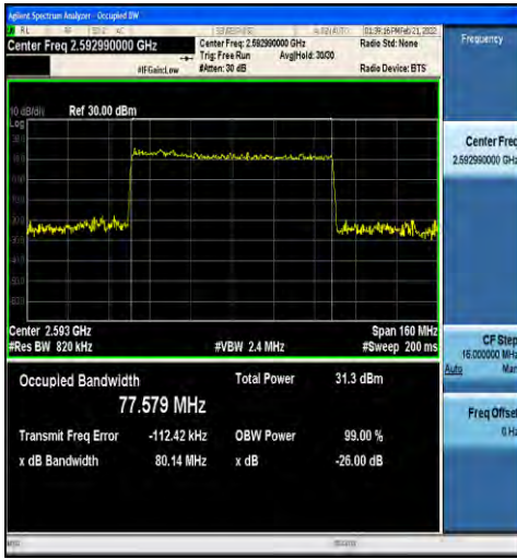
1-N41-30-80-M-7-CP-16QAM-Outer_Full-217@0-Ant 1-77.579-80.14-≤80-PASS
