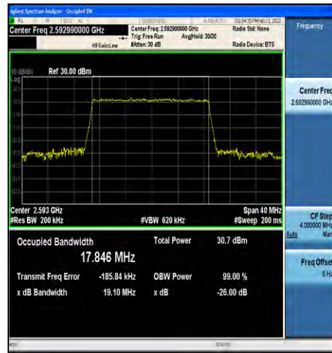
1-N41-30-20-M-1-DFT-QPSK-Outer_Full-50@0-Ant1 -17.846-19.10-≤20-PASS
