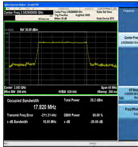
1-N41-30-20-M-5-DFT-256QAM-Outer_Full-50@0-A nt1-17.820-18.95-≤20-PASS
