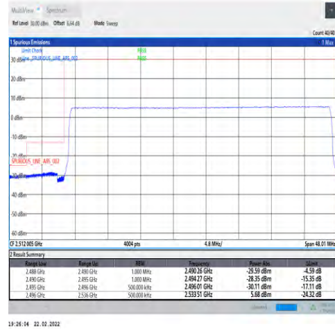
1-N41-30-40-L-6-CP-QPSK-Outer_Full-106@0-Ant1-PASS-see graph
