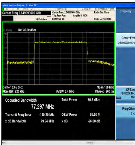
1-N41-30-80-H-8-CP-64QAM-Outer_Full-217@0-Ant1 1-77.297-79.94-≤80-PASS
