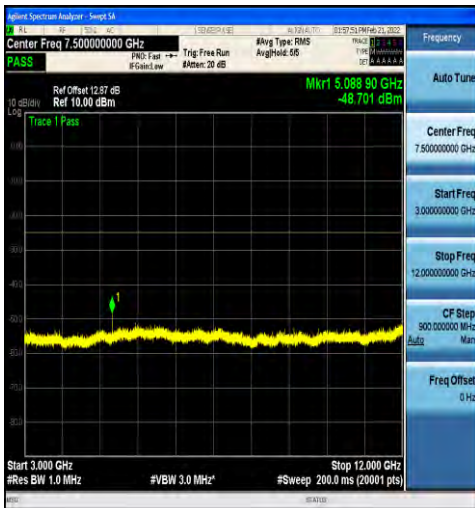
1-N41-30-100-M-1-DFT-PI2BPSK-Inner_1RB_Left-1 @1-3000-12000-Ant1--48.70--25-PASS
