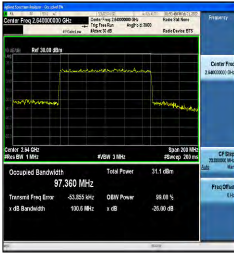
1-N41-30-100-H-7-CP-16QAM-Outer_Full-273@0-A nt1-97.360-100.6-≤100-PASS
