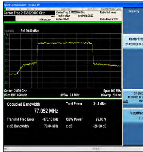
1-N41-30-80-L-3-DFT-16QAM-Outer_Full-216@0-Ant t1-77.052-79.84-≤80-PASS
