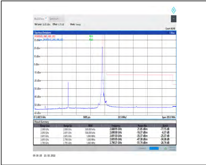
1-N41-30-100-H-2-DFT-PI2BPSK-Edge_1RB_Right-1 @272-Ant1-PASS-see graph
