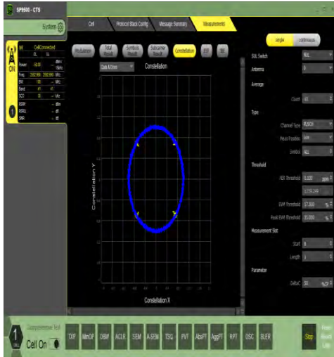
1-N41-30-100-M-1-DFT-PI2BPSK-Outer_Full-270@0-A Ant1-see graph-PASS
