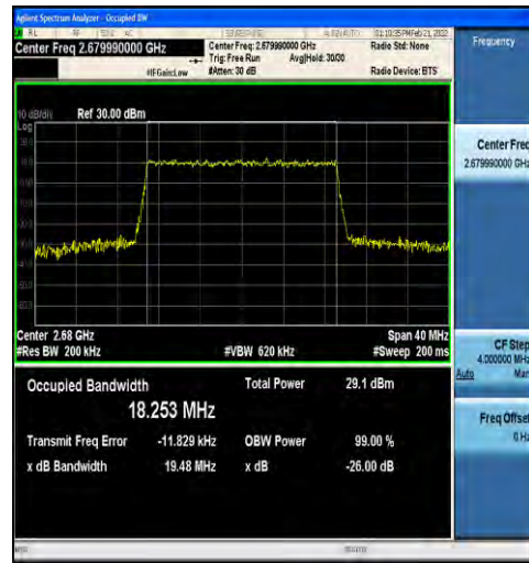
1-N41-30-20-H-8-CP-64QAM-Outer_Full-51@0-Ant1 -18.253-19.48-≤20-PASS
