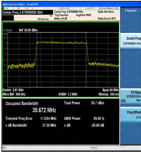
1-N41-30-40-H-4-DFT-64QAM-Outer_Full-100@0-A nt1-35.672-37.30-≤40-PASS
