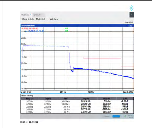
1-N41-30-20-H-6-CP-QPSK-Outer_Full-51@0-Ant1-PASS-see graph
