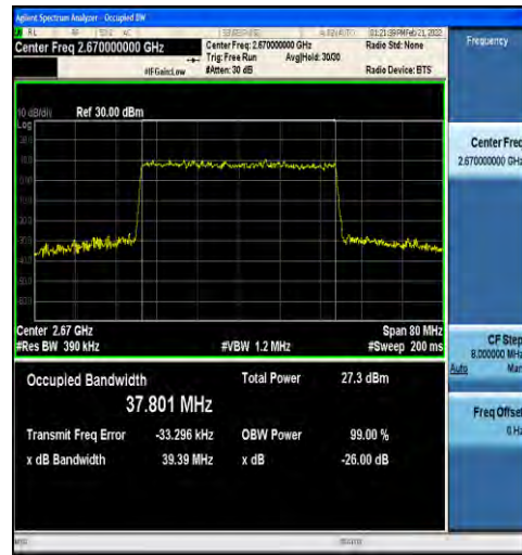
1-N41-30-40-H-9-CP-256QAM-Outer_Full-106@0-Ant nt1-37.801-39.39-≤40-PASS
