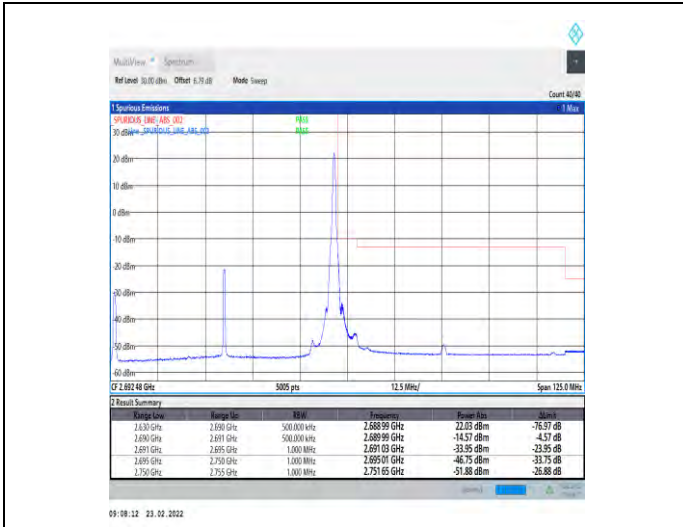
1-N41-30-60-H-2-DFT-PI2BPSK-Edge_1RB_Right-1@161-Ant1-PASS-see graph
