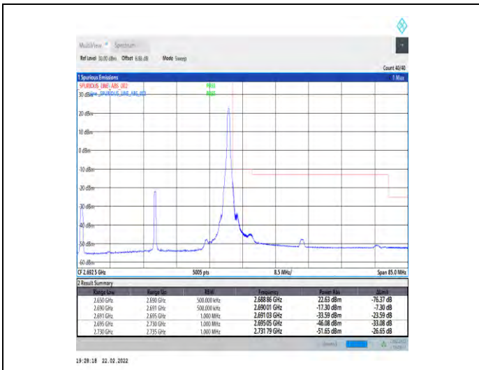
1-N41-30-40-H-2-DFT-PI2BPSK-Edge_1RB_Right-1@105-Ant1-PASS-see graph
