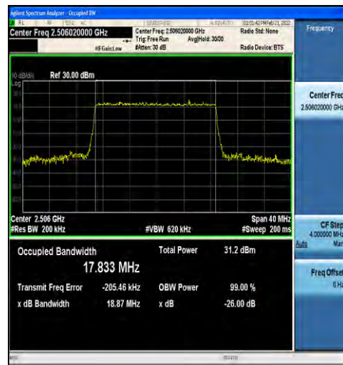
1-N41-30-20-L-4-DFT-64QAM-Outer_Full-50@0-Ant 1-17.833-18.87-≤20-PASS
