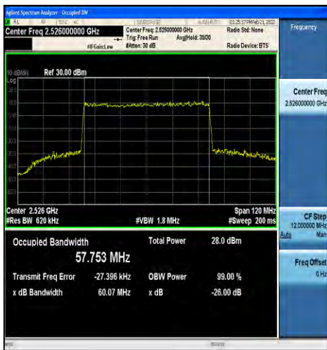
1-N41-30-60-L-9-CP-256QAM-Outer_Full-162@0-Ant t1-57.753-60.07-≤60-PASS
