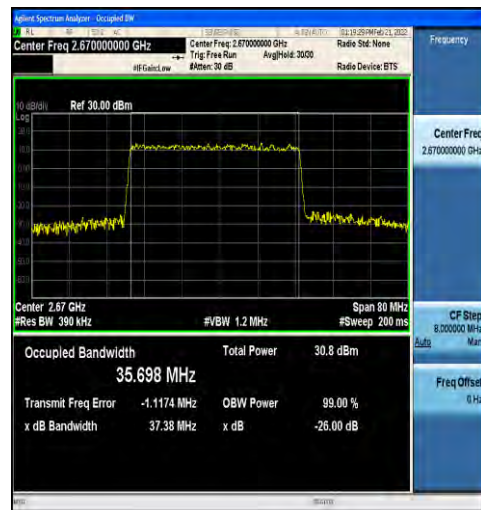
1-N41-30-40-H-3-DFT-16QAM-Outer_Full-100@0-A nt1-35.698-37.38-≤40-PASS
