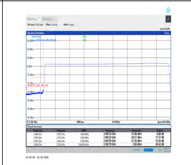
1-N41-30-60-L-6-CP-QPSK-Outer_Full-162@0-Ant1-PASS-see graph
