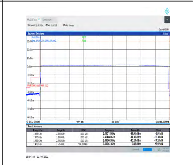
1-N41-30-80-L-6-CP-QPSK-Outer_Full-217@0-Ant1-PASS-see graph
