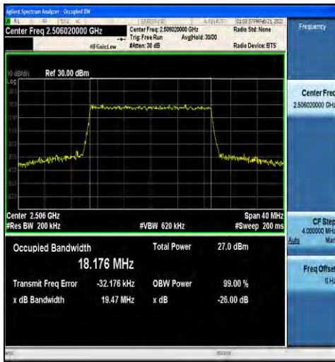
1-N41-30-20-L-9-CP-256QAM-Outer_Full-51@0-Ant 1-18.176-19.47-≤20-PASS
