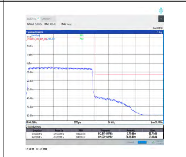
1-N5-15-10-H-6-CP-QPSK-Outer_Full-52@0-Ant1 -seegraph-PASS-see graph
