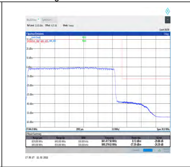
1-N5-15-20-H-3-DFT-PI2BPSK-Outer_Full-100@0-Ant1-seegraph-PASS-see graph
