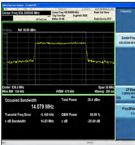
1-N5-15-15-M-8-CP-64QAM-Outer_Full-79@0-Ant1-1 14.079-14.83-≤15-PASS
