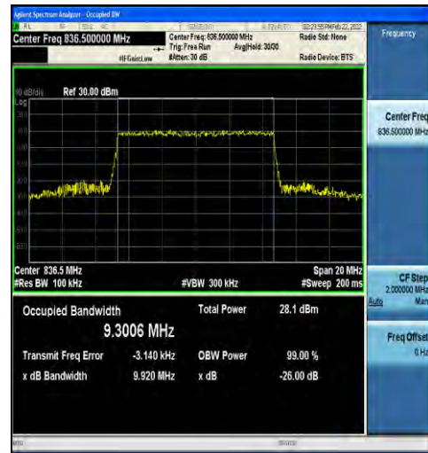
1-N5-15-10-M-8-CP-64QAM-Outer_Full-52@0-Ant1-9. 9.3006-9.920-≤10-PASS
