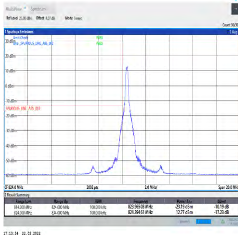
1-N5-15-10-L-4-CP-QPSK-Edge_1RB_Left-1@0-Ant1-seegraph-PASS-see graph
