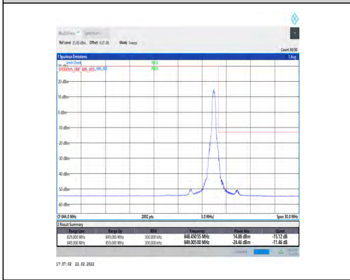
1-N5-15-20-H-5-CP-QPSK-Edge_1RB_Right-1@105-Ant1-seegraph-PASS-see graph
