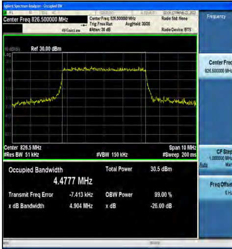
1-N5-15-5-L-1-DFT-QPSK-Outer_Full-25@0-Ant1-4. 4777-4.904-≤5-PASS
