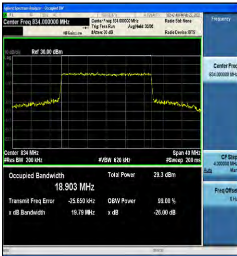
1-N5-15-20-L-6-CP-QPSK-Outer_Full-106@0-Ant1 18.903-19.79-≤20-PASS
