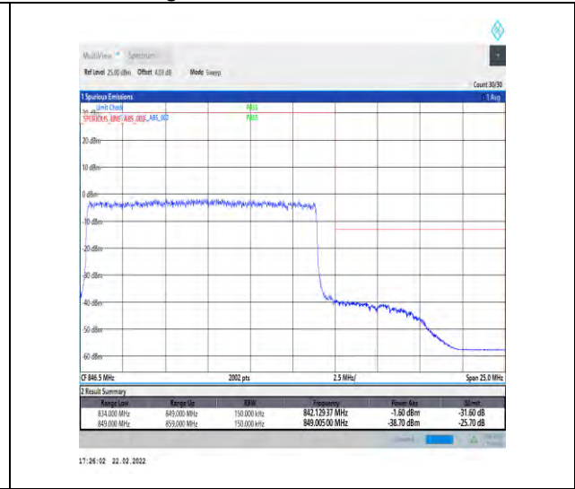
1-N5-15-15-H-3-DFT-PI2BPSK-Outer_Full-75@0- Ant1-seegraph-PASS-see graph
