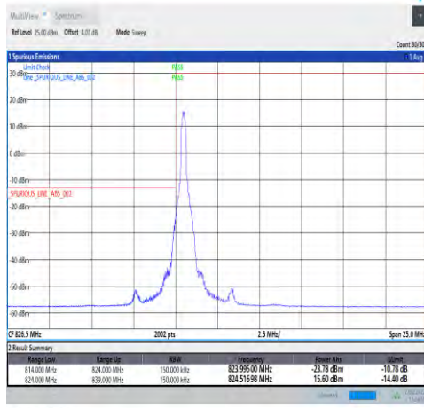
1-N5-15-15-L-1-DFT-PI2BPSK-Edge_1RB_Left-1@0-A nt1-seegraph-PASS-see graph
