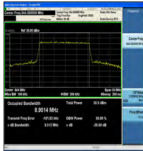
1-N5-15-10-H-1-DFT-QPSK-Outer_Full-50@0-Ant1- 8.9014-9.512-≤10-PASS
