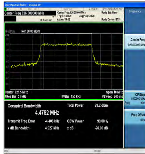
1-N5-15-5-L-4-DFT-64QAM-Outer_Full-25@0-Ant1-4 .4782-4.927-≤5-PASS
