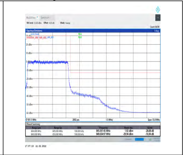
1-N5-15-5-H-3-DFT-PI2BPSK-Outer_Full-25@0-Ant1-seegraph-PASS-see graph
