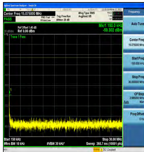
1-N5-15-20-H-1-DFT-PI2BPSK-Inner_1RB_Left-1@ -0.15-30-Ant1--59.30--23-PASS
