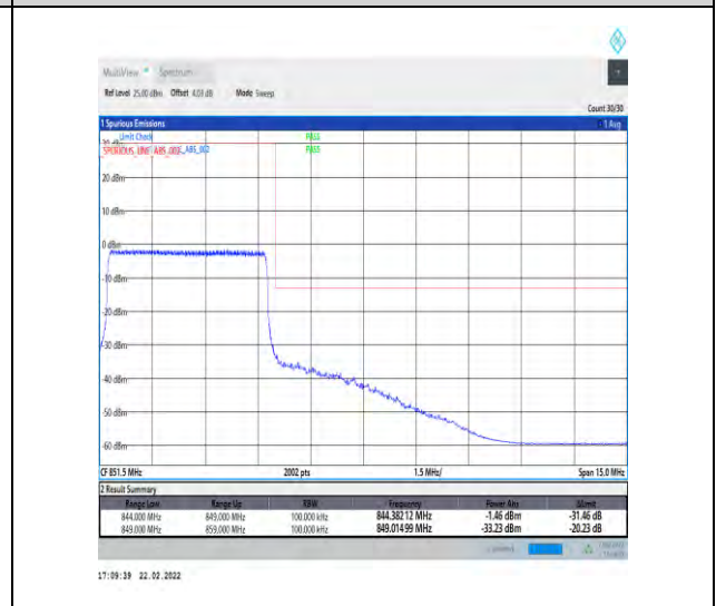
1-N5-15-5-H-6-CP-QPSK-Outer_Full-25@0-Ant1-seegraph-PASS-see graph
