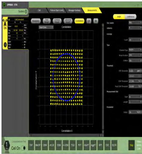
1-N5-15-20-M-5-DFT-256QAM-Outer_Full-100@0-Ant1-see graph-PASS
