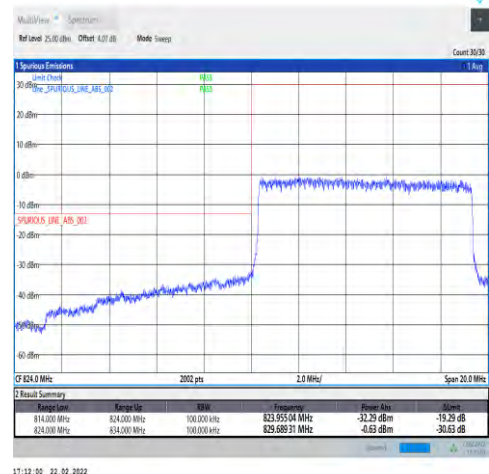
1-N5-15-10-L-3-DFT-PI2BPSK-Outer_Full-50@0-Ant1-seegraph-PASS-see graph
