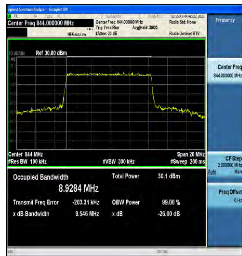
1-N5-15-10-H-3-DFT-16QAM-Outer_Full-50@0-Ant1 -8.9284-9.546-≤10-PASS
