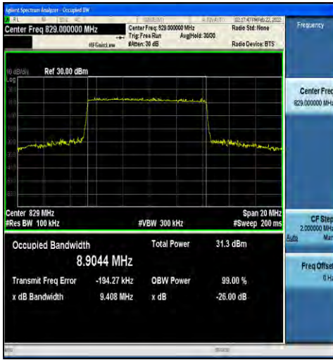
1-N5-15-10-L-2-DFT-PI2BPSK-Outer_Full-50@0-Ant 1-8.9044-9.408-≤10-PASS
