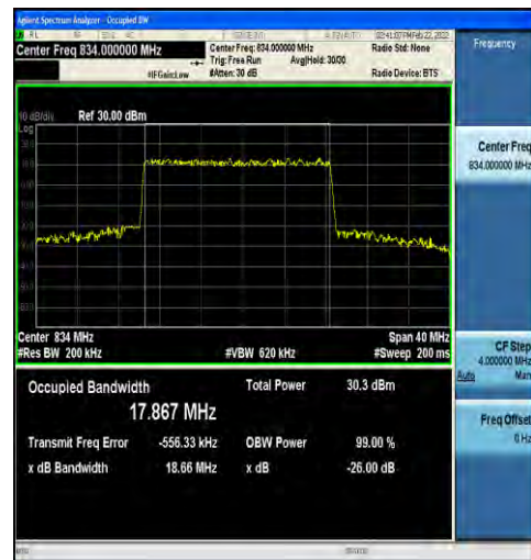
1-N5-15-20-L-3-DFT-16QAM-Outer_Full-100@0-Ant 1-17.867-18.66-≤20-PASS
