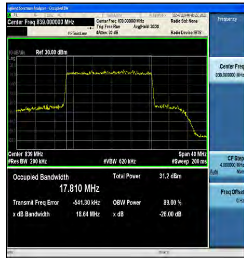
1-N5-15-20-H-1-DFT-QPSK-Outer_Full-100@0-Ant1 -17.810-18.64-≤20-PASS
