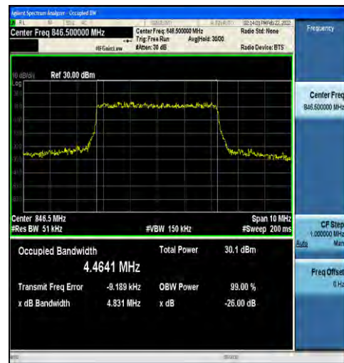
1-N5-15-5-H-2-DFT-PI2BPSK-Outer_Full-25@0-Ant1 -4.4641-4.831-≤5-PASS
