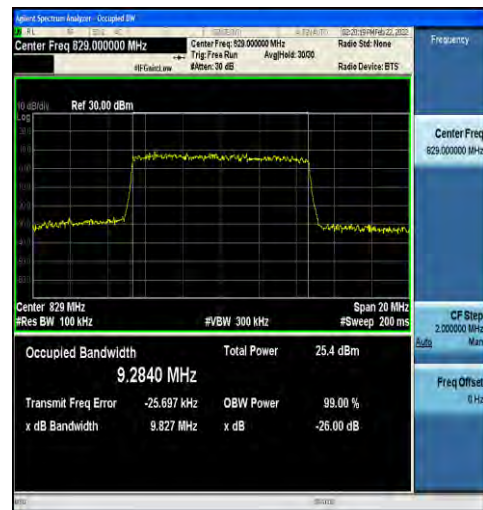
1-N5-15-10-L-9-CP-256QAM-Outer_Full-52@0-Ant1-9 9.2840-9.827-≤10-PASS
