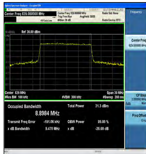
1-N5-15-10-L-1-DFT-QPSK-Outer_Full-50@0-Ant1-8 .8984-9.470-≤10-PASS
