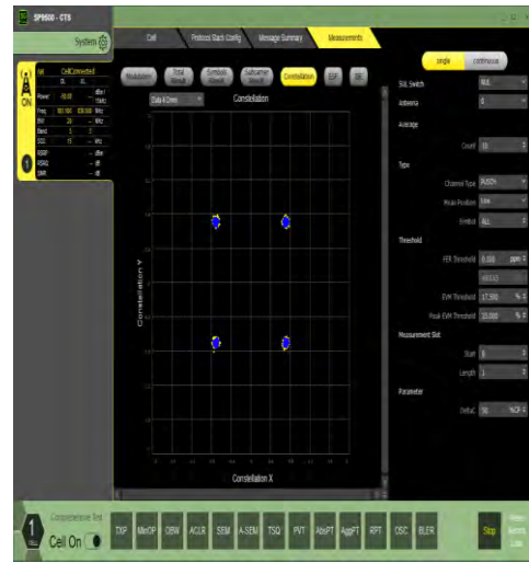
1-N5-15-20-M-6-CP-QPSK-Outer_Full-106@0-Ant1-see graph-PASS
