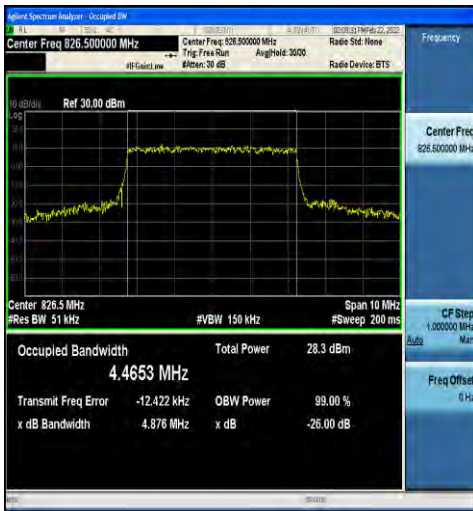
1-N5-15-5-L-7-CP-16QAM-Outer_Full-25@0-Ant1-4. 4653-4.876-≤5-PASS
