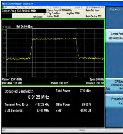
1-N5-15-10-M-5-DFT-256QAM-Outer_Full-50@0-Ant 1-8.9125-9.467-≤10-PASS
