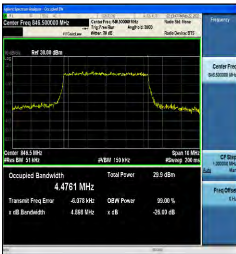
1-N5-15-5-H-1-DFT-QPSK-Outer_Full-25@0-Ant1-4. 4761-4.898-≤5-PASS
