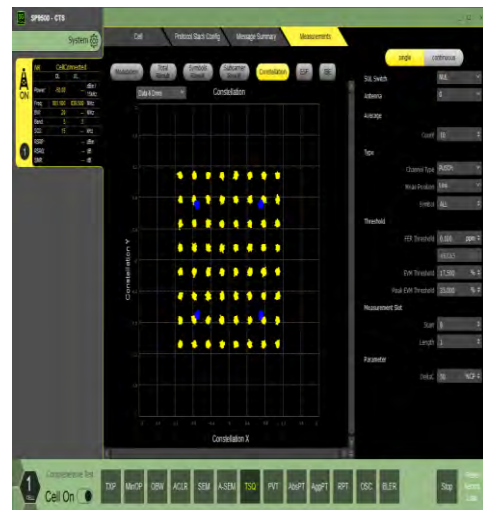
1-N5-15-20-M-8-CP-64QAM-Outer_Full-106@0-Ant1-see graph-PASS
