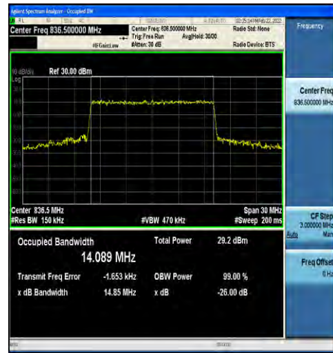
1-N5-15-15-M-7-CP-16QAM-Outer_Full-79@0-Ant1-1 14.089-14.85-≤15-PASS
