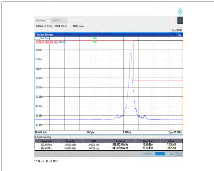
1-N5-15-20-H-2-DFT-PI2BPSK-Edge_1RB_Right-1@105-Ant1-seegraph-PASS-see graph
