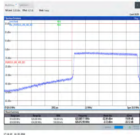
1-N5-15-10-L-6-CP-QPSK-Outer_Full-52@0-Ant1-seegraph-PASS-see graph
