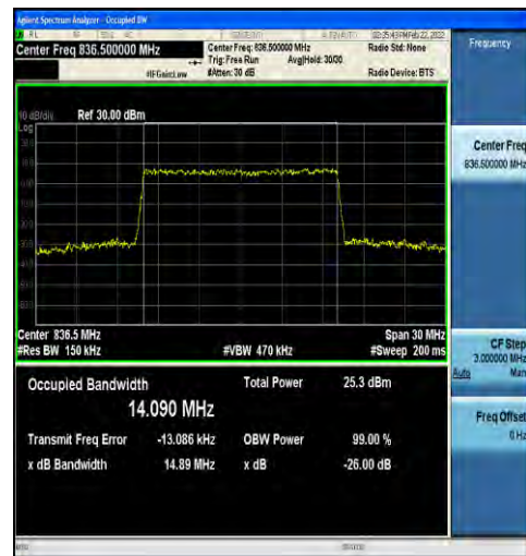
1-N5-15-15-M-9-CP-256QAM-Outer_Full-79@0-Ant1-1 -14.090-14.89-≤15-PASS
