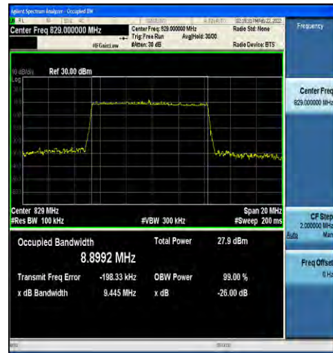
1-N5-15-10-L-5-DFT-256QAM-Outer_Full-50@0-Ant 1-8.8992-9.445-≤10-PASS
