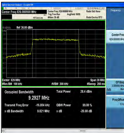
1-N5-15-10-L-8-CP-64QAM-Outer_Full-52@0-Ant1-9. 9.2927-9.821-≤10-PASS
