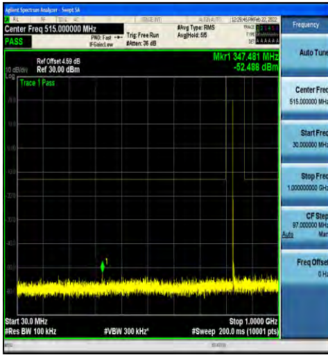
1-N5-15-20-H-1-DFT-PI2BPSK-Inner_1RB_Left-1@ 1-30-1000-Ant1--52.49--13-PASS
