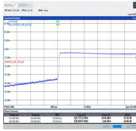
1-N5-15-15-L-6-CP-QPSK-Outer_Full-79@0-Ant1-seegraph-PASS-see graph
