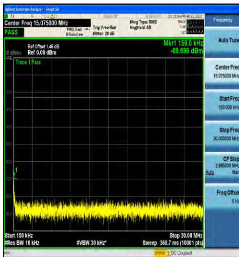
1-N5-15-20-M-1-DFT-PI2BPSK-Inner_1RB_Left-1@ 1-0.15-30-Ant1--69.70--23-PASS
