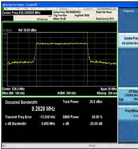
1-N5-15-10-M-7-CP-16QAM-Outer_Full-52@0-Ant1-9. 9.2828-9.868-≤10-PASS
