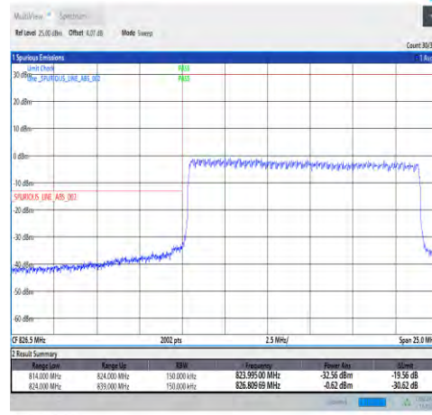
1-N5-15-15-L-3-DFT-PI2BPSK-Outer_Full-75@0-Ant1-seegraph-PASS-see graph
