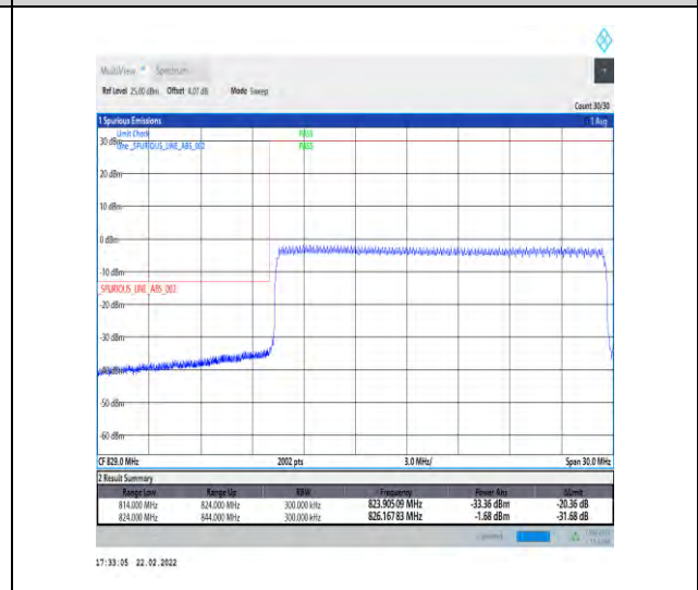
1-N5-15-20-L-6-CP-QPSK-Outer_Full-106@0-Ant1-seegraph-PASS-see graph
