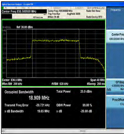
1-N5-15-20-M-9-CP-256QAM-Outer_Full-106@0-An t1-18.909-19.65-≤20-PASS
