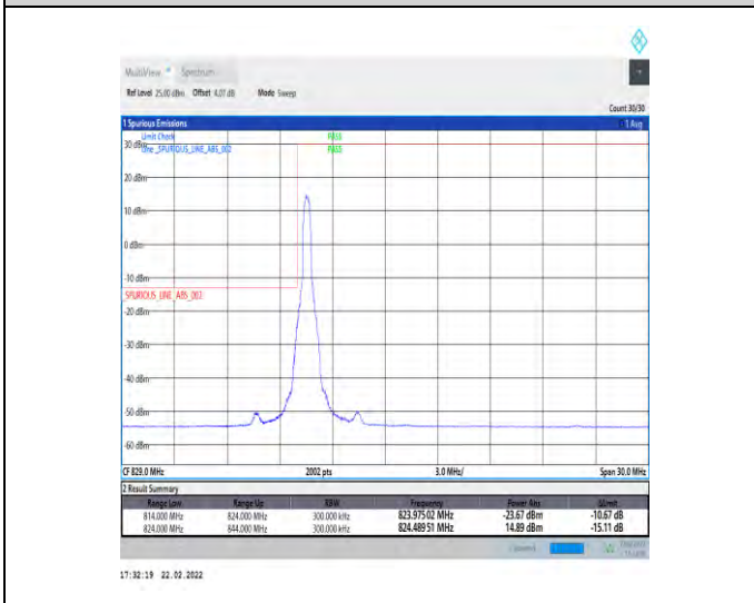
1-N5-15-20-L-4-CP-QPSK-Edge_1RB_Left-1@0-Ant1-seegraph-PASS-see graph
