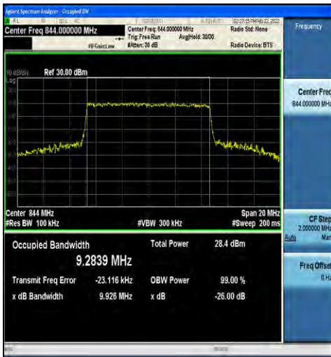
1-N5-15-10-H-6-CP-QPSK-Outer_Full-52@0-Ant1-9. 2839-9.926-≤10-PASS
