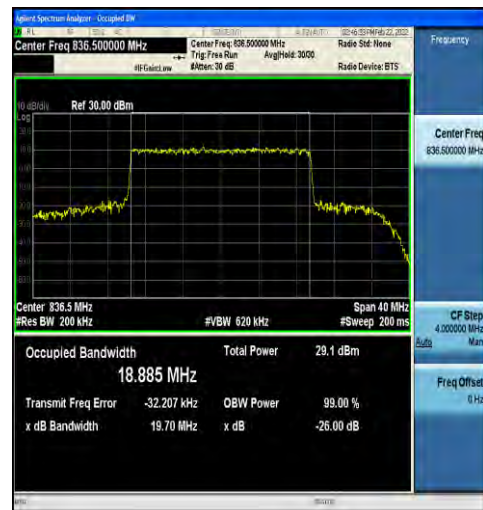
1-N5-15-20-M-6-CP-QPSK-Outer_Full-106@0-Ant1 18.885-19.70-≤20-PASS
