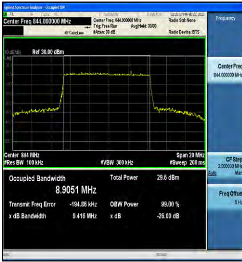
1-N5-15-10-H-4-DFT-64QAM-Outer_Full-50@0-Ant1 -8.9051-9.416-≤10-PASS
