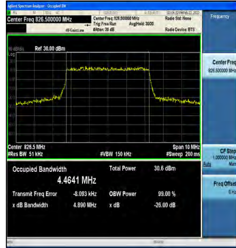
1-N5-15-5-L-2-DFT-P12BPSK-Outer_Full-25@0-Ant1 -4.4641-4.890-≤5-PASS
