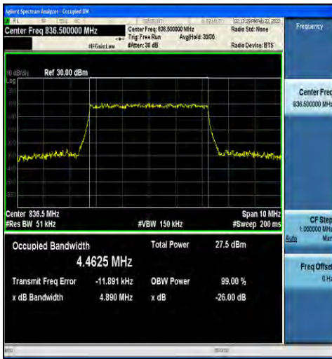
1-N5-15-5-M-8-CP-64QAM-Outer_Full-25@0-Ant1-4 4.4625-4.890-≤5-PASS
