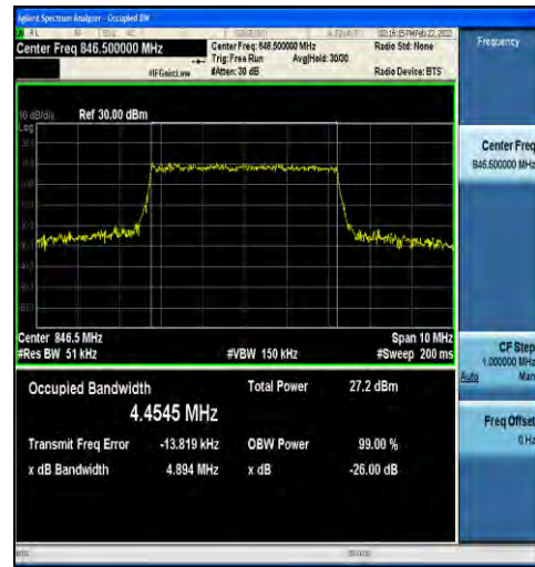
1-N5-15-5-H-8-CP-64QAM-Outer_Full-25@0-Ant1-4. 4545-4.894-≤5-PASS
