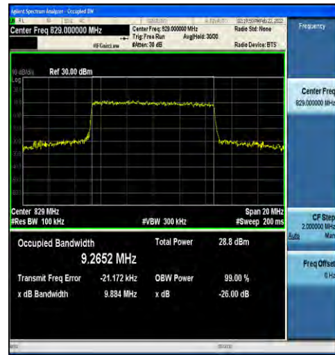
1-N5-15-10-L-7-CP-16QAM-Outer_Full-52@0-Ant1-9 .2652-9.884-≤10-PASS
