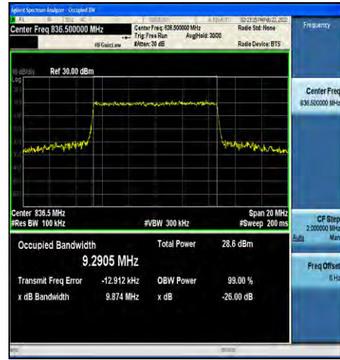
1-N5-15-10-M-6-CP-QPSK-Outer_Full-52@0-Ant1-9. 2905-9.874-≤10-PASS
