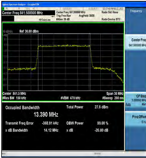
1-N5-15-15-H-5-DFT-256QAM-Outer_Full-75@0-Ant 1-13.390-14.12-≤15-PASS
