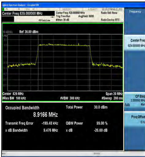
1-N5-15-10-L-4-DFT-64QAM-Outer_Full-50@0-Ant1 -8.9166-9.476-≤10-PASS
