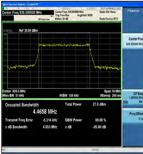
1-N5-15-5-L-5-DFT-256QAM-Outer_Full-25@0-Ant1 -4.4658-4.853-≤5-PASS
