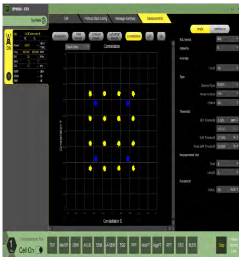
1-N5-15-20-M-7-CP-16QAM-Outer_Full-106@0-Ant1-see graph-PASS
