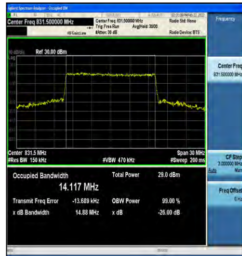
1-N5-15-15-L-6-CP-QPSK-Outer_Full-79@0-Ant1-14 .117-14.88≤15-PASS
