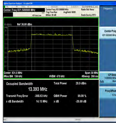
1-N5-15-15-L-4-DFT-64QAM-Outer_Full-75@0-Ant1- 13.393-14.13≤15-PASS
