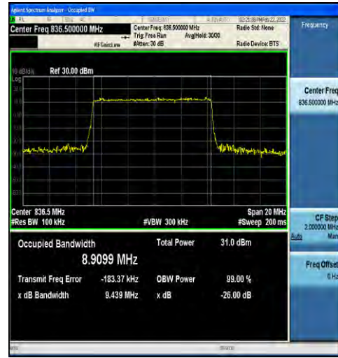
1-N5-15-10-M-2-DFT-PI2BPSK-Outer_Full-50@0-An t1-8.9099-9.439-≤10-PASS
