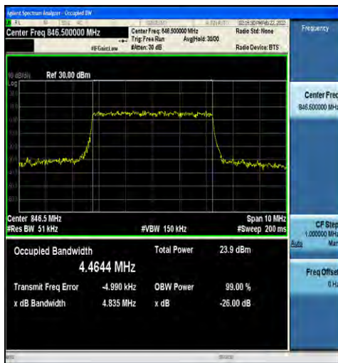
1-N5-15-5-H-9-CP-256QAM-Outer_Full-25@0-Ant1- 4.4644-4.835-≤5-PASS
