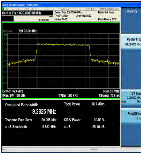
1-N5-15-10-L-6-CP-QPSK-Outer_Full-52@0-Ant1-9. 2825-9.892-≤10-PASS
