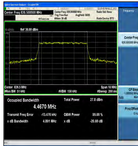
1-N5-15-5-L-8-CP-64QAM-Outer_Full-25@0-Ant1-4. 4670-4.891-≤5-PASS
