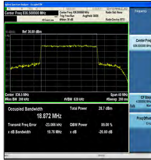
1-N5-15-20-M-8-CP-64QAM-Outer_Full-106@0-Ant1 -18.872-19.76-≤20-PASS
