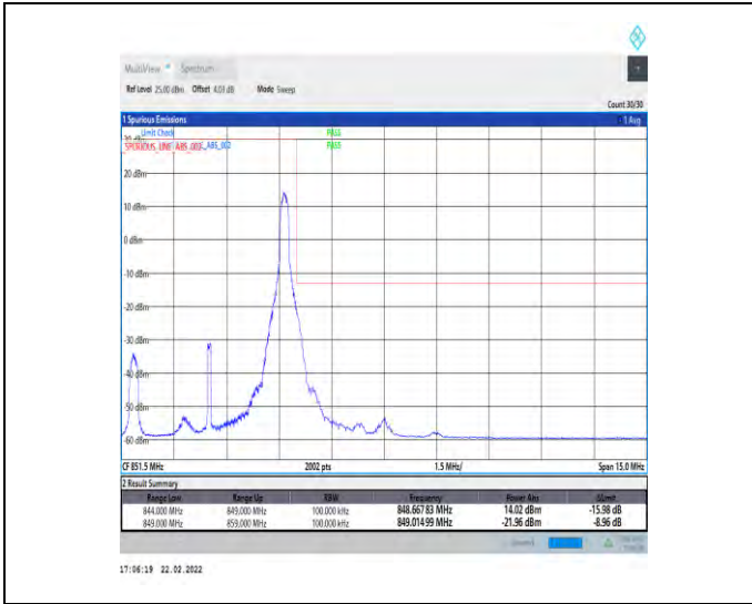
1-N5-15-5-H-2-DFT-PI2BPSK-Edge_1RB_Right-1@24-Ant1-seegraph-PASS-see graph
