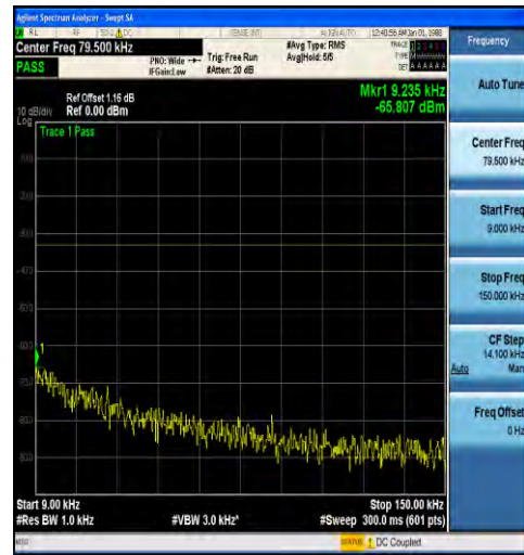
1-N5-15-20-M-1-DFT-PI2BPSK-Inner_1RB_Left-1@ 1-0.009-0.15-Ant1--65.81--33-PASS
