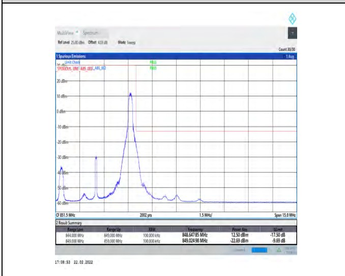
1-N5-15-5-H-5-CP-QPSK-Edge_1RB_Right-1@24-Ant1-seegraph-PASS-see graph
