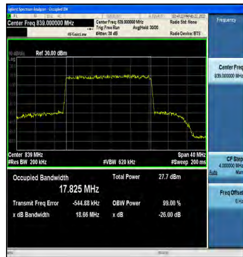
1-N5-15-20-H-5-DFT-256QAM-Outer_Full-100@0-A nt1-17.825-18.66-≤20-PASS
