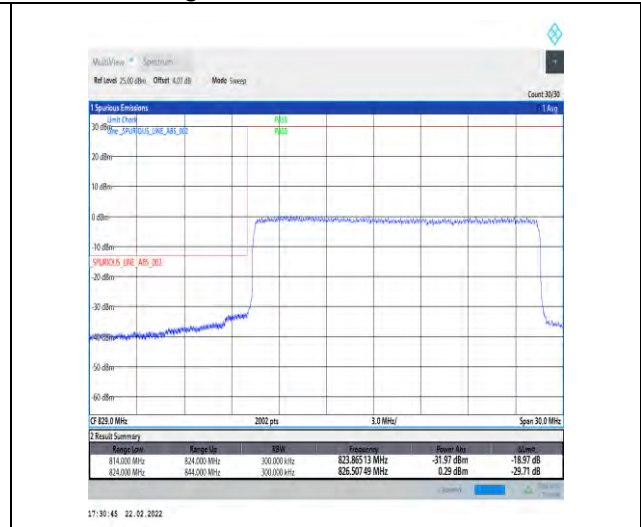
1-N5-15-20-L-3-DFT-PI2BPSK-Outer_Full-100@0-Ant1-seegraph-PASS-see graph
