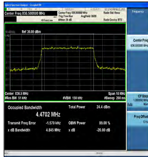
1-N5-15-5-M-9-CP-256QAM-Outer_Full-25@0-Ant1-4 4.4702-4.845-≤5-PASS
