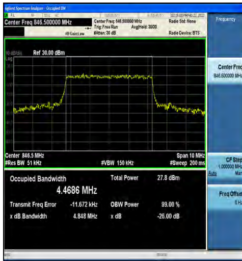
1-N5-15-5-H-7-CP-16QAM-Outer_Full-25@0-Ant1-4. 4686-4.848-≤5-PASS
