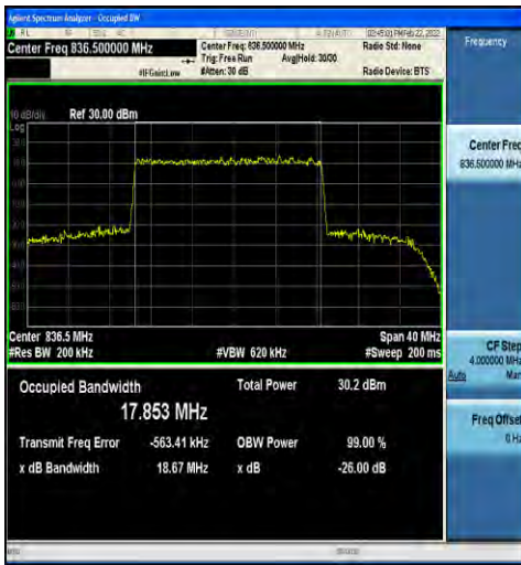
1-N5-15-20-M-3-DFT-16QAM-Outer_Full-100@0-Ant 1-17.853-18.67-≤20-PASS
