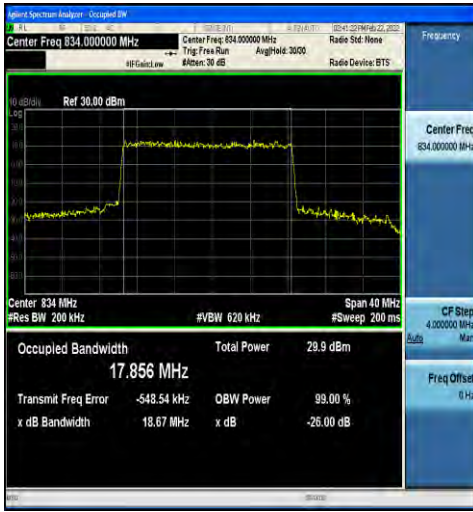
1-N5-15-20-L-4-DFT-64QAM-Outer_Full-100@0-Ant 1-17.856-18.67-≤20-PASS
