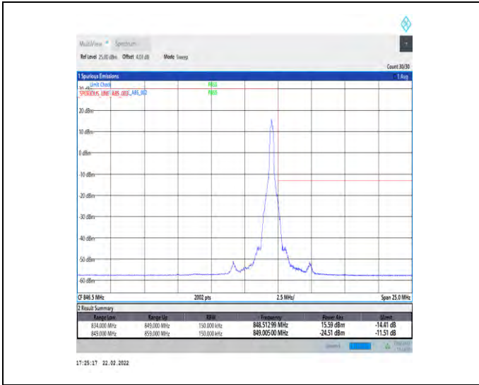
1-N5-15-15-H-2-DFT-PI2BPSK-Edge_1RB_Right-1@7 8-Ant1-seegraph-PASS-see graph
