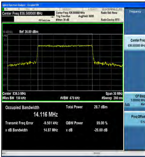
1-N5-15-15-M-6-CP-QPSK-Outer_Full-79@0-Ant1-1 4.116-14.87-≤15-PASS
