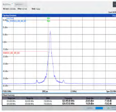
1-N5-15-15-L-4-CP-QPSK-Edge_1RB_Left-1@0-Ant1-seegraph-PASS-see graph
