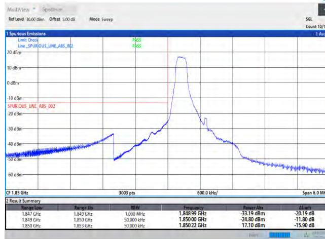
Band2-1.4MHz-QPSK-18607-6RB#0
