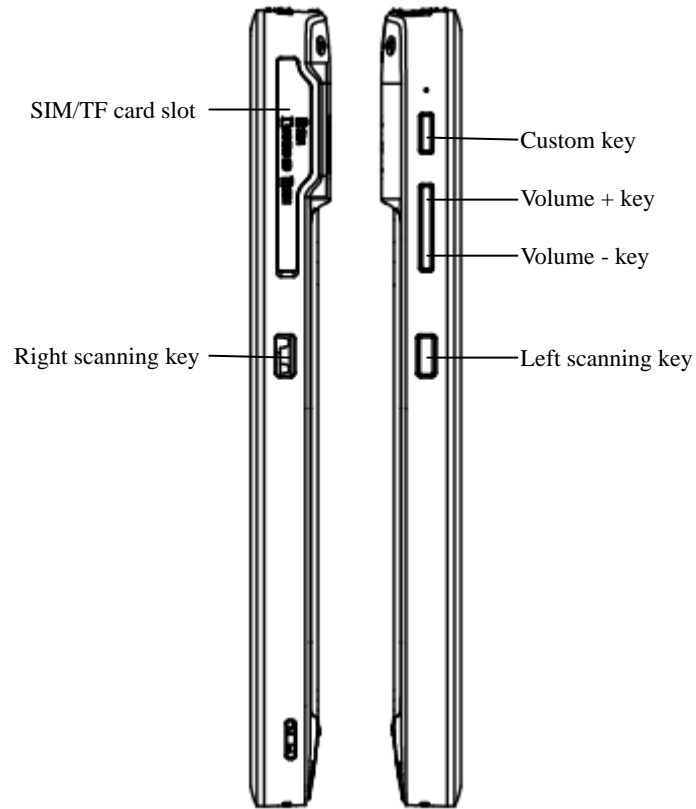
Figure 2-2 Side view
