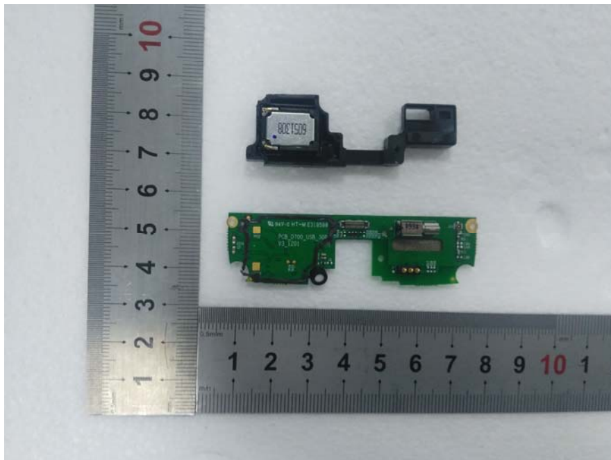
EUT –Main Board-1 Cover off View
