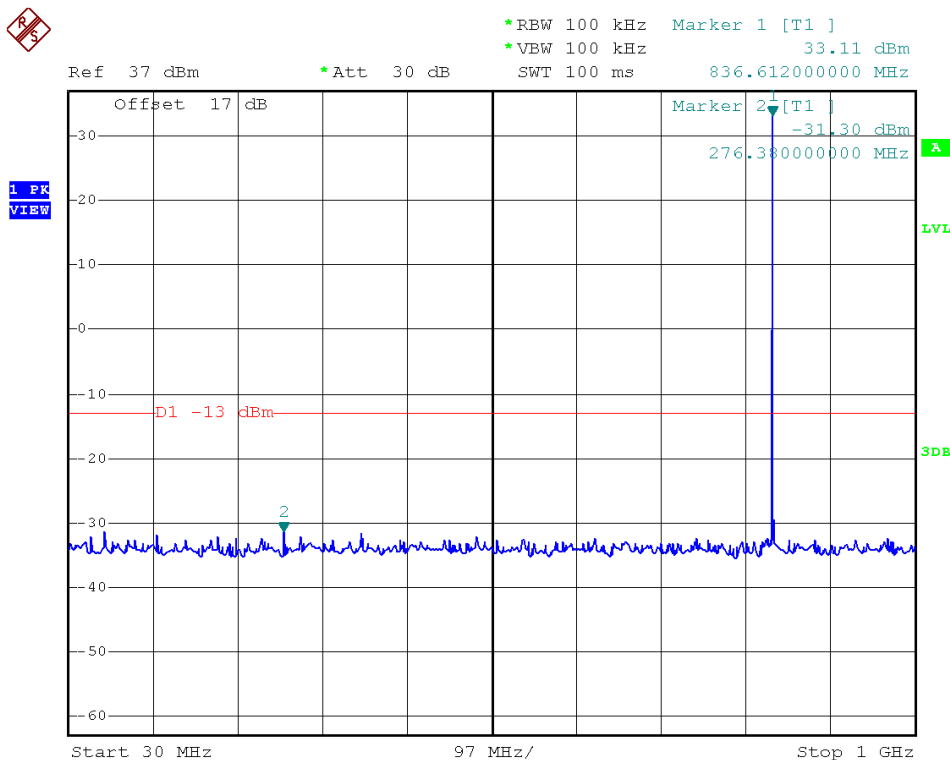
(Plot C2: EDGE 850MHz Channel = 190, 30MHz to 1GHz)
