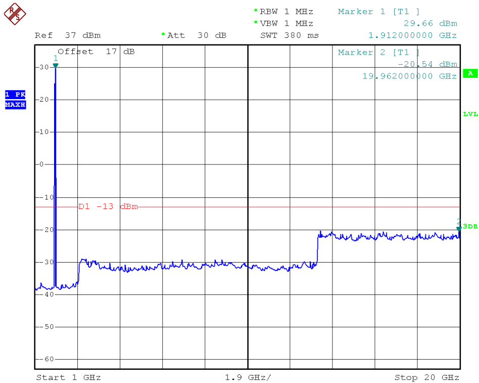
(Plot D3.1: EDGE 1900MHz Channel = 810, 1GHz to 20GHz)
