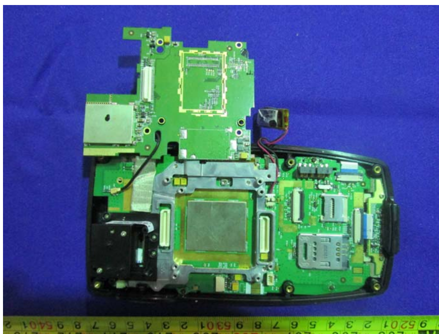
EUT –BT/Wifi Board Off View
