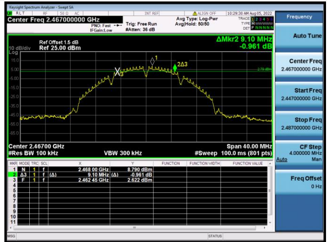
802.11b CHANNEL 12
