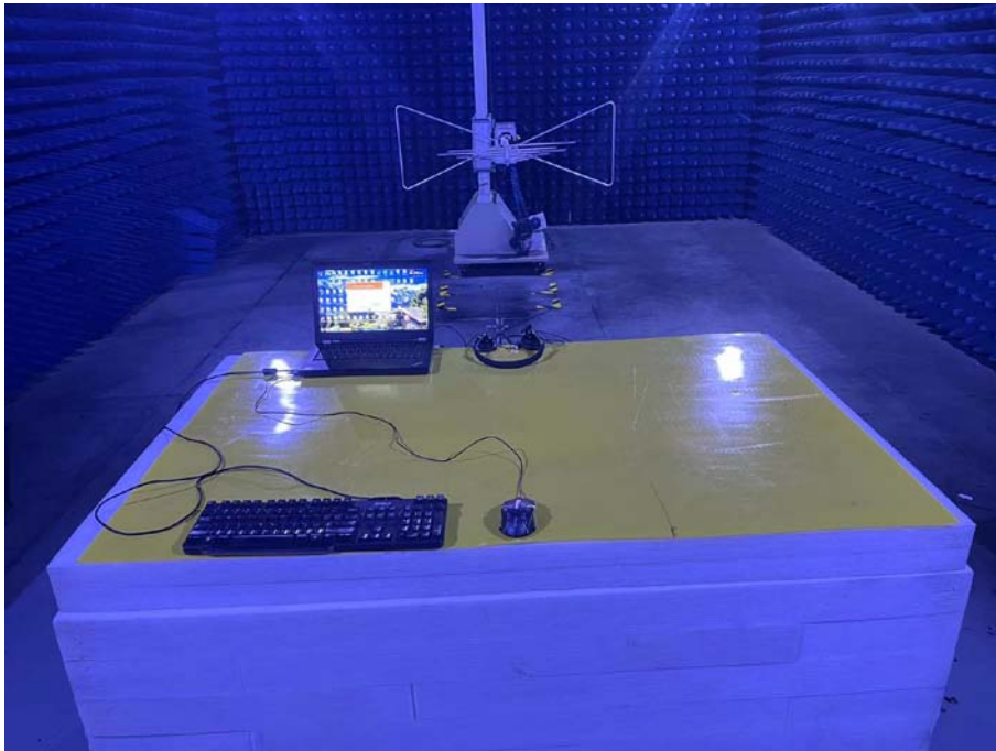
VT 8200 Duo
