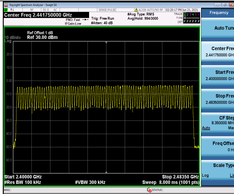
GFSK Modulation
