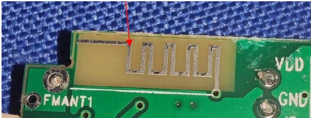
Antenna Photo
