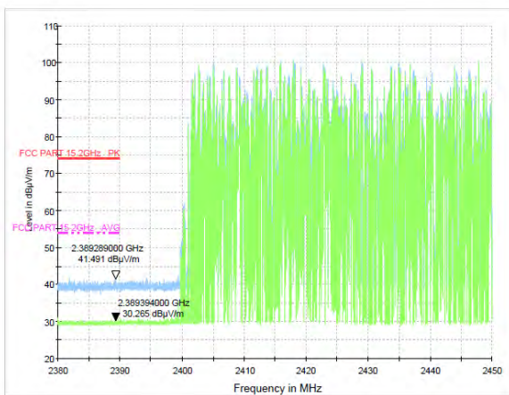
Test Mode: GFSK-Low Hopping-on Polarization: Vertical
