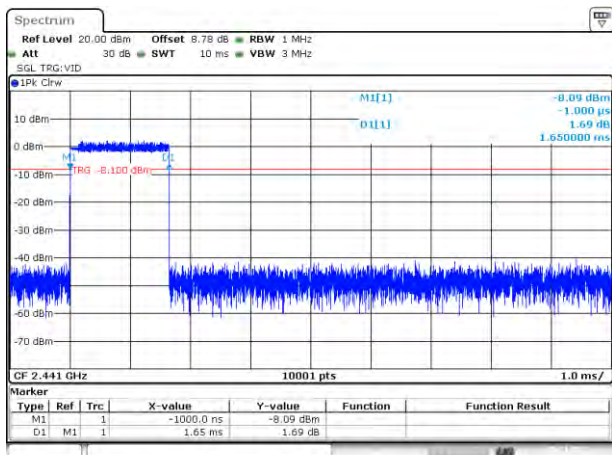
Channel 39 / 2441 MHz - 3DH1
