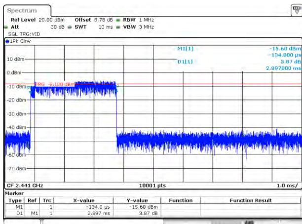
Channel 39 / 2441 MHz - 3DH3
