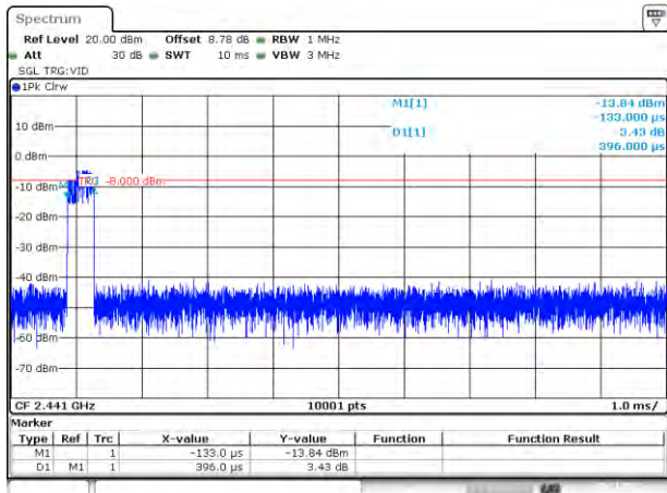
Channel 39 / 2441 MHz - 3DH1
