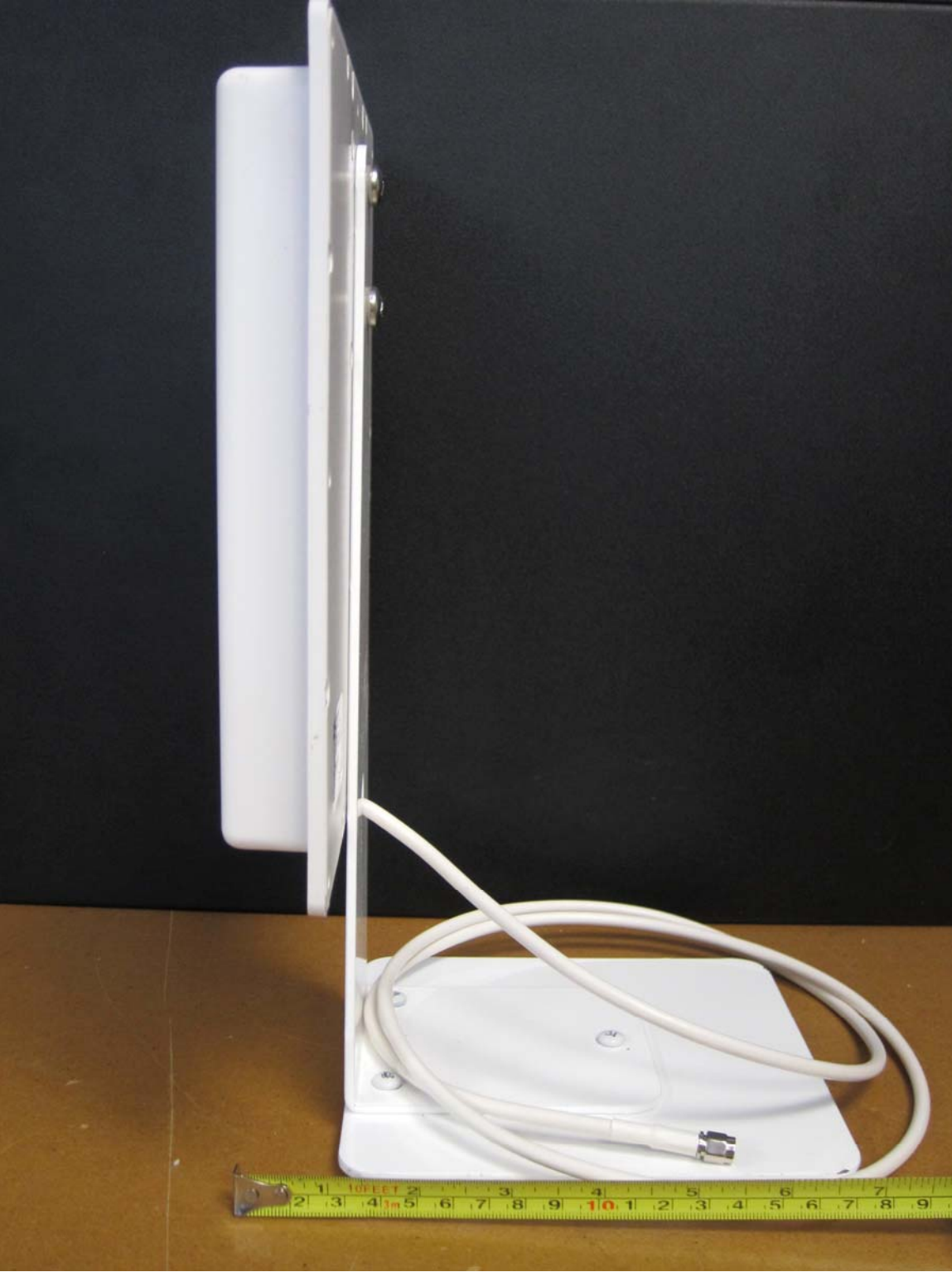
Antenna Right Side View
