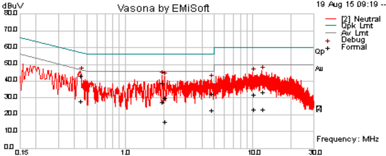
Neutral Line Plot @ 120Vac, 60Hz
