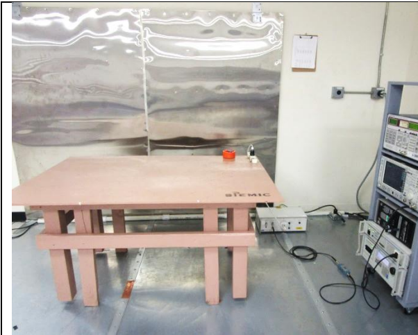
AC Line Conducted Emissions – Front View
