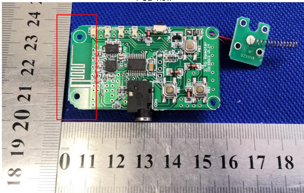
PCB view
