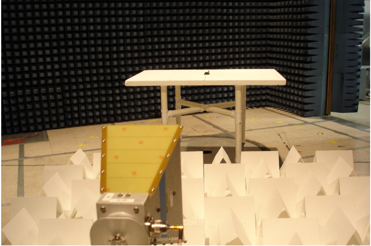
Figure 1. Photo of Radiated Emissions EUT Set-up for Frequencies > 1GHz
