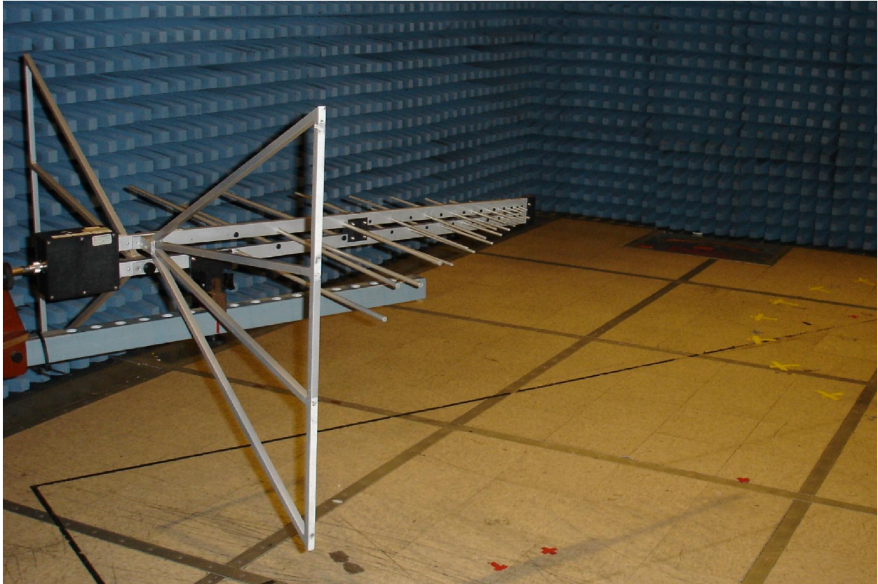
Figure 2. Radiated Emissions Antenna used in EUT Set-up for Frequencies < 1GHz (Biconilog)
