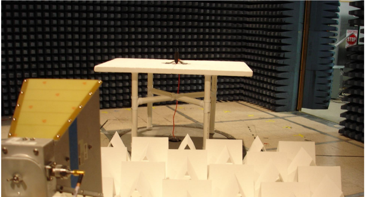
Figure 1. Radiated emissions set-up > 1GHz (Horn Antenna)
