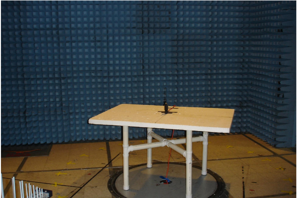
Figure 2. Radiated emissions set-up < 1GHz (Biconilog Antenna)
