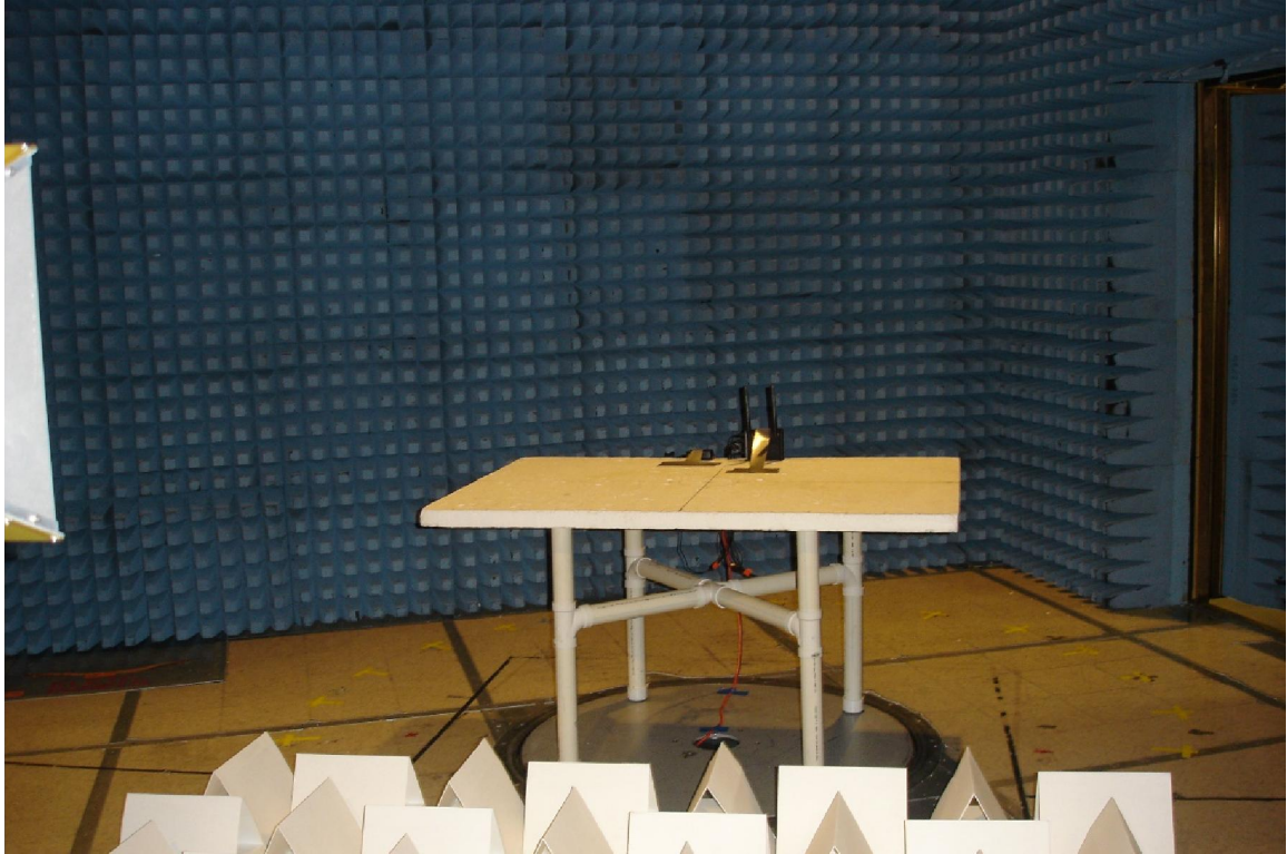
Figure 2. Photo of Radiated Emissions EUT Set-up for Frequencies >1GHz.
