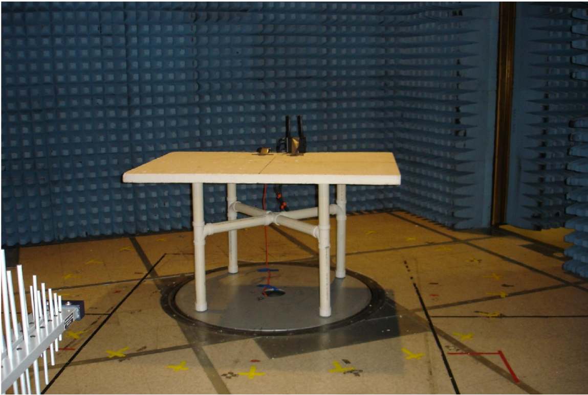
Figure 1. Photo of Radiated Emissions EUT Set-up for Frequencies 30MHz - 1GHz
